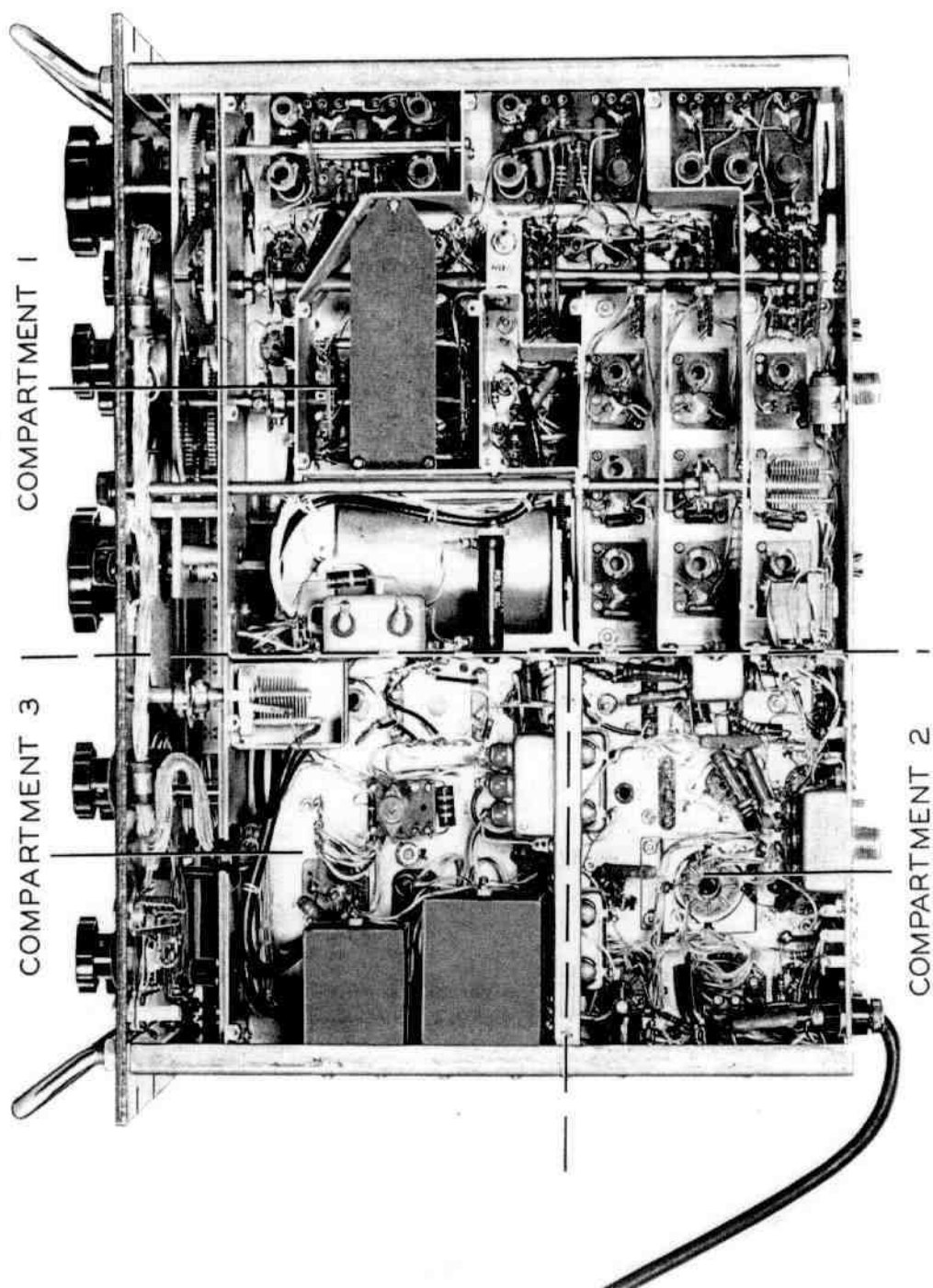
Figure 7-2. 51J-4 Bottom View
