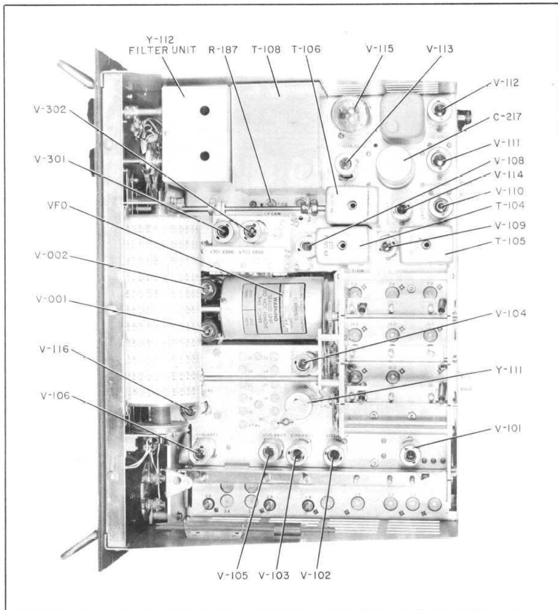
Figure 7-1. 51J-4 Top View, Tube and Parts Identification
