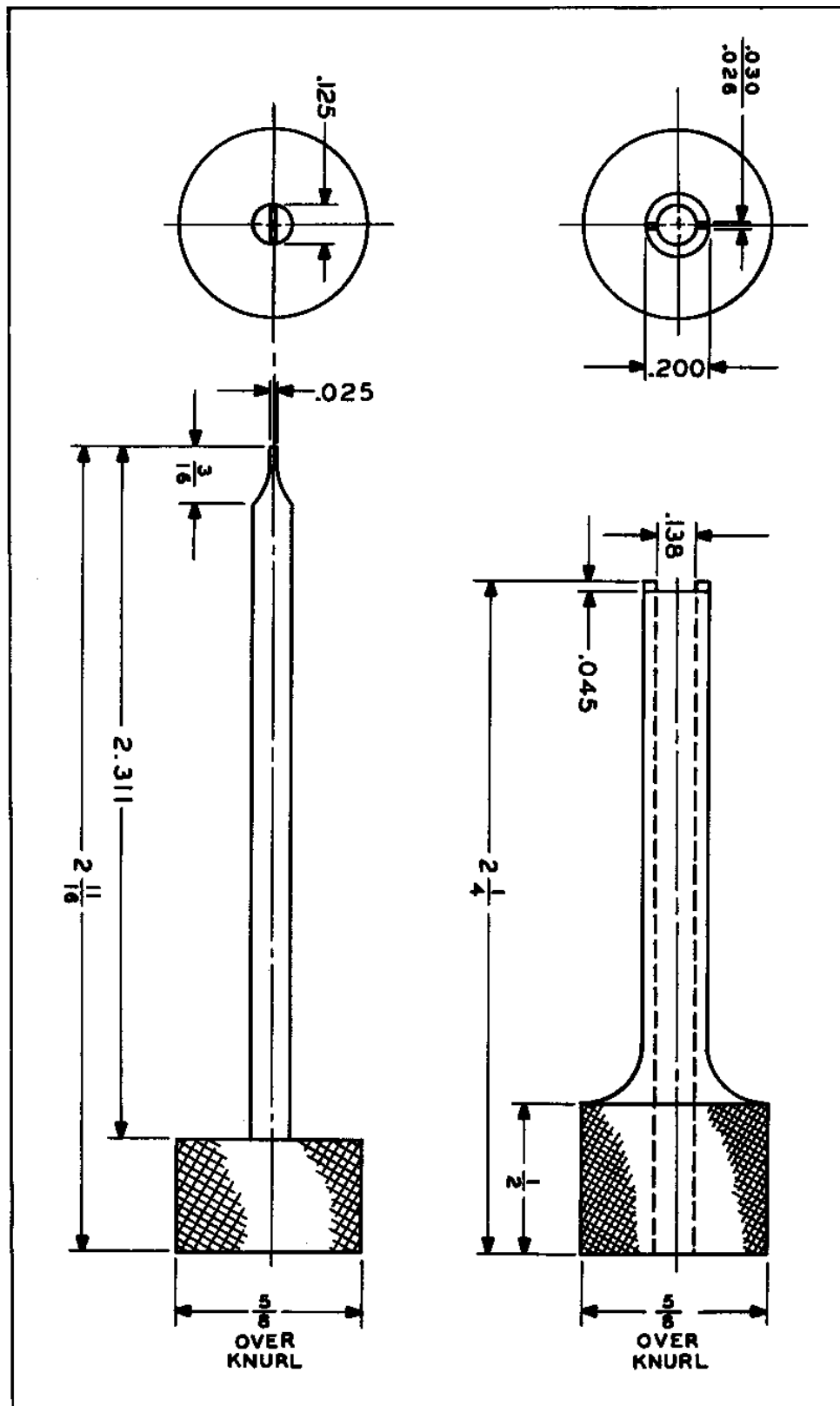
Figure 5-7. 51J-4 VFO Adjustment Tool
