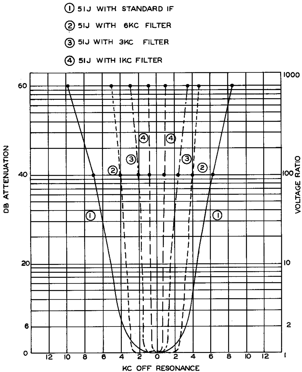
Figure 5-2. 51J-4 Selectivity Curves
