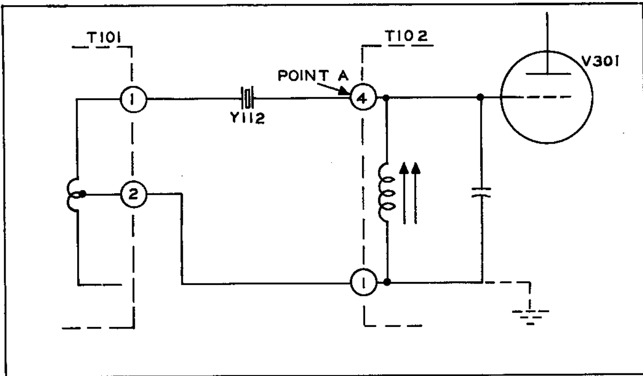
Figure 4-5. 51J-4 Crystal Filter - Simplified, Position "1"
