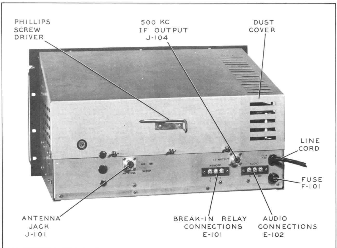
Figure 2-2. 51J-4 Rear Connections
