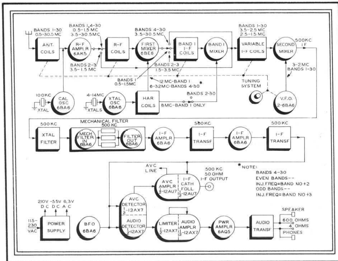
Figure 1-1. 51J-4 Receiver, Front View and Block Diagram
