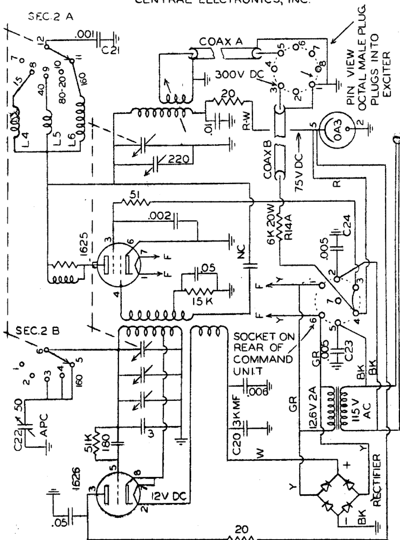
SCHEMATIC OF BC458 CONVERTED FOR 5 BAND OPERATION
