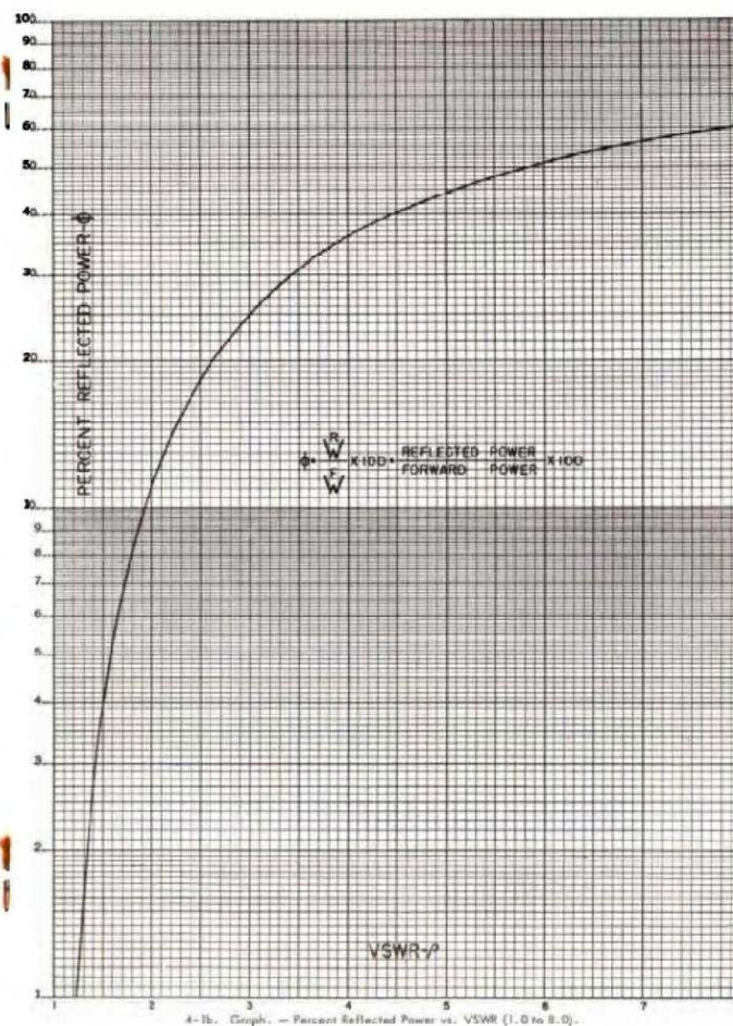
4-1b. Graph. — Percent Reflected Power vs. VSWR (1.0 to 8.0).
