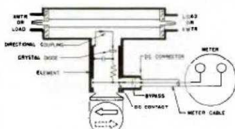
Fig. 2-1. Schematic Diagram
