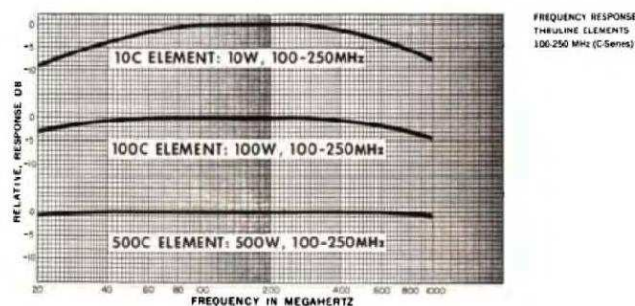
Fig. 4-2. Graph - Representative Frequency Response
