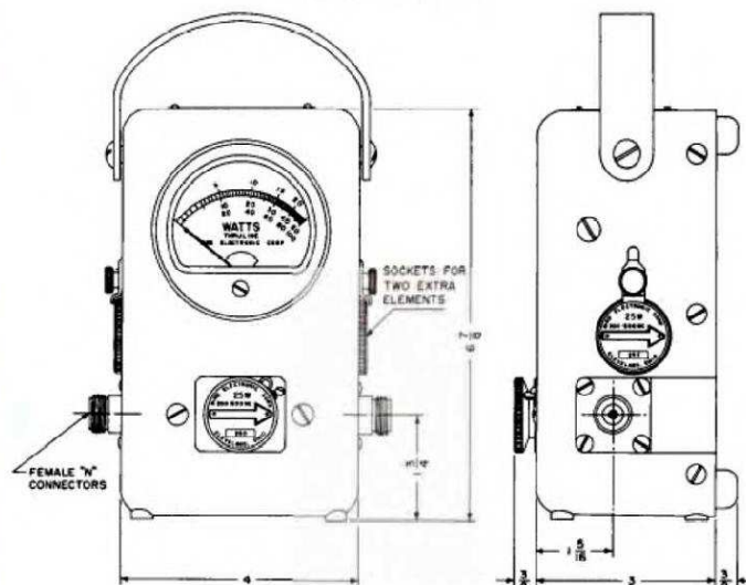
Fig. 3-1. Outline Drawing, Model 43 THRULINE
