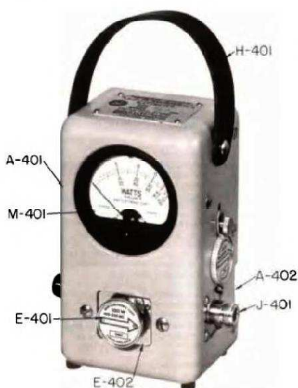
Fig. 5-1. Parts Illustration.
