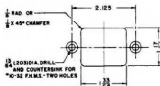
Fig. 3-3. Panel Cut for Mounting RF Body
