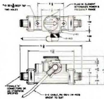
Fig. 3-2. Installation Drawing, RF Line Section
