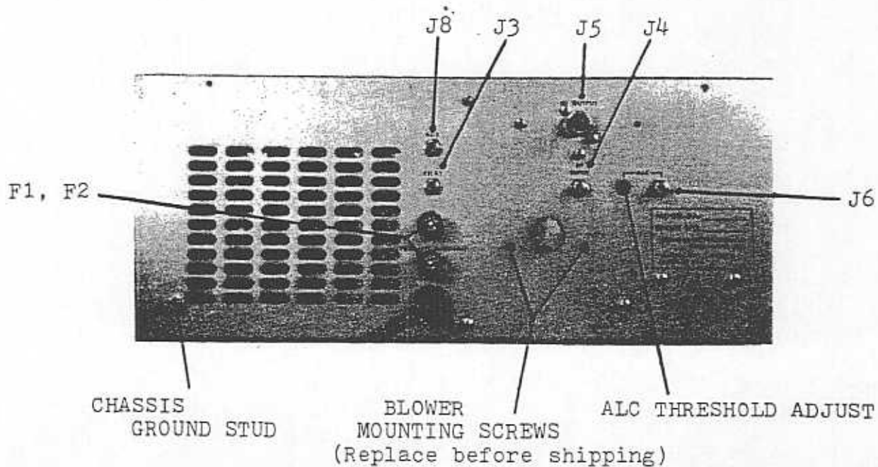
FIGURE 5. Rear View.
