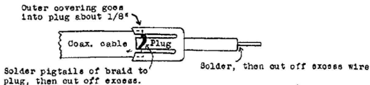
Fig. 1-B. Cable inserted in auto radio antenna plug.
