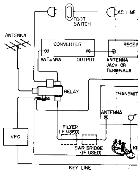
FIG.4 CONNECTIONS FOR PHONE AN
