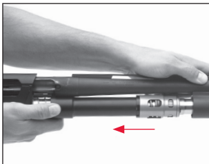
Slide the barrel and piston over the magazine tube and the barrel extension into the receiver.
