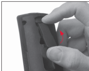
Press and hold the release button while lifting the Speed Lock lever.
