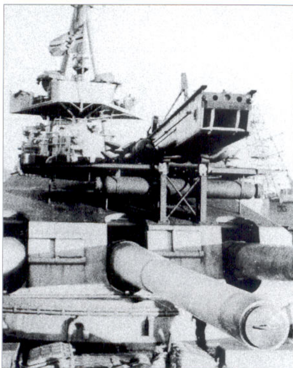
This view of turret 'Caesar' on Scharnhorst gives excellent detail of the second aircraft catapult, subsequently removed. Note the tompons that have been fitted to the ends of the gun barrels to protect the bore when not in use.
