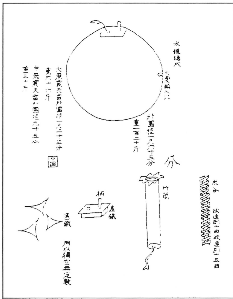
The details of the construction of the Korean version of the thunder crash bomb as shown by a drawing in Yungwon p'ilbi . This is quite a sophisticated weapon made from two cast iron hemispheres with a fuse wrapped round a cylindrical core.
