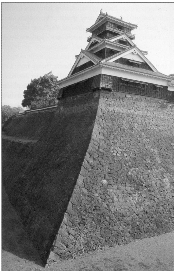
The Uto tower of Kumamoto, the castle built by Kato Kiyomasa after his experience of Chinese siege warfare. This shows the final form of Japanese defensive architecture whereby tower keeps were raised on top of the massive stone-clad mounds. The tower is provided with concealed 'machicolations' for dropping stones.
