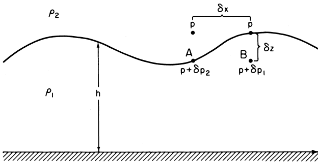
Fig. 7.7 A two-layer fluid system.
