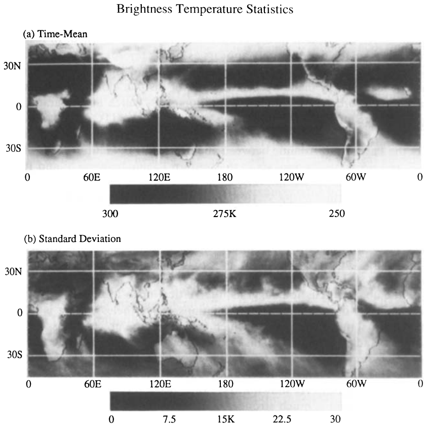
Fig. 11.2 (a) Time-mean IR brightness temperature and (b) three-hourly standard deviations about the time-mean IR brightness temperature for August 14 to December 17, 1983. Low values of brightness temperature indicate the presence of high cold cirrus anvil clouds. (After Salby et al., 1991.)
