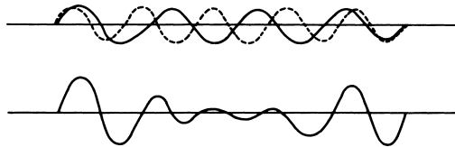
Fig. 7.3 Wave groups formed from two sinusoidal components of slightly different wavelengths. For nondispersive waves, the pattern in the lower part of the diagram propagates without change of shape. For dispersive waves, the shape of the pattern changes in time.
