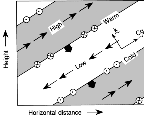
Fig. 7.12 Vertical section in a plane containing the wave vector k showing the phase relationships among velocity, geopotential, and temperature fluctuations in an upward propagating inertia–gravity wave with m < 0 , v > 0 , and f > 0 (Northern Hemisphere). Thin sloping lines denote the surfaces of constant phase (perpendicular to the wave vector), and thick arrows show the direction of phase propagation. Thin arrows show the perturbation zonal and vertical velocity fields. Meridional wind perturbations are shown by arrows pointed into the page (northward) and out of the page (southward). Note that the perturbation wind vector turns clockwise (anticyclonically) with height. (After Andrews et al., 1987.)
