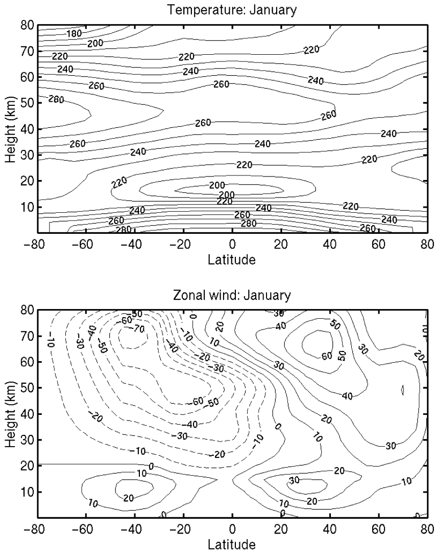
Fig. 12.2 Observed monthly and zonally averaged temperature ( \text{K} ) and zonal wind ( \text{m s}^{-1} ) for January. (Based on Fleming et al., 1990.)
