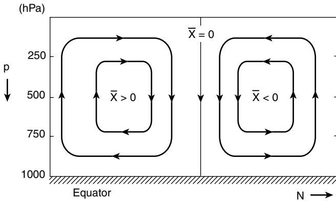
Fig. 10.1 Relationship of the Eulerian mean meridional stream function to vertical and meridional motion.
