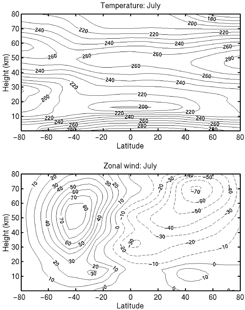
Fig. 12.3 Observed monthly and zonally averaged temperature (K) and zonal wind ( \text{m s}^{-1} ) for July. (Based on Fleming et al., 1990.)
