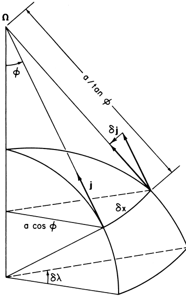
Fig. 2.3 Dependence of unit vector \mathbf{j} on longitude.
