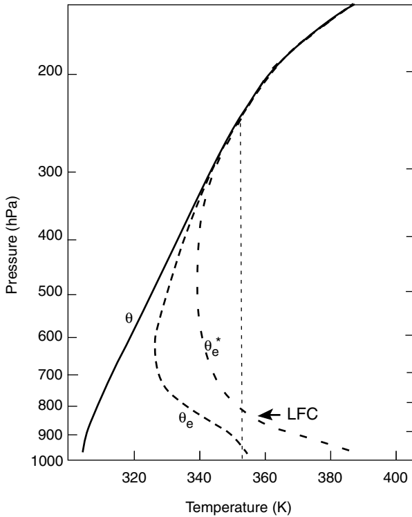
Fig. 9.10 Schematic sounding for a conditionally unstable environment characteristic of Midwestern North America thunderstorm conditions showing the vertical profiles of potential temperature, \theta , equivalent potential temperature, \theta_e , and the equivalent temperature, \theta_e^* , of a hypothetically saturated atmosphere with the same temperature profile. Dotted line shows \theta_e for a nonentraining parcel raised from the surface. Arrow denotes the LFC for the parcel.
