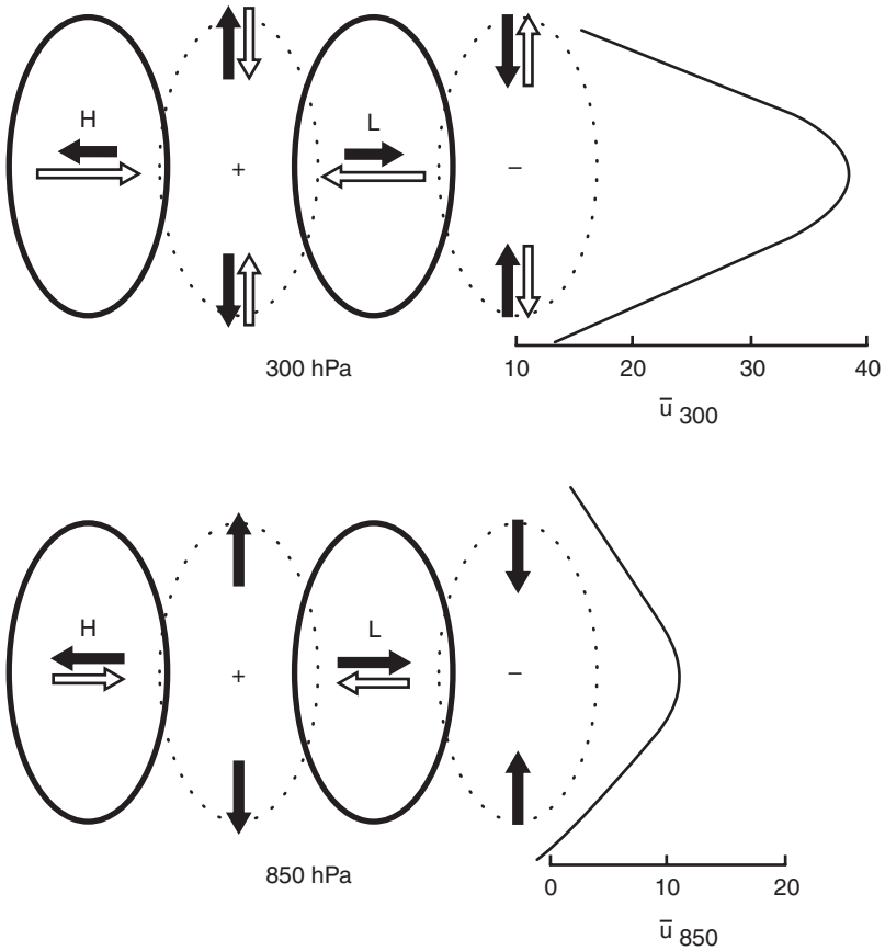
Fig. 6.15 Isallobaric and advective contributions to the ageostrophic wind for baroclinic waves in westerlies. Solid ellipses indicate perturbation geopotential patterns at 300 and 850 hPa. Dashed ellipses show a geopotential tendency pattern with positive and negative tendencies indicated by + and - signs, respectively. The mean zonal flow distribution in which the waves are embedded is indicated on the right for each level. Solid arrows show the isallobaric part of the ageostrophic wind, and open arrows show the advective part. (Adapted from Lim et al., 1991.)
