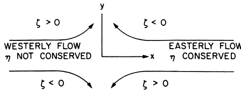
Fig. 4.8 Absolute vorticity conservation for curved flow trajectories.
