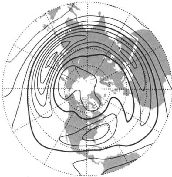
Fig. 6.2 Mean zonal wind at the 200-hPa level for December–February averaged for years 1958–1997. Contour interval 10\text{ m s}^{-1} (heavy contour, 20\text{ m s}^{-1} ). (Based on NCEP/NCAR reanalyses; after Wallace, 2003.)
