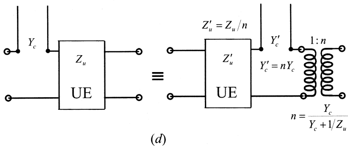
FIGURE 3.26 Kuroda identities.
