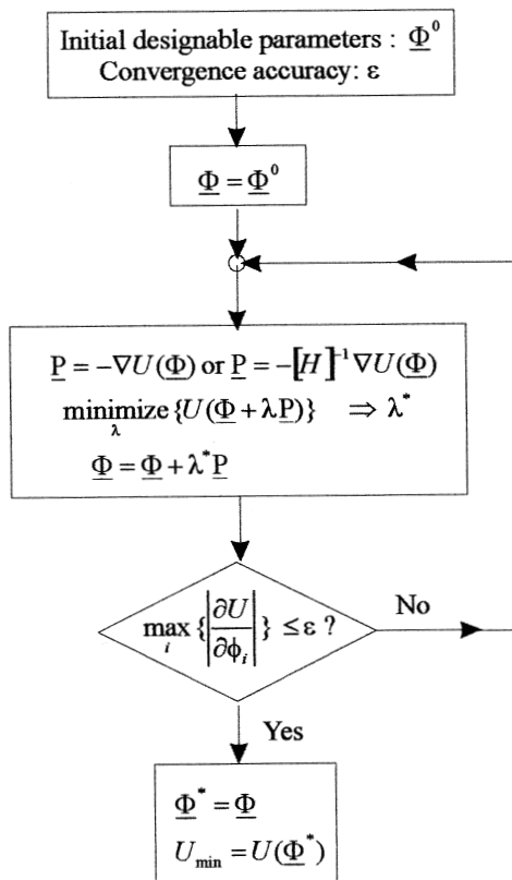
FIGURE 9.10 Algorithm of the gradient-based optimization.
