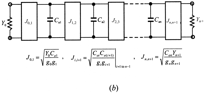
FIGURE 3.18 Lowpass prototype filters modified to include immittance inverters.
