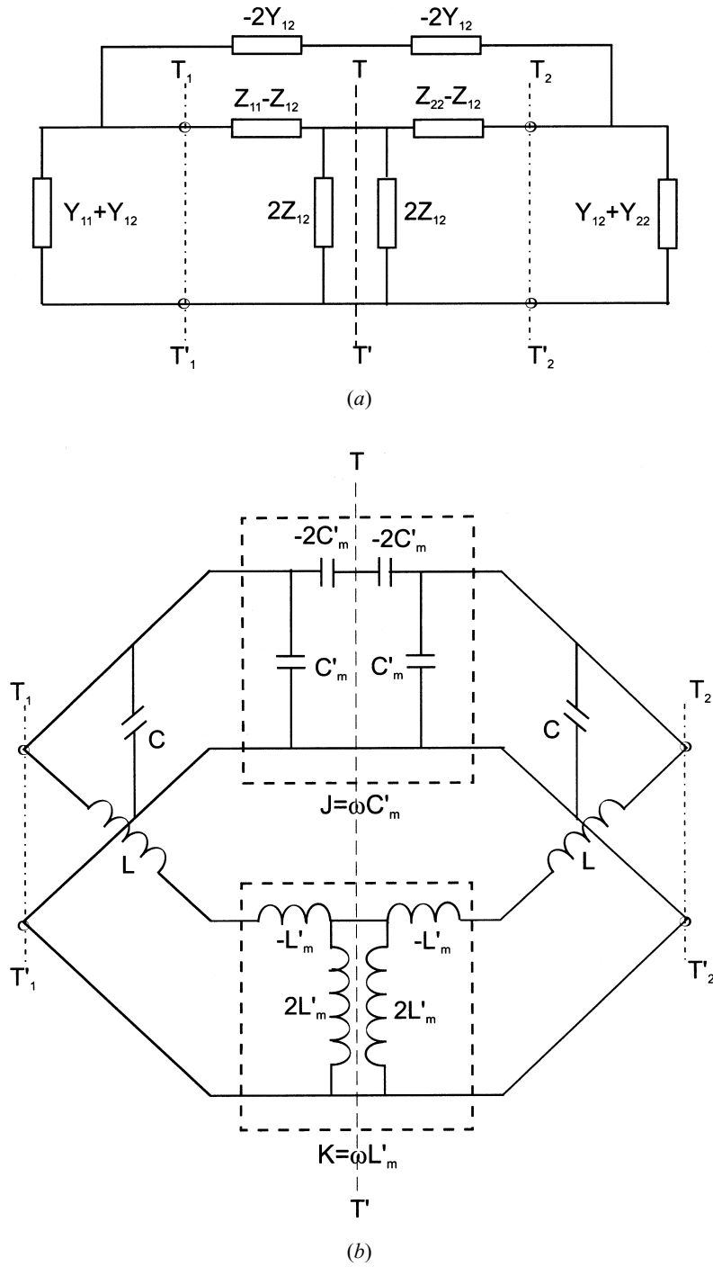
FIGURE 8.6 (a) Network representation of synchronously tuned coupled resonator circuit with mixed coupling. (b) An associated equivalent circuit with an impedance inverter K = \omega L'_m and an admittance inverter J = \omega C'_m to represent the magnetic coupling and electric coupling, respectively.
