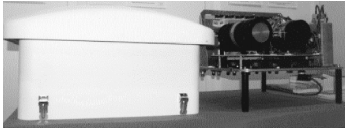
FIGURE 12.5 Tower-mounted transceiver with HTS microstrip duplexers and filters for mobile base station application.
