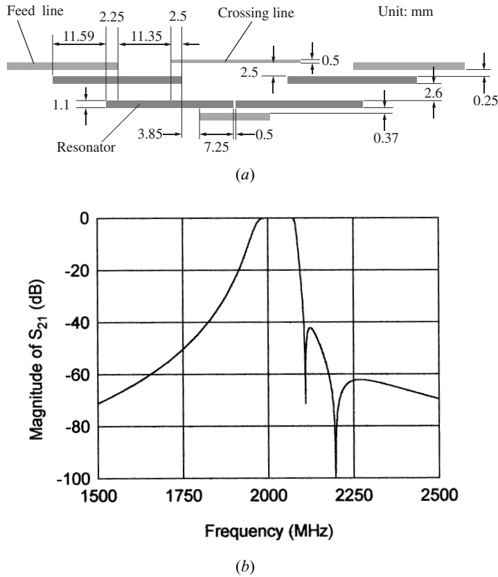
FIGURE 10.23 (a) Layout of a four-pole microstrip transmission line filter on a 1.27 mm thick substrate with a relative dielectric constant of 10.8. (b) Simulated performance of the filter.
