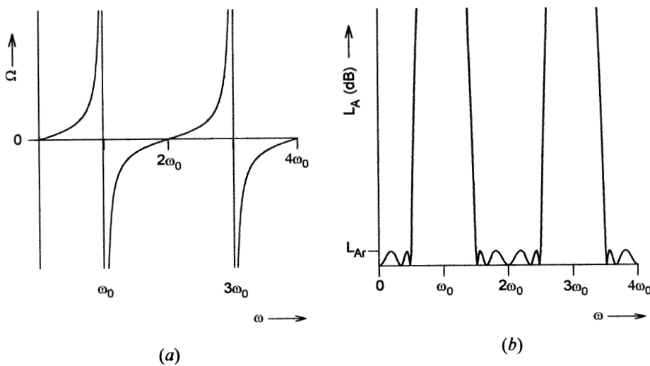
FIGURE 3.23 (a) Frequency mapping between real frequency variable \omega and distributed frequency variable \Omega . (b) Chebyshev lowpass response using the Richards' transformation.
