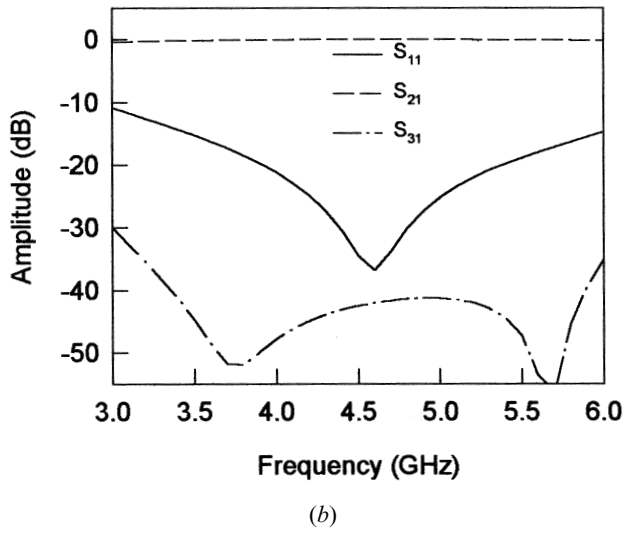
FIGURE 6.15 (a) A microstrip bias T incorporating a bandstop (pseudolowpass) filter for RF choke. (b) EM simulated performance of the microstrip bias T.
