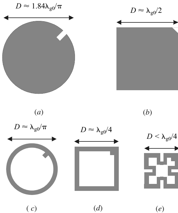
FIGURE 11.23 Some microstrip dual-mode resonators. (a) Circular disk. (b) Square patch. (c) Circular ring. (d) Square loop. (e) Meander loop.
