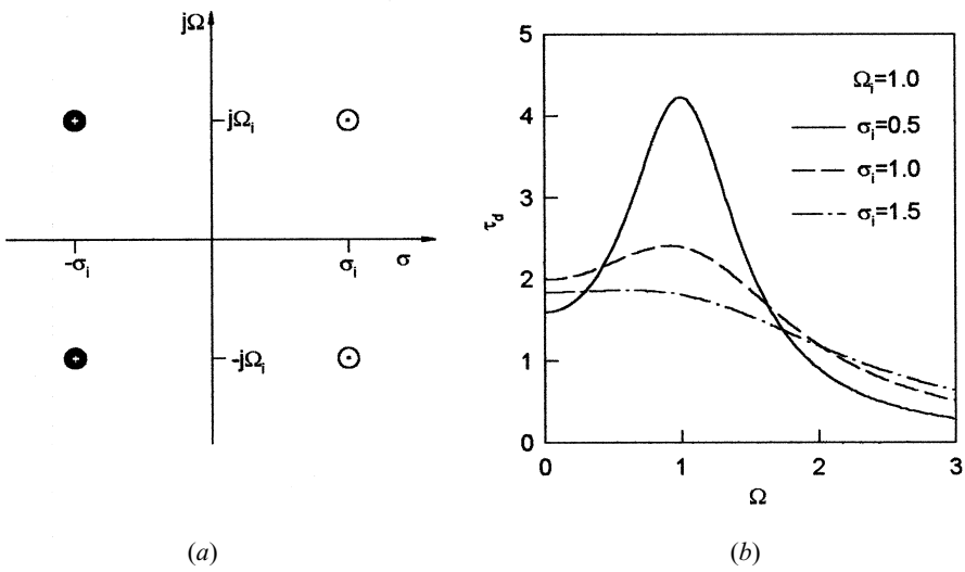
FIGURE 3.9 Characteristics of single-section, D-type, all-pass network: (a) pole-zero diagram, (b) group delay response.
