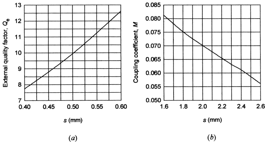
FIGURE 5.20 Design curves obtained by full-wave EM simulations for designing the microstrip combline filter. (a) External quality factor. (b) Coupling coefficient.
