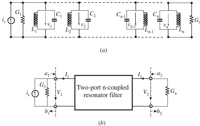
FIGURE 8.2 (a) Equivalent circuit of n -coupled resonators for node-equation formulation. (b) Its network representation.
