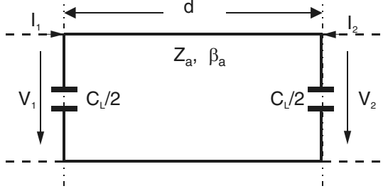
FIGURE 11.13 Capacitively loaded transmission line resonator.
