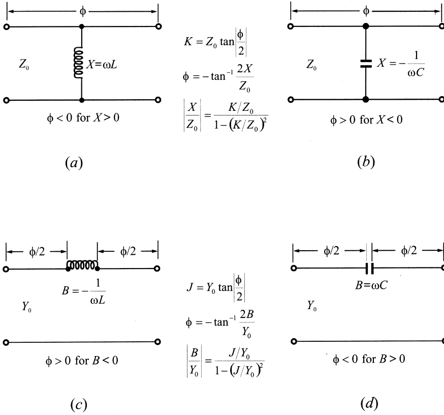
FIGURE 3.22 Immittance inverters comprised of lumped and transmission line elements.
