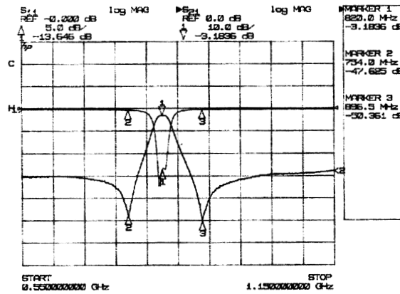
FIGURE 11.26 (a) Miniaturized 820 MHz bandpass filter with fractal microstrip dual-mode resonator on a 1.27 mm thick substrate with a relative dielectric constant of 10.8. (b) Measured performance of the filter.
