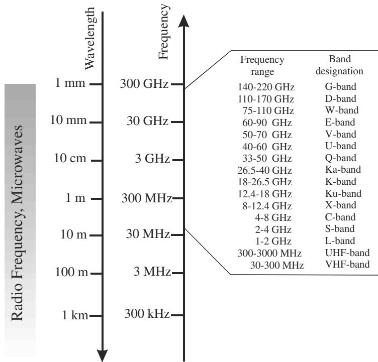
FIGURE 1.1 RF/microwave spectrums.
