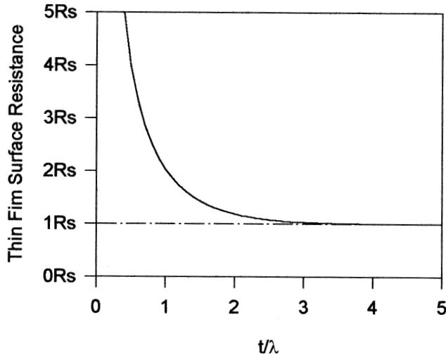
FIGURE 7.4 Surface resistance of superconducting thin films as a function of normalized thickness.
