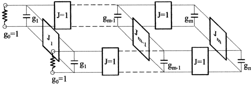
FIGURE 10.24 A lowpass prototype for design of RF/microwave linear phase filters.
