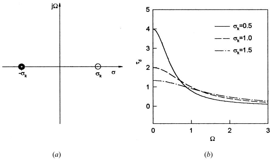
FIGURE 3.8 Characteristics of single-section C-type all-pass network: (a) pole-zero diagram, (b) group delay response.
