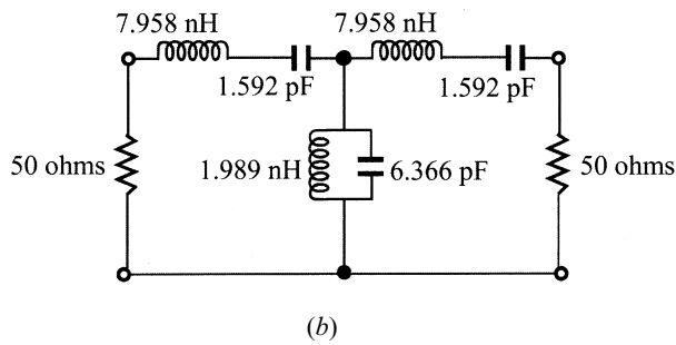
FIGURE 3.15 Lowpass prototype to bandpass transformation: (a) basic element transformation, (b) a practical bandpass filter based on the transformation.
