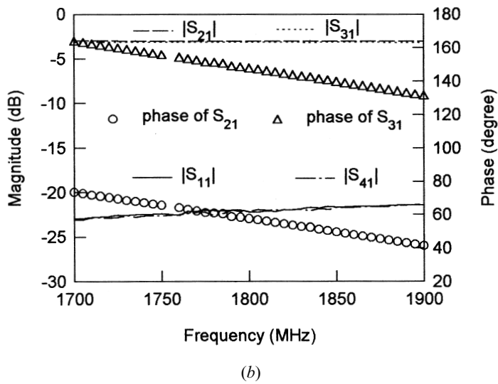
FIGURE 12.8 (a) Layout of HTS microstrip hybrid using tandem couplers on a 0.5 mm thick LAO substrate. (b) Full-wave simulated performance of the hybrid.
