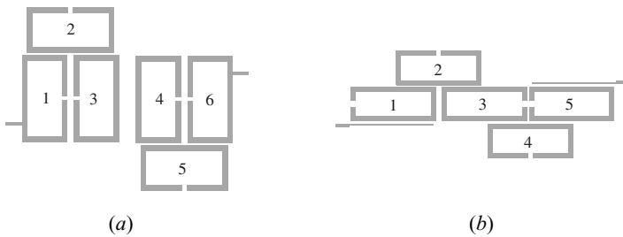
FIGURE 10.16 Configurations of microstrip CT filters.
