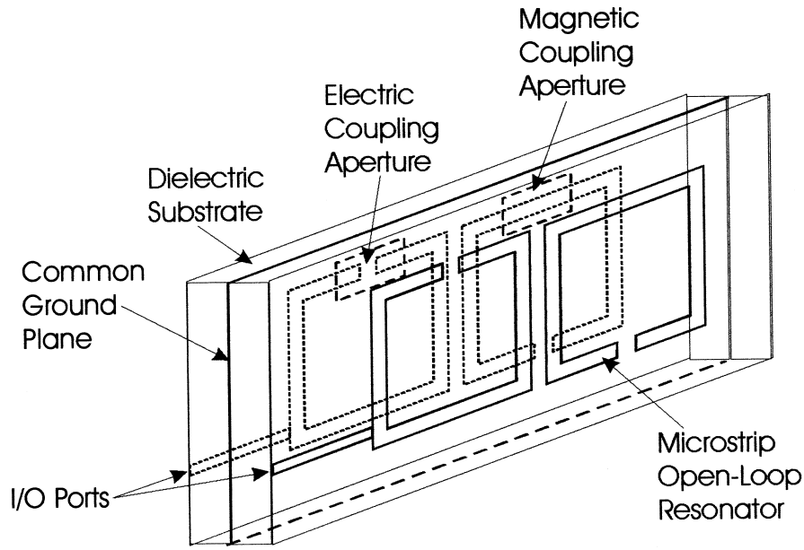
FIGURE 11.29 Structure of aperture-coupled microstrip open-loop resonator filter.
