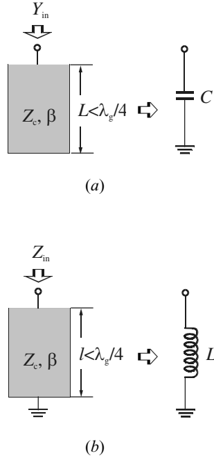
FIGURE 4.9 Short stub elements: (a) open-circuited stub; (b) short-circuited stub.
