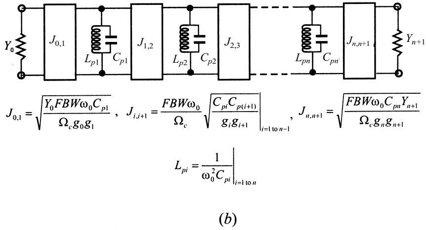
FIGURE 3.19 Bandpass filters using immittance inverters.
