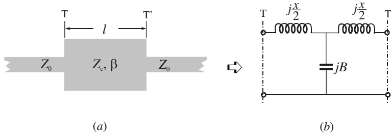
FIGURE 4.8 Low-impedance short-line element.
