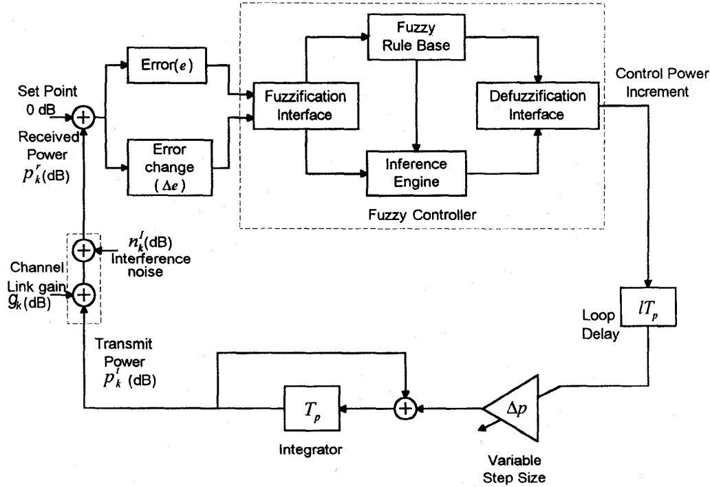
Fig. 1. Adaptive fuzzy power control system for CDMA mobile radio channels.
