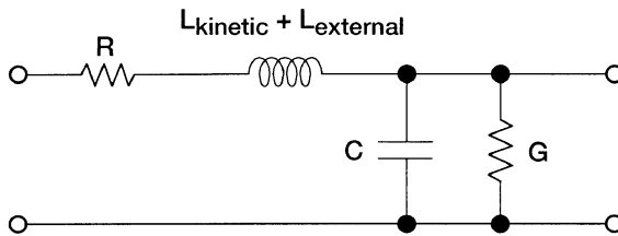
FIGURE 12.13 Lumped element equivalent circuit model for an incremental section of the superconducting coplanar waveguide.
