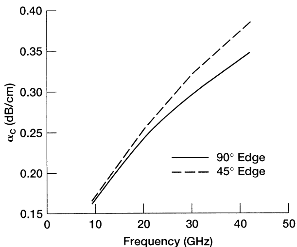
FIGURE 8.5 Computed attenuation constant due to conductor loss as a function of frequency for a CPW with 90° and 45° edges and t = 3 \mu\text{m} , a = 5 \mu\text{m} , b = 25 \mu\text{m} , \epsilon_r = 12.9 , g \rightarrow \infty , and \sigma_c = 3.0 \times 10^7 S/meter. (Reference [6], © IEEE 1995.)
