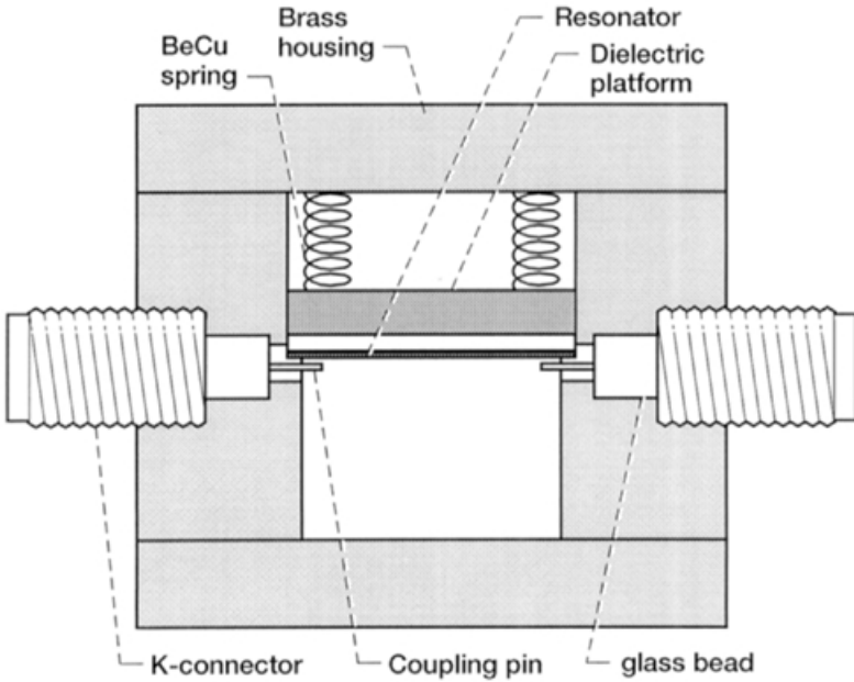
FIGURE 12.16 Schematic showing the flip chip assembly of the superconducting resonator within a microwave package mounted inside a closed-cycle cryo-cooler. (From Reference [19], © 1995 IEEE.)
