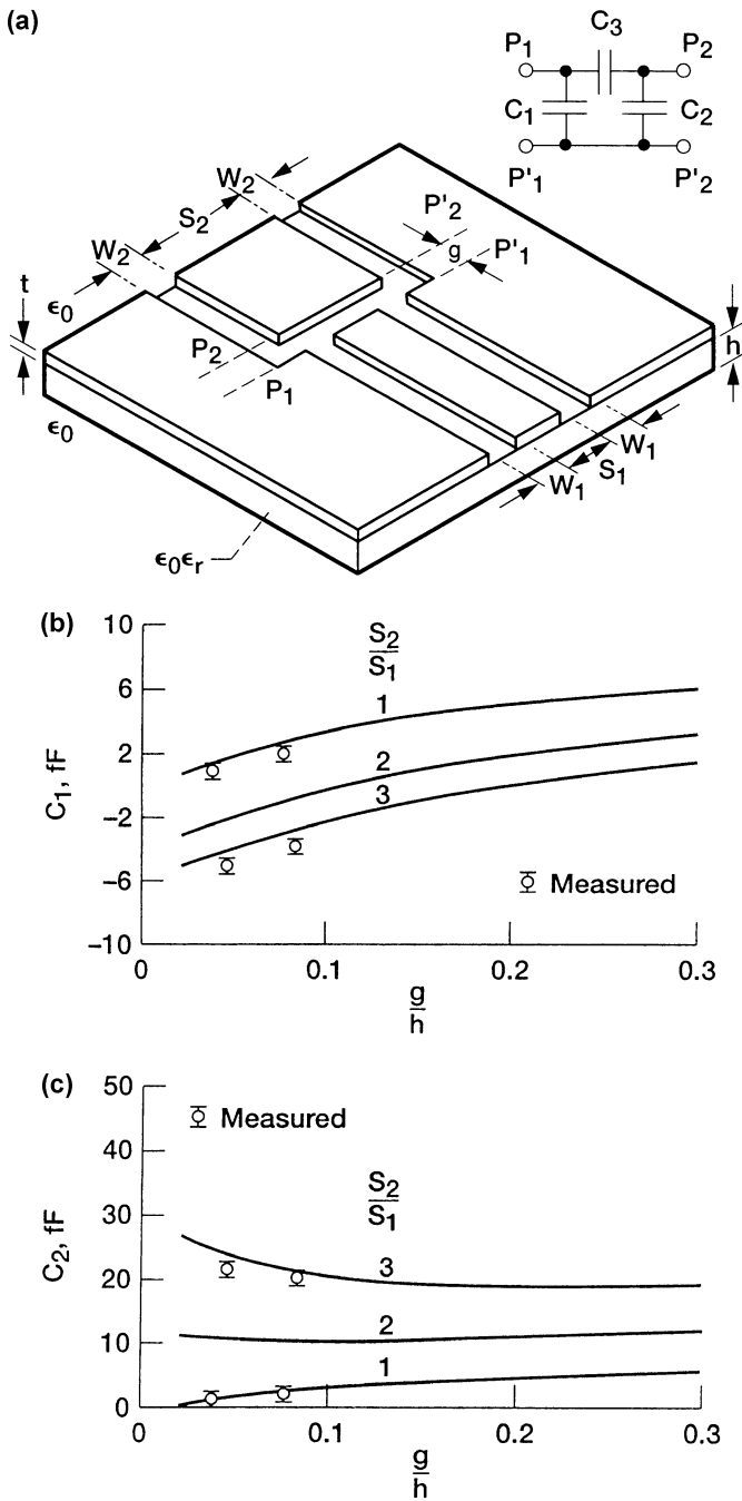
FIGURE 9.4 Series gap in the center strip conductor of a coplanar waveguide: (a) circuit layout; (b) computed fringing capacitance C_1 ; (c) computed fringing capacitance C_2 ; (d) computed coupling capacitance C_3 ; (e) effect of metallization thickness t on the coupling capacitance C_3 . (Reference [11], ©IEEE 1990.)
