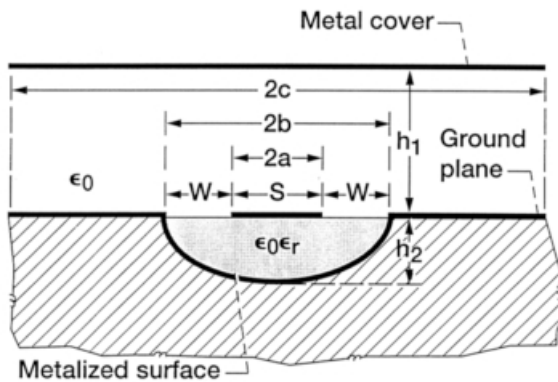
FIGURE 7.5 Elliptic-shaped microshield line.
