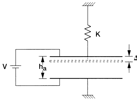
FIGURE 12.3 A simple lumped capacitor-spring model for the membrane switch.
