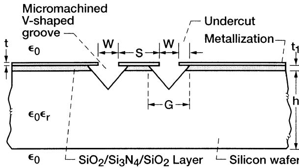
FIGURE 8.10 Coplanar waveguide with V-shaped micromachined grooves.
