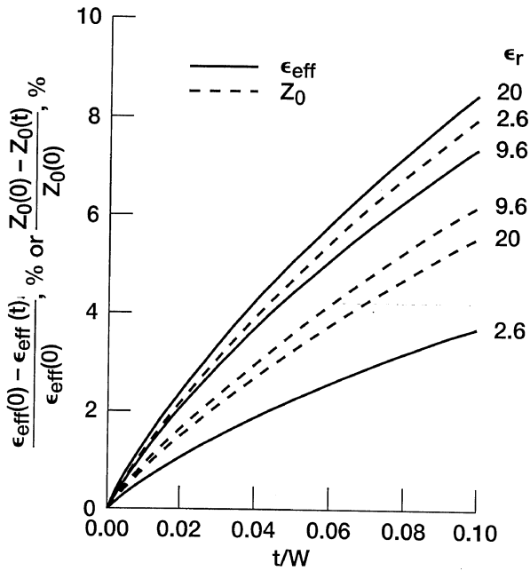
FIGURE 5.10 Computed percentage change in \epsilon_{\text{eff}} and Z_0 of shielded suspended CPW as a function of the normalized conductor thickness with the substrate dielectric constant as a parameter: S/h = 1.0 , (S + 2W)/h = 3.0 , (S + 2W + 2g)/h = 15.0 , (h_1 + t)/h = 3.0 , h_2/h = 3.0 , frequency = 0 GHz. (From Reference [4], copyright © IEE.)
