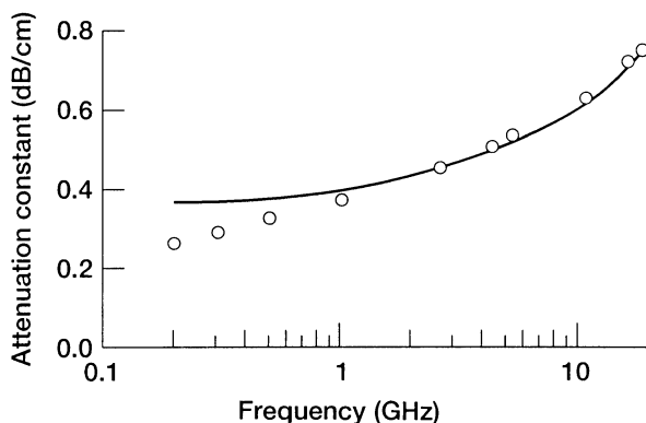
FIGURE 8.3 Comparison of computed and measured attenuation constant due to conductor loss as a function of the frequency for a CPW with t = 1.61 \mu\text{m} , a = 35.6 \mu\text{m} , b = 84.6 \mu\text{m} , \epsilon_r = 12.9 , g \rightarrow \infty , and \sigma_c = 3.602 \times 10^7 \text{ S/meter} (the circles are measured attenuation). (Reference [6], © IEEE 1995.)
