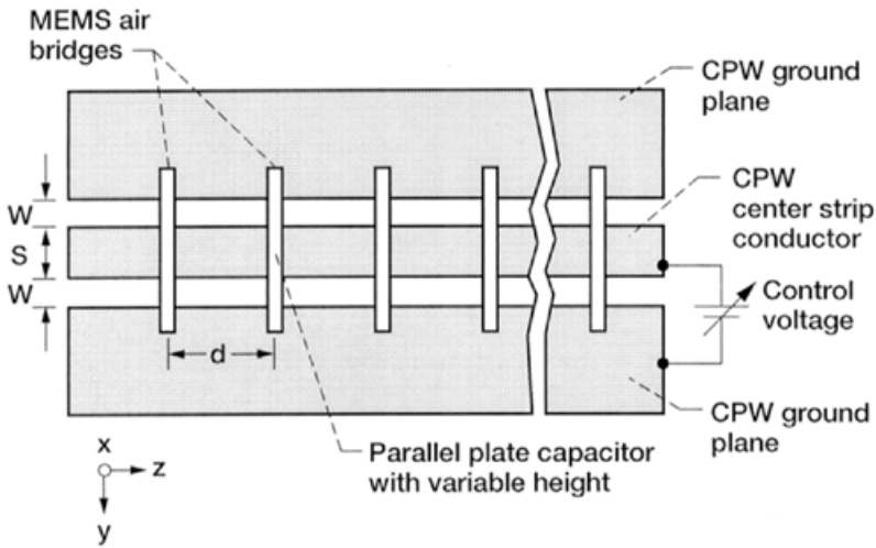
FIGURE 12.8 Schematic of a coplanar waveguide periodically loaded with MEMS air-bridge variable capacitors.
