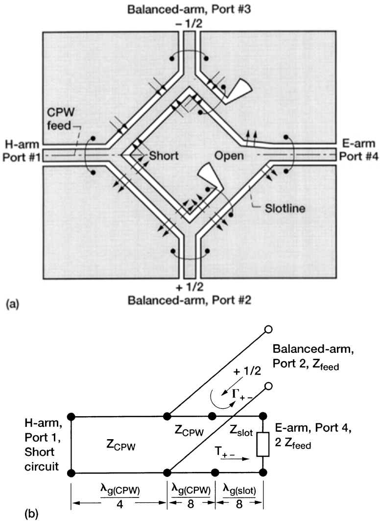
FIGURE 11.18 180° out-of-phase excitation at ports 2 and 3 of the magic-T: (a) Electric-field distribution; (b) simplified equivalent circuit.
