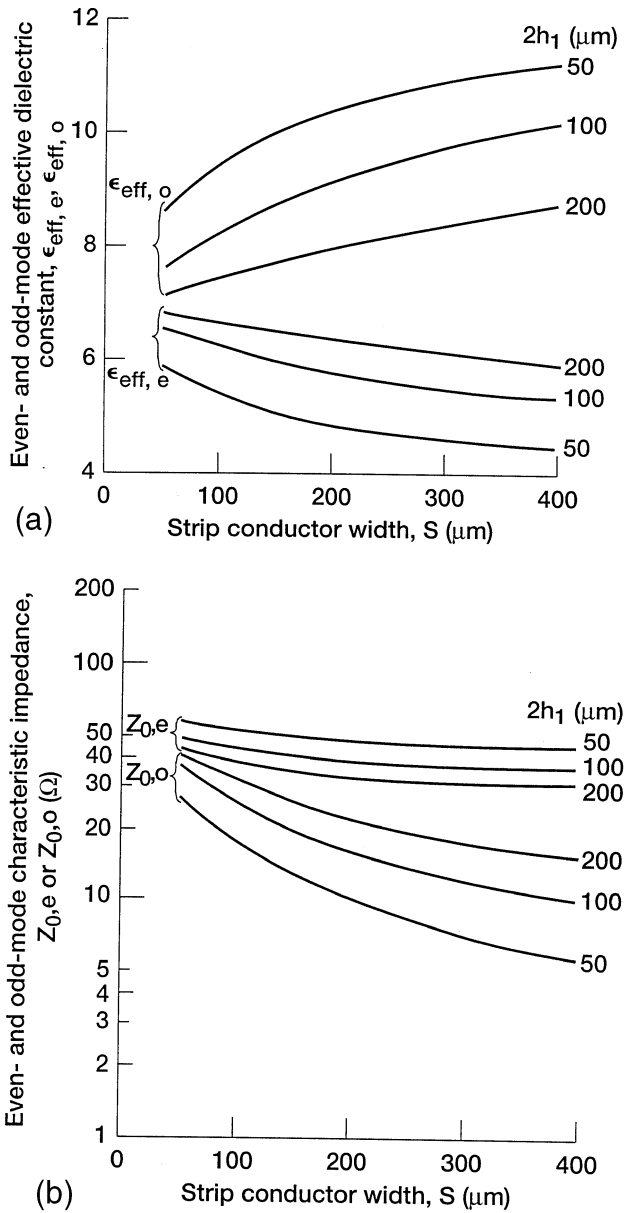
FIGURE 7.18 Computed even- and odd-mode (a) effective dielectric constant and (b) characteristic impedance, \epsilon_{r1} = 12.9 , \epsilon_{r2} = 1.0 , W = 20 \mu\text{m} , h_2 = 1 \text{ mm} . (From Reference [13], © IEEE 1989.)
