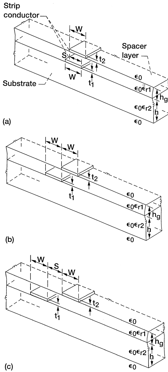
FIGURE 6.8 Micro-coplanar stripline (MCPS) configuration. (a) Strips overlap; (b) strip edges are even; (c) strips are separated.
