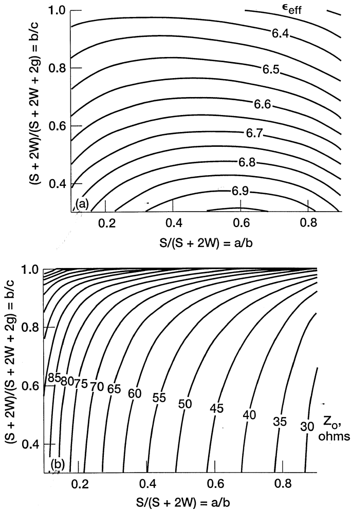
FIGURE 4.4 Contour of constant propagation parameters for FW-CPW, \epsilon_r = 13 , h/b = 1 : (a) Effective dielectric constant, \epsilon_{\text{eff}} ; (b) characteristic impedance, Z_0 . (From Reference [4], © 1987 IEEE.)
