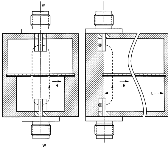
FIGURE 5.20 Cross-sectional view of the cavity showing magnetic-field lines for the dominant mode resonance. The magnetic wall symmetry is denoted by the plane mw .
