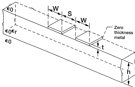
FIGURE 6.7 Coplanar stripline configuration.
