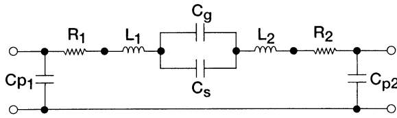
FIGURE 9.28 Lumped element equivalent circuit model for the series MIM capacitor.
