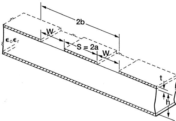
FIGURE 3.1 Schematic of conductor backed coplanar waveguide (CBCPW).
