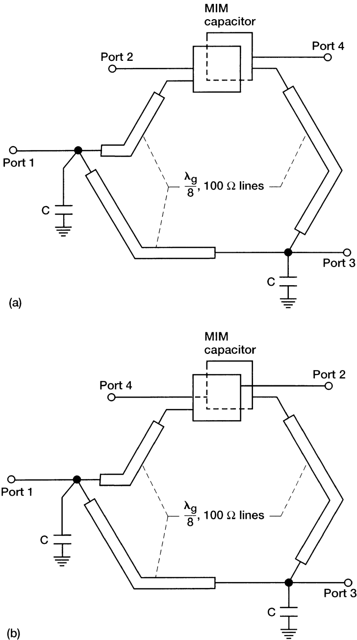
FIGURE 11.13 (a) Normal port layout; (b) port layout convenient for balanced mixer applications.
