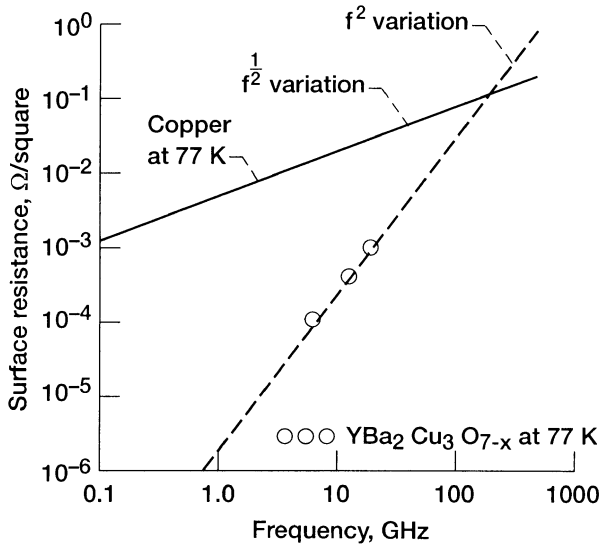
FIGURE 12.19 Measured surface resistance of YBa 2 Cu 3 O 7-x as a function of frequency at 77 K. (From Reference [17], © 1993 American Institute of Physics.)
