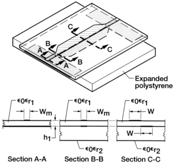
FIGURE 10.40 Two back-to-back micro-coplanar stripline-to-microstrip transition.
