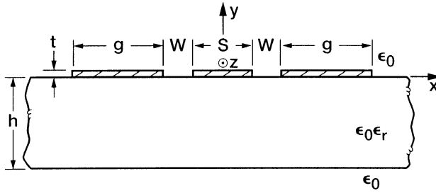
FIGURE 8.1 Coplanar waveguide with finite thickness conductors.
