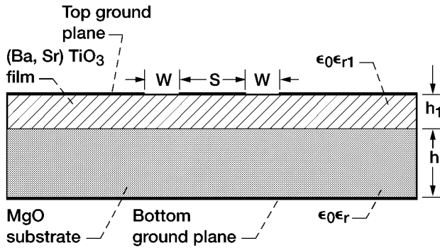
FIGURE 12.24 Schematic showing the cross-section of the phase-shifter: h = 500 \mu\text{m} , h_1 = 8 \mu\text{m} , S = 60 \mu\text{m} , W = 40 \mu\text{m} , \epsilon_r = 9.7 , \epsilon_{r1} is bias dependent.
