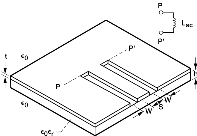
FIGURE 9.2 Coplanar waveguide short circuit.
