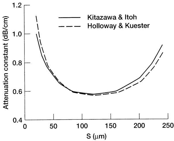
FIGURE 8.7 Computed attenuation constant due to conductor loss as a function of center strip conductor width S for a CPW with t = 3.0\ \mu\text{m} , b = 150.0\ \mu\text{m} , \epsilon_r = 12.8 , g \rightarrow \infty , and \sigma_c = 5.882 \times 10^7\ \text{S/meter} . (Reference [6], © IEEE 1995.)
