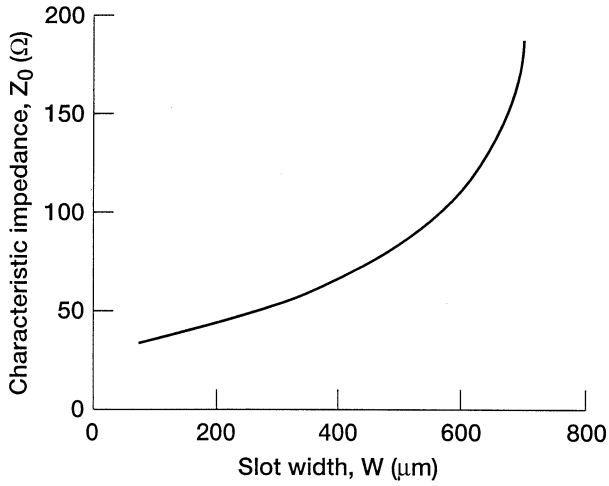
FIGURE 7.6 Computed Z_0 as a function of the slot width, \epsilon_r = 2.55 , h_1 = 3.0 mm, h_2 = 400 \mu\text{m} , b = 692.82 \mu\text{m} . (From Reference [8], © IEEE 1994.)
