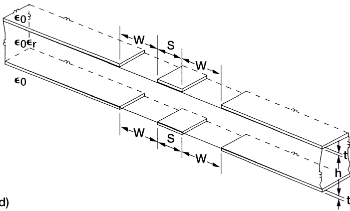
FIGURE 11.1 Coupled-line configurations: (c) edge coupled grounded CPW with metal underpass; (d) broadside coupled CPW.
