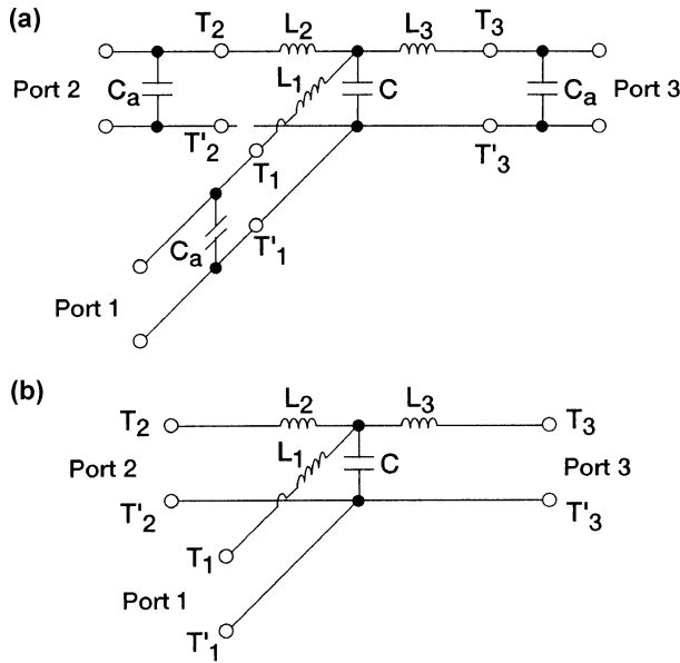
FIGURE 9.21 Lumped element equivalent circuit model: (a) Conventional T-junction; (b) air-bridge T-junction.
