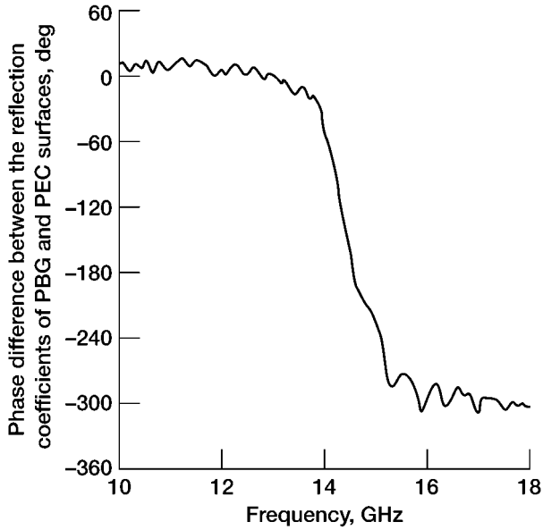
FIGURE 12.29 Measured phase difference between the reflection coefficients of a photonic-bandgap surface and a perfect electrically conducting surface. (From reference [34], © IEEE 1999.)
