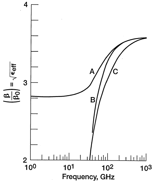
FIGURE 5.14 The quasi-TEM dominant mode (A) and the first higher-order mode (C) dispersion characteristics of a shielded grounded CPW: S = 0.14 mm, 2B = 2 mm, h = 0.2 mm, W = 0.28 mm, h_1 = 2 mm, \epsilon_r = 12.9 , t = 0 . (From Reference [8], copyright © IEE.)
