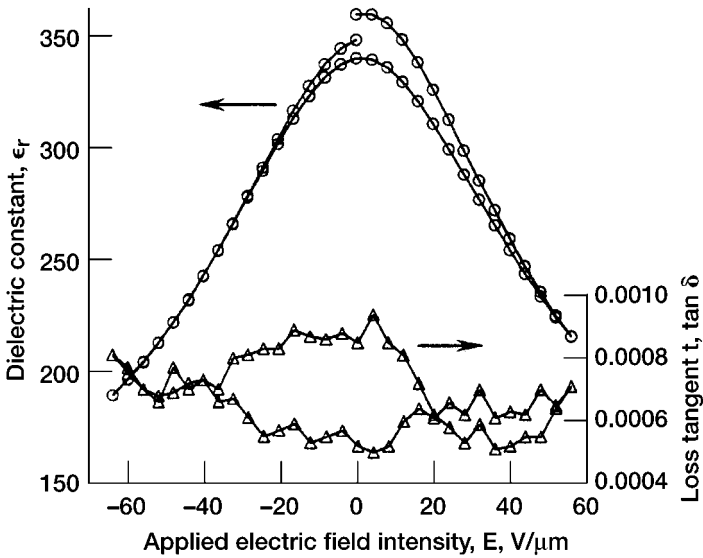
FIGURE 12.22 Measured dielectric characteristics of 2.5 \mu m thick SrTiO_3 film as a function of the applied dc electric field intensity at a fixed temperature of 190 K. (From reference [28], © 1998 American Institute of Physics.)
