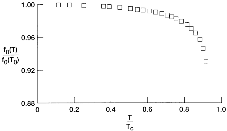
FIGURE 12.17 Measured normalized resonance frequency as a function of the temperature for a YBa_2C_3O_{7-x} coplanar waveguide resonator. For material characteristics and resonator dimensions refer to data for sample 3/circuit 1 in Tables 12.2 and 12.4. (From Reference [17], © 1993 American Institute of Physics.)
