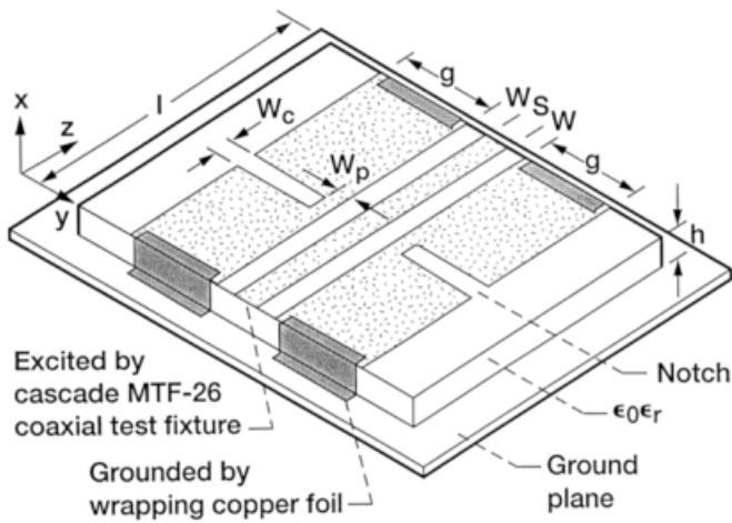
FIGURE 4.9 Schematic of the 50Ω FW-CBCPW through line with two notches cut in the top ground plane: S = W = 0.508 mm, g = 6.0 mm, l = 18.0 mm, W_p = 1.0 mm, W_c = 1.016 mm, h = 0.635 mm, \epsilon_r = 10.2
