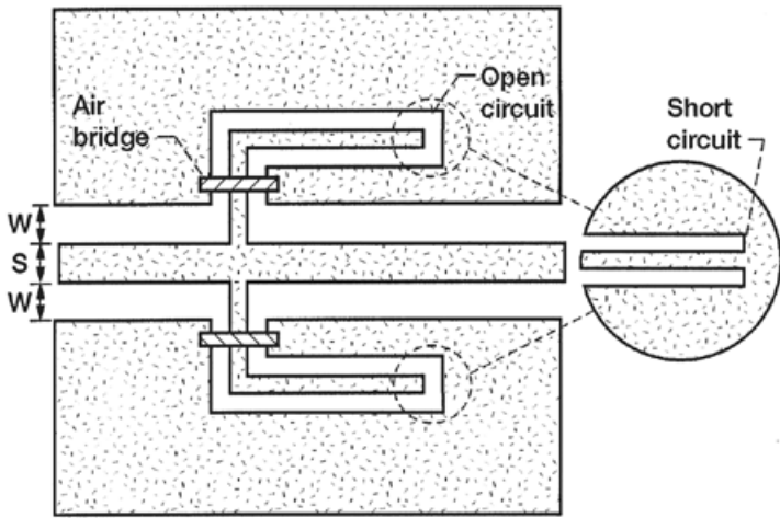
FIGURE 9.39 Open end coplanar waveguide shunt stub. Inset shows a short-end shunt stub.
