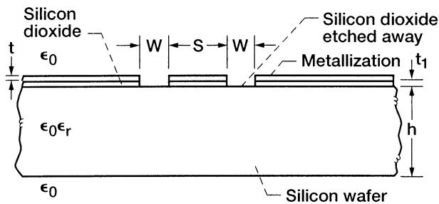
FIGURE 8.9 Coplanar waveguide on a silicon wafer with a thin interfacial layer of silicon dioxide.
