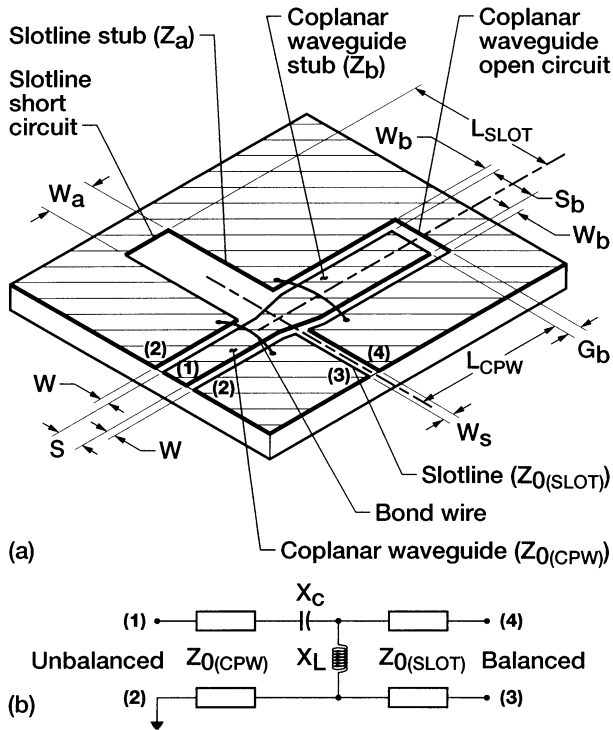
FIGURE 10.25 Coplanar waveguide-to-slotline compensated Marchand balun or transition: (a) Circuit layout; (b) lumped element equivalent circuit model.
