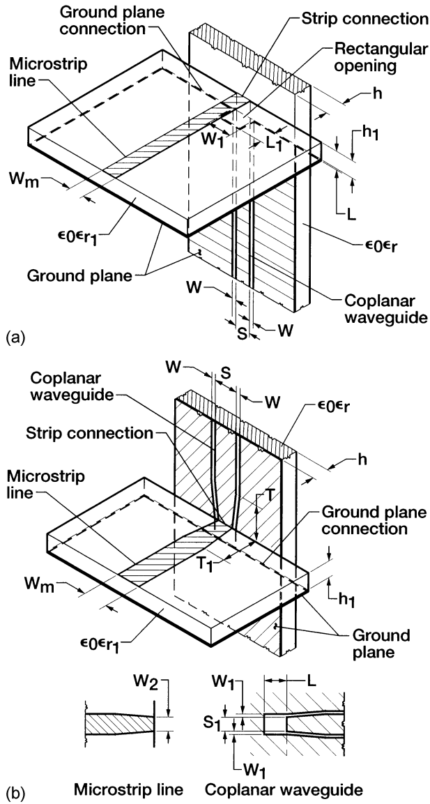
FIGURE 10.6 Coplanar waveguide-to-microstrip orthogonal transition via direct contact: (a) Connection is from the bottom, h = h_1 = 0.63 mm, \epsilon_r = \epsilon_{r1} = 6.0 , S = 0.93 mm, W = 0.20 mm, L = 0.65 mm, W_1 = 1.33 mm, L_1 = 0.42 mm, W_m = 0.93 mm; (b) connection is from the top, h = h_1 = 0.63 mm, \epsilon_r = \epsilon_{r1} = 6.0 , S = 0.93 mm, W = 0.20 mm, T = 0.99 mm, L = 0.65 mm, S_1 = 0.65 mm, W_1 = 0.3 mm, W_m = 0.93 mm, T_1 = 0.99 mm, W_2 = 0.65 mm.
