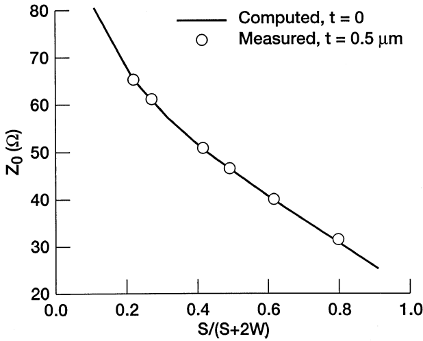
FIGURE 2.18 Computed and measured characteristic impedance as a function of S/(S + 2W) : \epsilon_r = 12.9 , h_1 = 0.5 mm, S = 75 \mu m. (From Reference [26], © IEEE 1991.)
