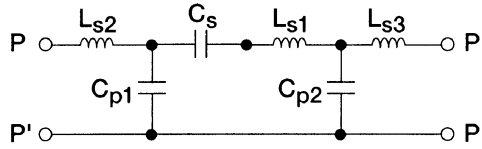
FIGURE 9.34 Lumped element equivalent circuit model for the open end coplanar waveguide series stub.
