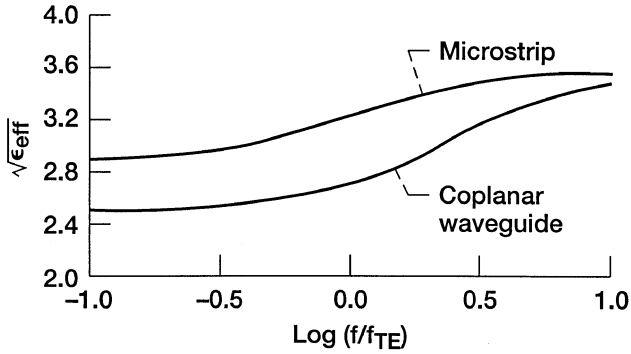
FIGURE 2.19 Computed effective dielectric constant as a function of normalized frequency. (From Reference [28], © IEEE 1986.)
