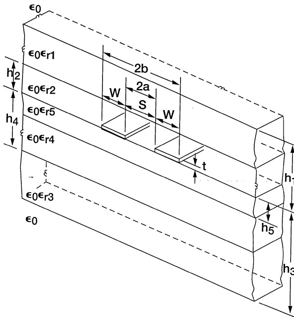
FIGURE 6.1 Schematic of a coplanar stripline (CPS) on a multi-layer dielectric substrate.
