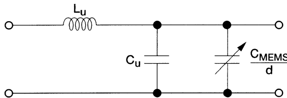
FIGURE 12.9 Lumped element equivalent circuit model for an incremental section of the loaded coplanar waveguide.
