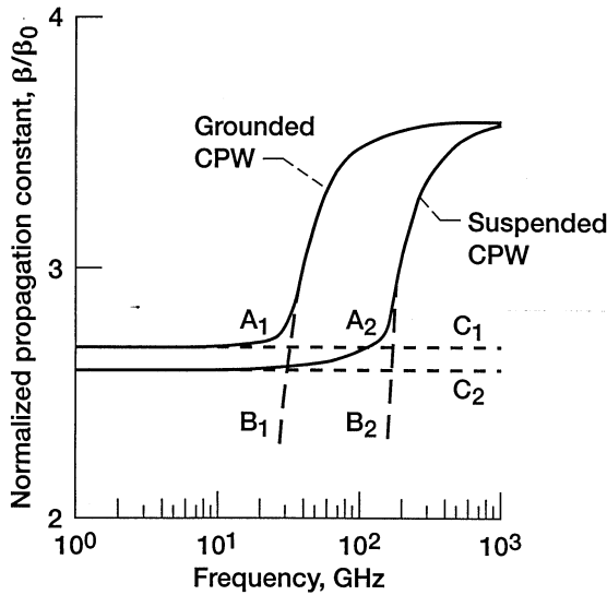
FIGURE 5.12 Computed dispersion characteristics of a shielded grounded CPW ( A_1 ) and a shielded suspended CPW ( A_2 ): S = 0.14 mm, 2B = 2 mm, h = 0.2 mm, W = 10 mm, \epsilon_r = 12.9 , t = 0 . For shielded grounded CPW, h_1 = 2 mm, and for shielded suspended CPW, h_1 = h_2 = 1 mm. (From Reference [16], © 1992 IEEE.)
