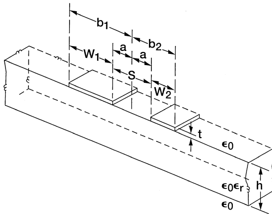
FIGURE 6.4 Schematic of asymmetric coplanar stripline (ACPS) on a dielectric substrate of finite thickness.
