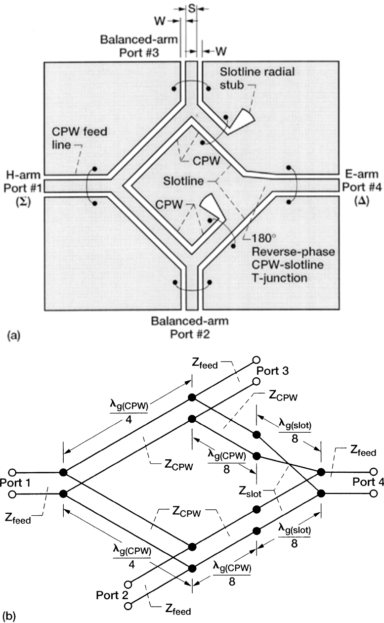
FIGURE 11.16 Standard 3-dB magic-T: (a) circuit configuration (from Reference [14], © 1994 IEEE); (b) equivalent transmission line model. The wavelength on the line is denoted as \lambda_g .
