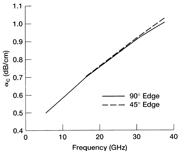
FIGURE 8.6 Computed attenuation constant due to conductor loss as a function of frequency for a CPW with 90° and 45° edges and t = 1.61 \mu\text{m} , a = 35.6 \mu\text{m} , b = 84.6 \mu\text{m} , \epsilon_r = 12.9 , g \rightarrow \infty , and \sigma_c = 3.602 \times 10^7 S/meter. (Reference [6], © IEEE 1995.)
