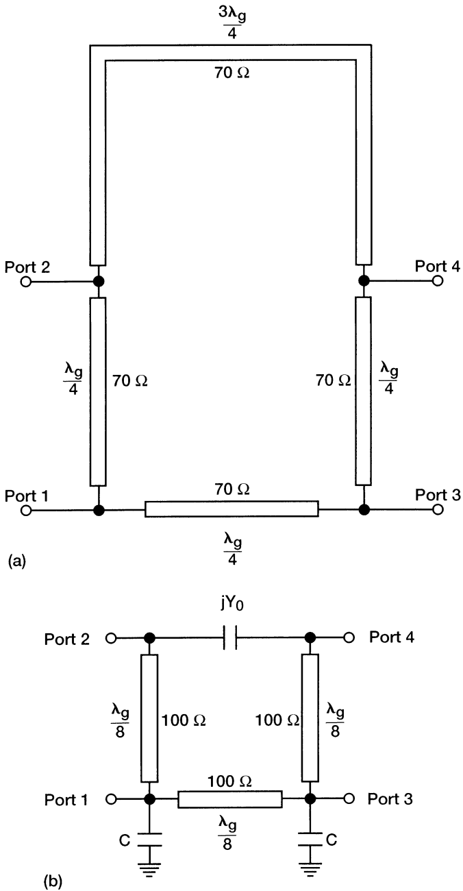
FIGURE 11.12 Representation of (a) standard 180° ring hybrid or rat race with transmission lines and (b) equivalent reduced size 180° ring hybrid or rat race with transmission lines and lumped elements. The wavelength on the line is denoted as \lambda_g .
