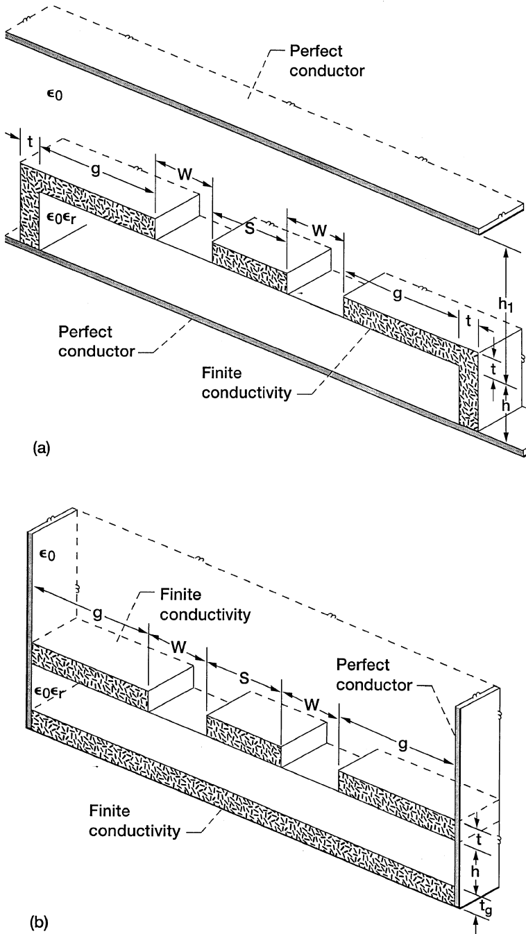
FIGURE 3.12 Cross-sectional geometry of CBCPW considered in the (a) mode-matching method and (b) method of lines.
