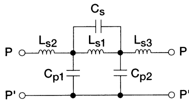
FIGURE 9.37 Lumped element equivalent circuit model for the short-end coplanar waveguide series stub.
