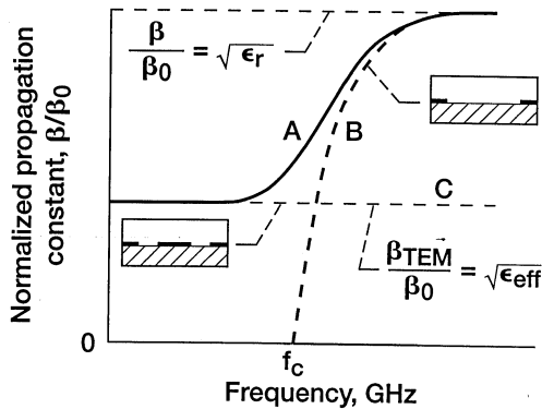
FIGURE 5.11 Typical dispersion characteristics of the grounded CPW dominant mode, which is considered as a superposition of the grounded slot line mode and the quasi-TEM mode of the grounded CPW. (From Reference [16], © 1992 IEEE.)
