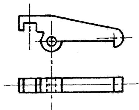
EXTRACTOR
