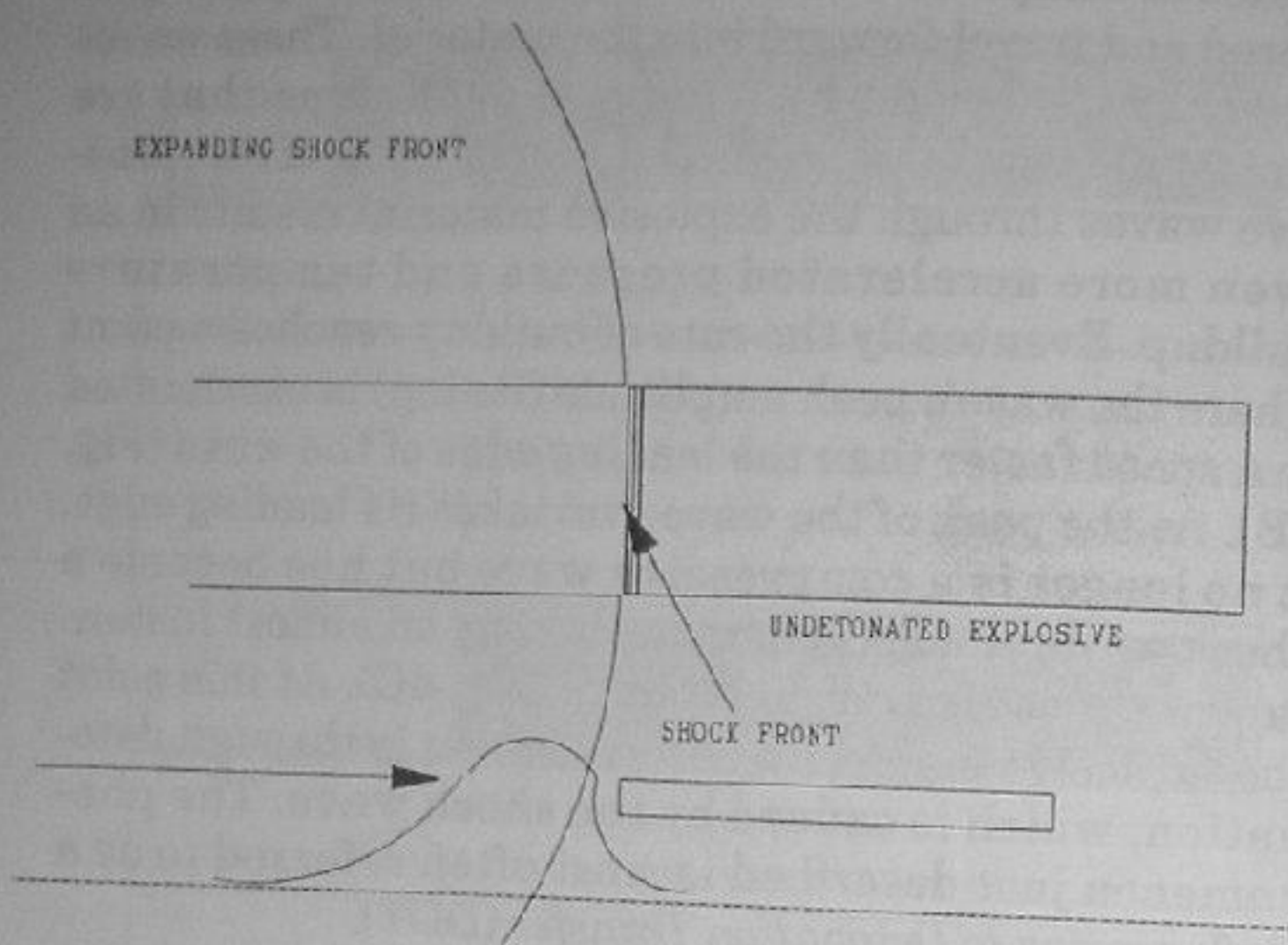
Figure 5. Shock wave.
