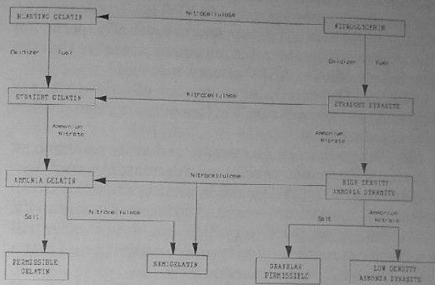
Figure 17. Dynamites and their composition.
