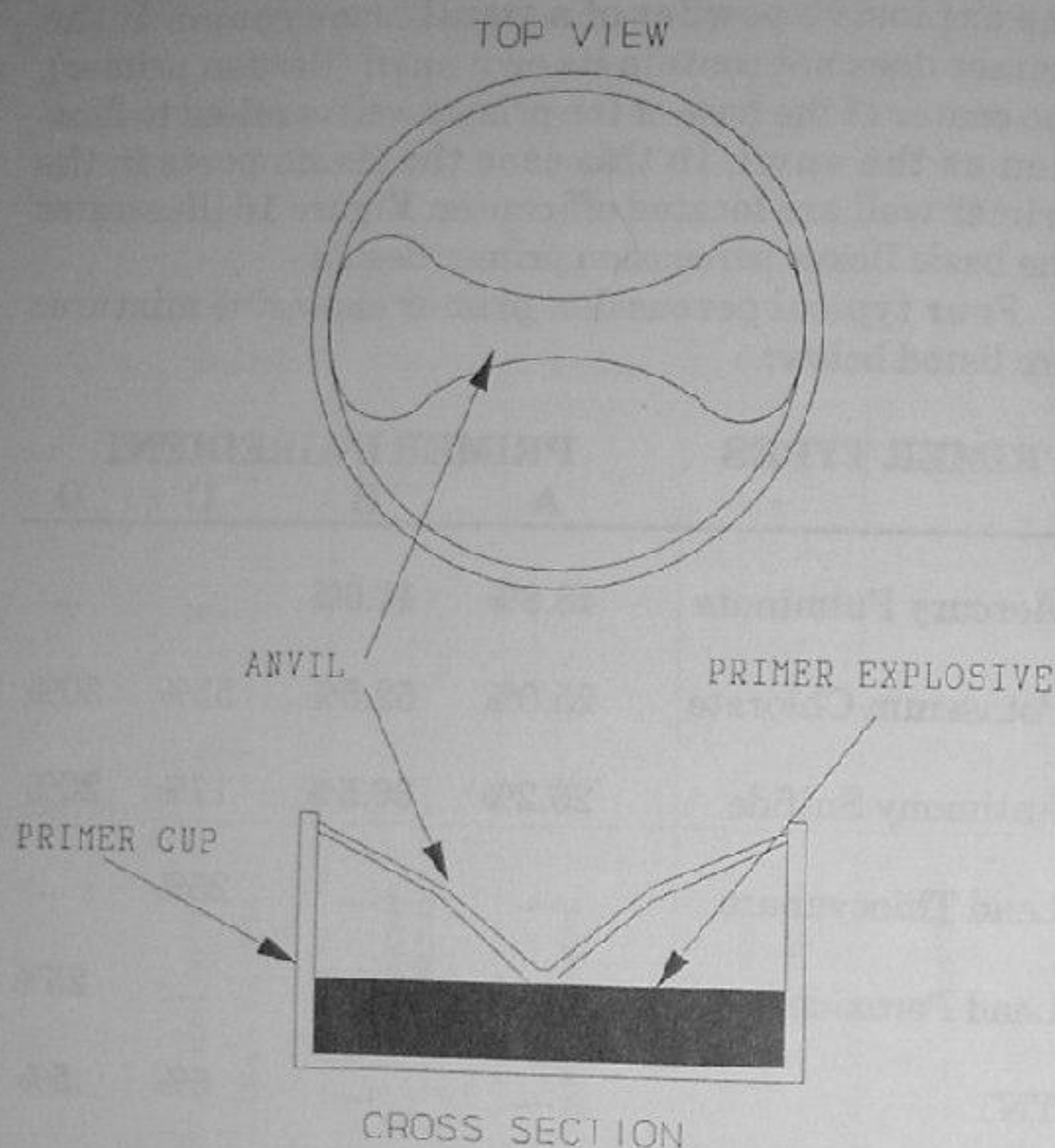
Figure 16. Percussion primer.
