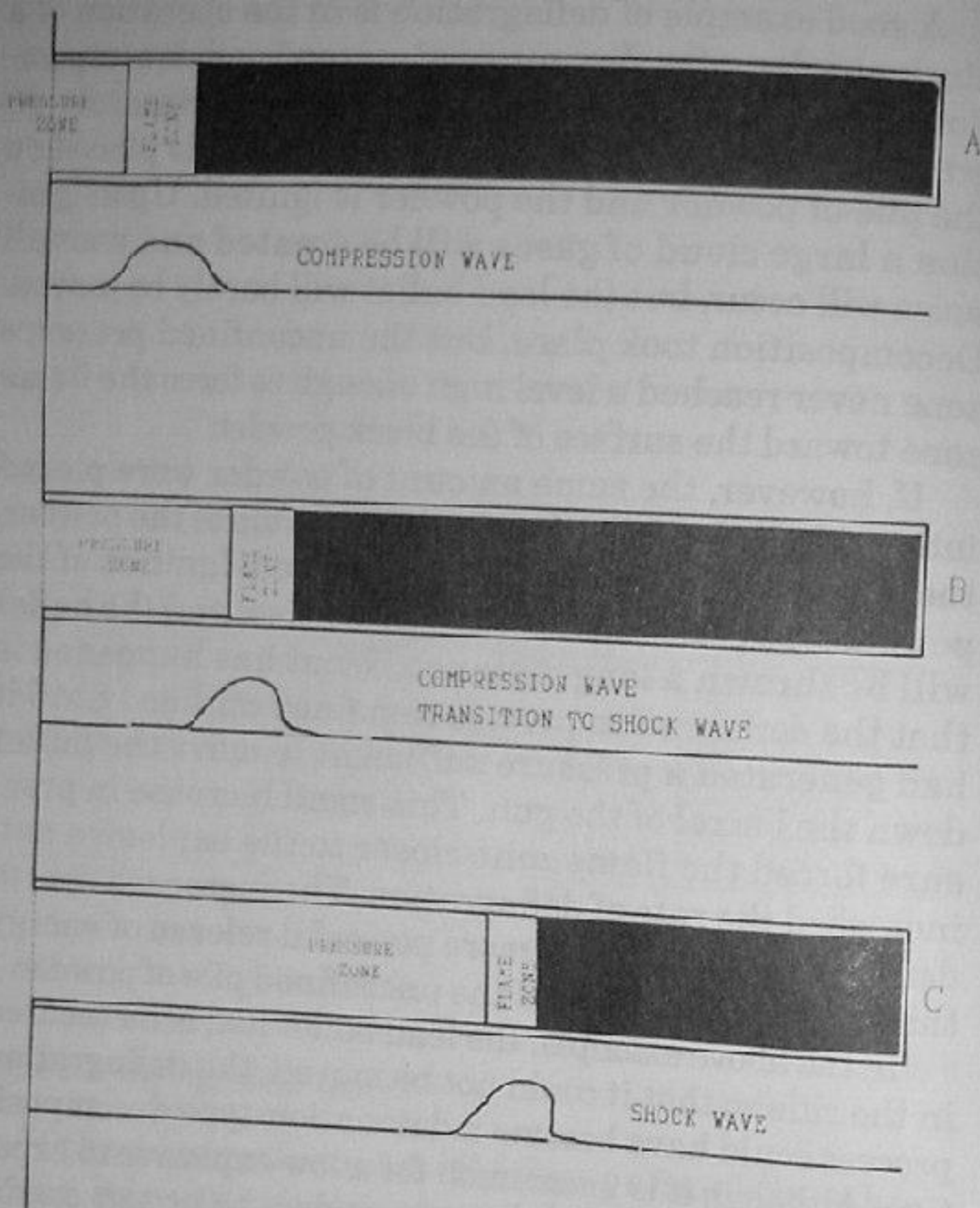
Figure 4. Deflagration to detonation transfer.
