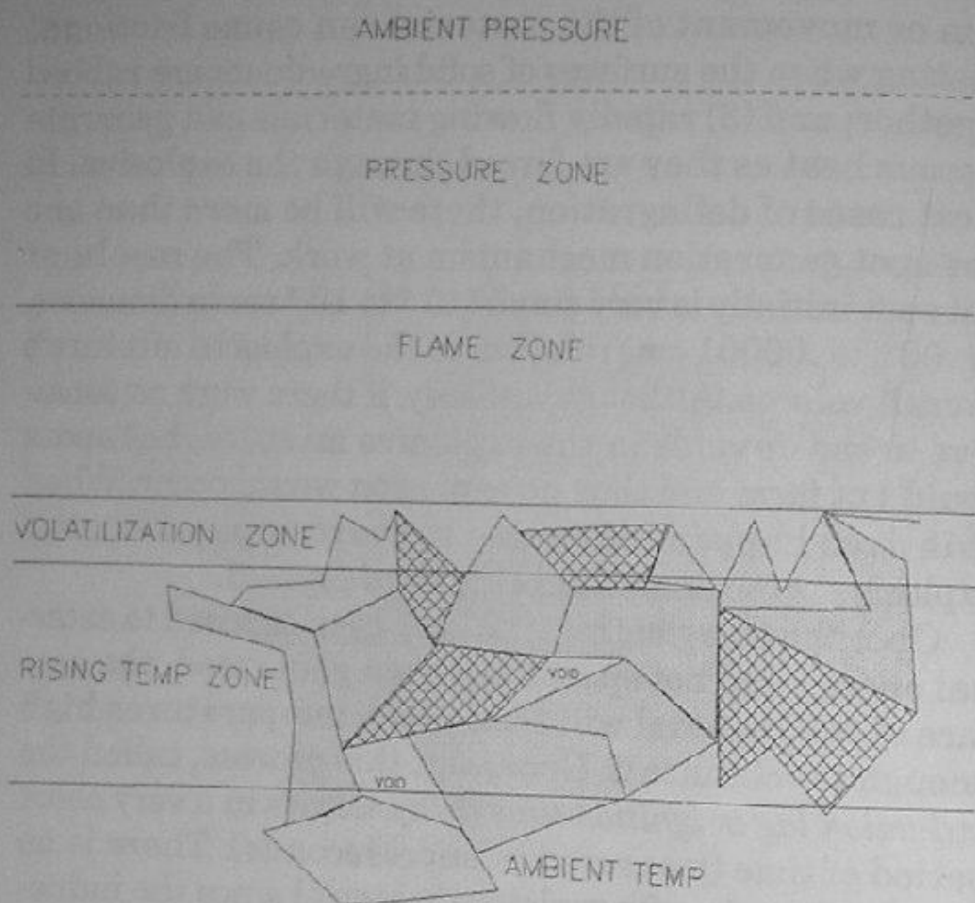
Figure 3. Deflagration zones.
