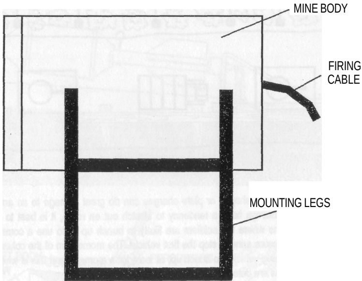
SIDE VIEW
