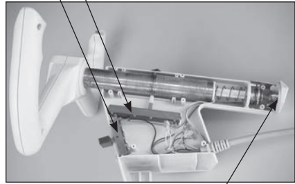
rotating potentiometer
