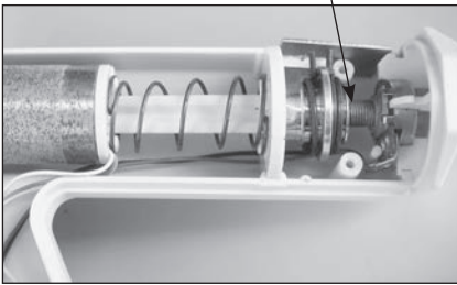
rotating potentiometer
