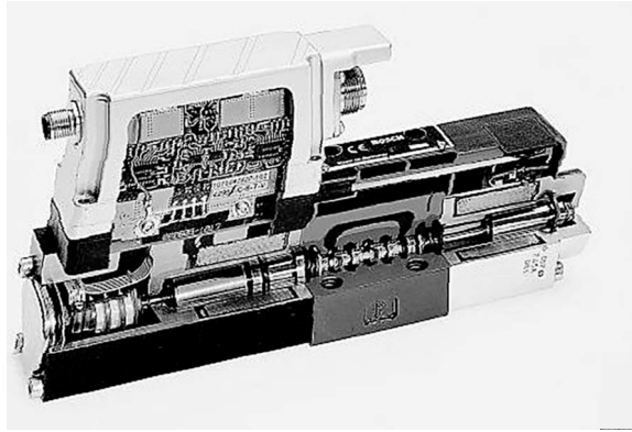
FIGURE 20.106 Flow proportional valve (Bosch Rexroth).
