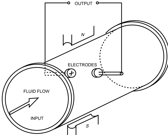
FIGURE 45.14 Electromagnetic flowmeter.
