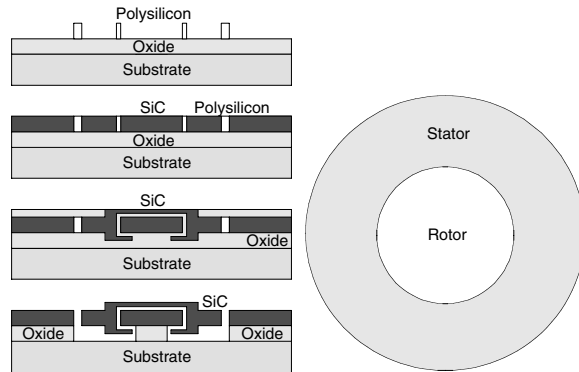
FIGURE 20.139 Fabrication of the SiC micromotors: cross-sectional schematics.
