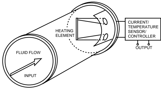
FIGURE 45.13 Thermal anemometer.
