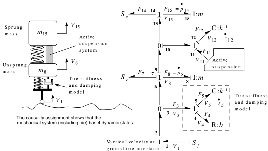
FIGURE 9.25 Example of model for vertical vibration in a quarter-car suspension model with an active suspension element. This example builds on the simple mass-spring-damper model, and shows how to integrate an actuator into a bond graph model structure.
