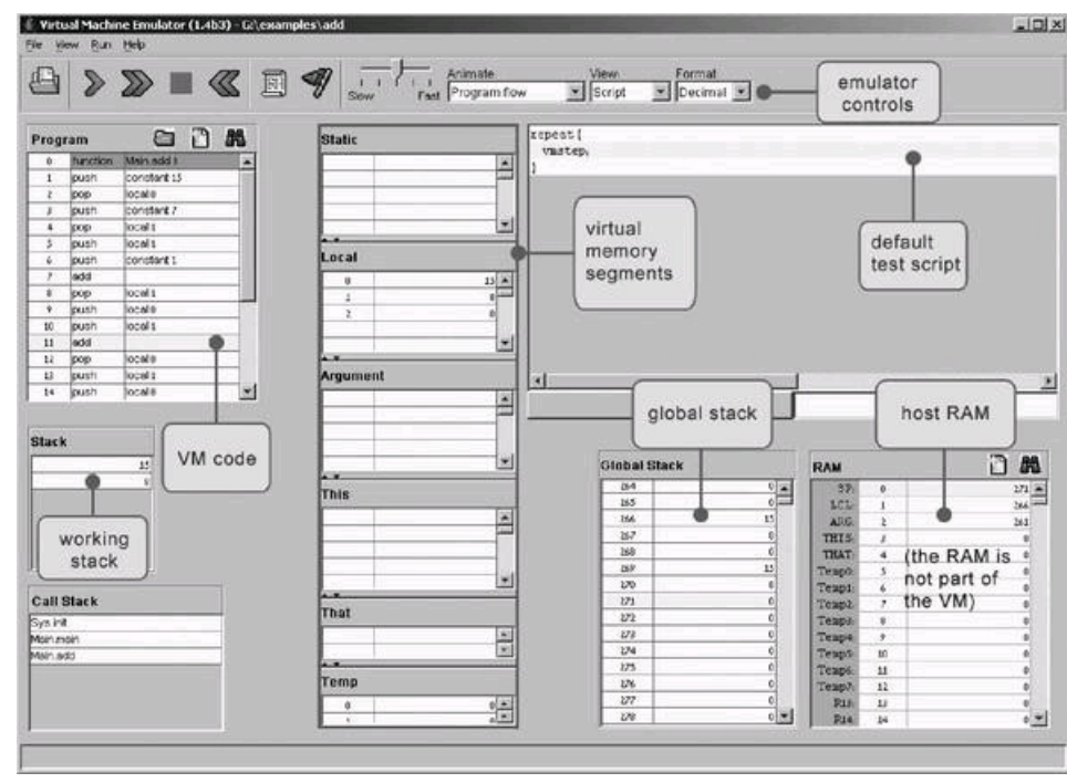
Figure 7.12 The VM emulator supplied with the book.
