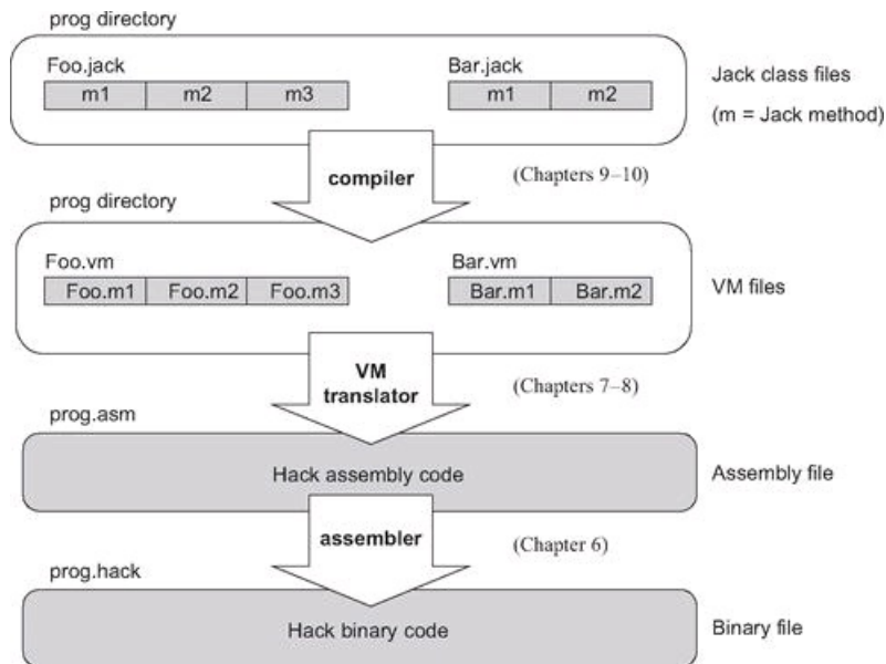
Figure 7.8 Program elements in the Jack-VM-Hack platform.
