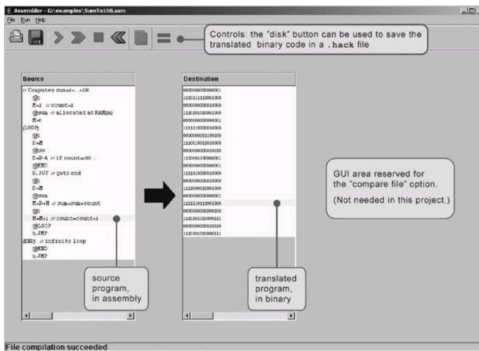
Figure 4.7 The visual assembler supplied with the book.
