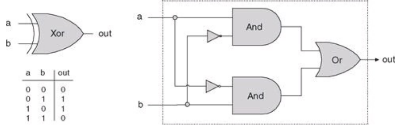
Figure 1.5 Xor gate, along with a possible implementation.
