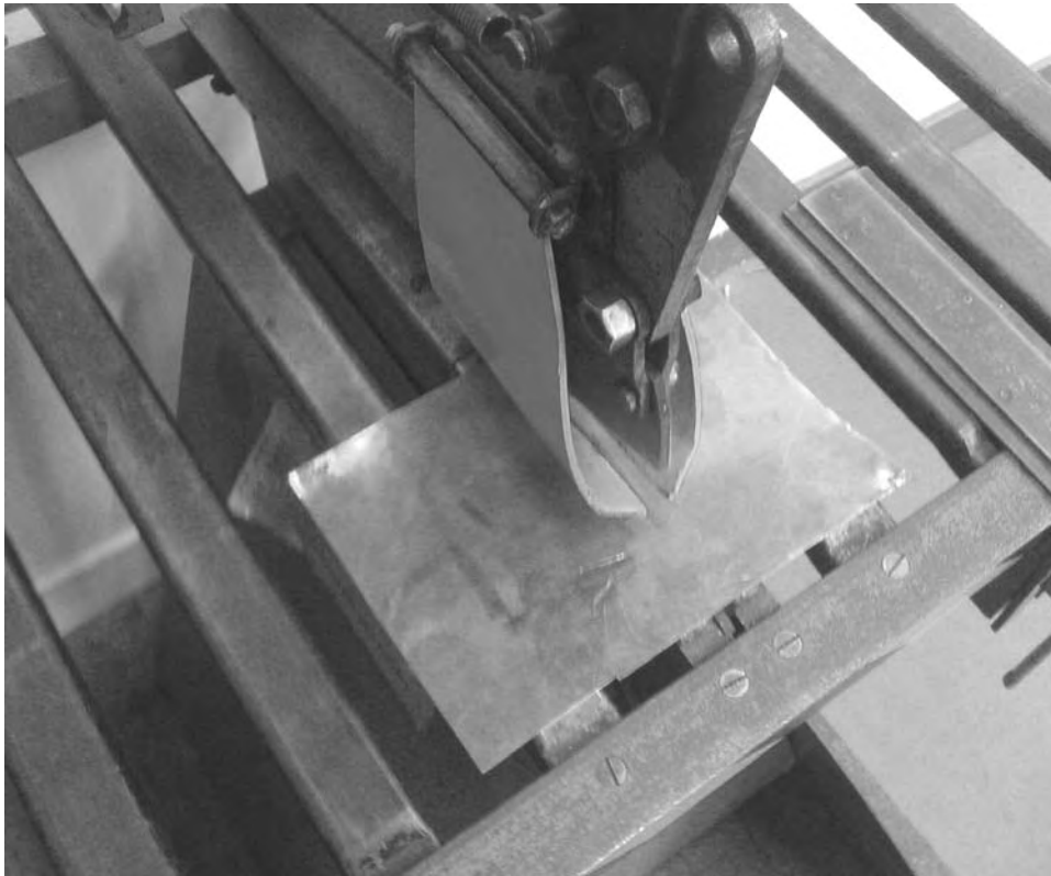
Figure 10-12 Cutting the copper with a guillotine.
