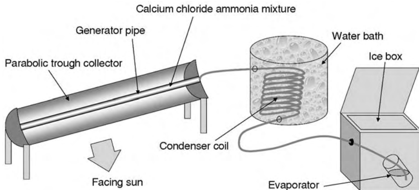
Figure 5-3 Solar cooler layout.
