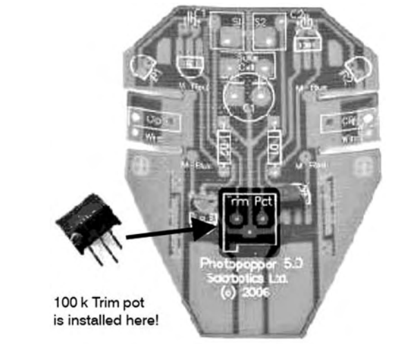
Figure 16-7 Adding the trimmer potentiometer. Image courtesy Solarbotics.
