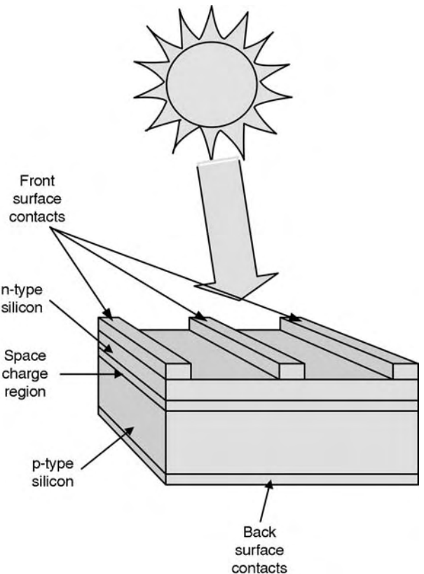
Figure 10-6 Cutaway solar cell.
