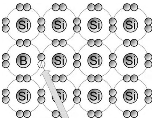
Electron hole
