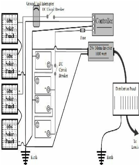
The holiday home wiring diagram
