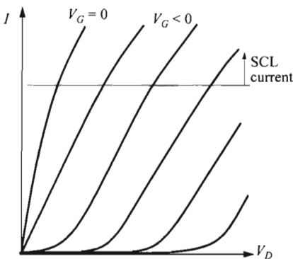
Fig. 32 Output characteristics of an SIT. At higher current levels, space-charge-limited current dominates.
