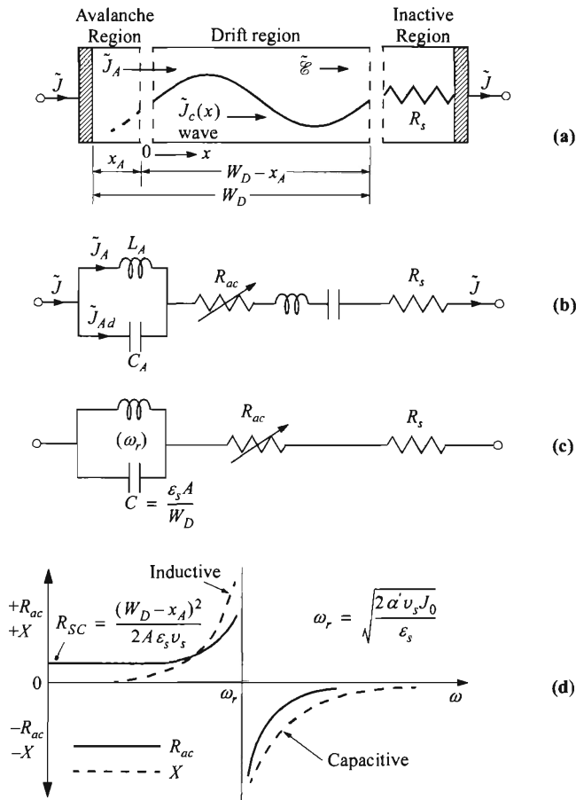
Fig. 7 (a) Model of Read diode with avalanche, drift, and inactive regions, and (b) its equivalent circuit. For small transit angle \theta , (c) equivalent circuit and (d) plots of real and imaginary parts of impedance vs. angular frequency \omega (After Ref. 7.)
