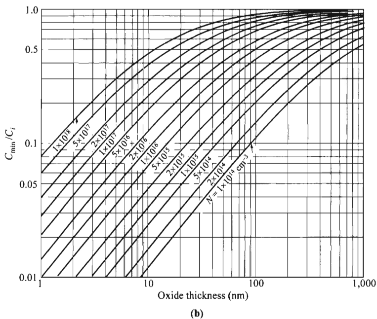
Fig. 11 Critical parameters of ideal SiO 2 -Si MOS capacitors as a function of doping level and oxide thickness. (a) Flat-band capacitance (normalized). (b) Low-frequency C_{\min} (normalized) (c) High-frequency C'_{\min} (normalized). (d) V_T and low-frequency V_{\min} .
