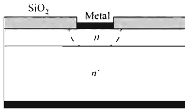
(a) Small-area contact
