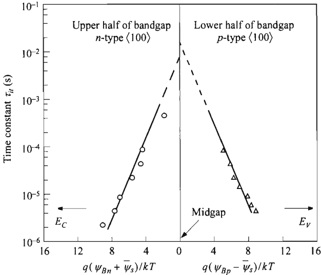
Fig. 17 Variation of trap time constant \tau_{ii} vs. energy. T = 300 K. (After Ref. 24.)
