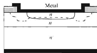
(h) Metal-overlap laterally diffused
