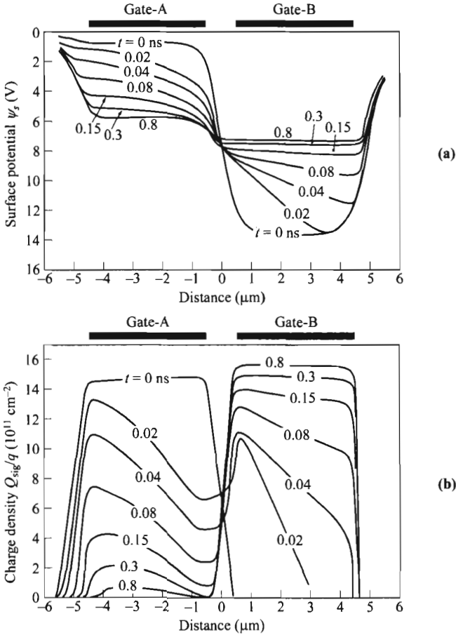
Fig. 30 (a) Time-dependent surface potential distribution under the storage and transfer gate (of length 4- \mu\text{m} ). (b) Transient charge distribution under the gates. (After Ref. 48.)
