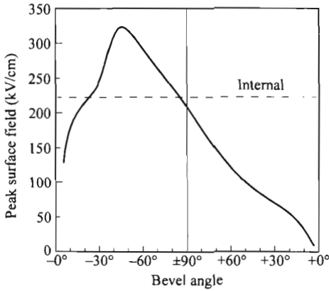
Fig. 7 Peak electric field along bevel surface for both positive and negative bevel angles. (After Ref. 16.)
