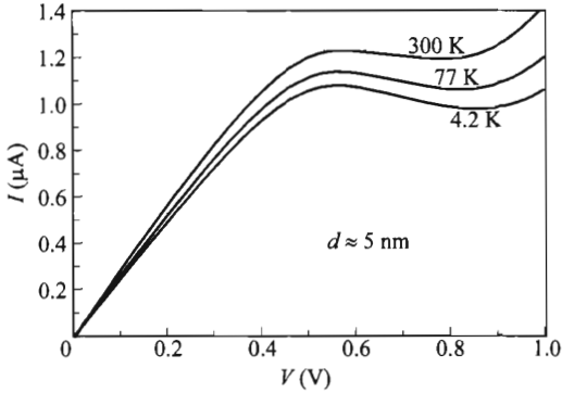
Fig. 24 MIS tunnel diode (Al- \text{Al}_2\text{O}_3 -SnTe) I - V characteristics showing negative resistance. (After Ref. 50.)
