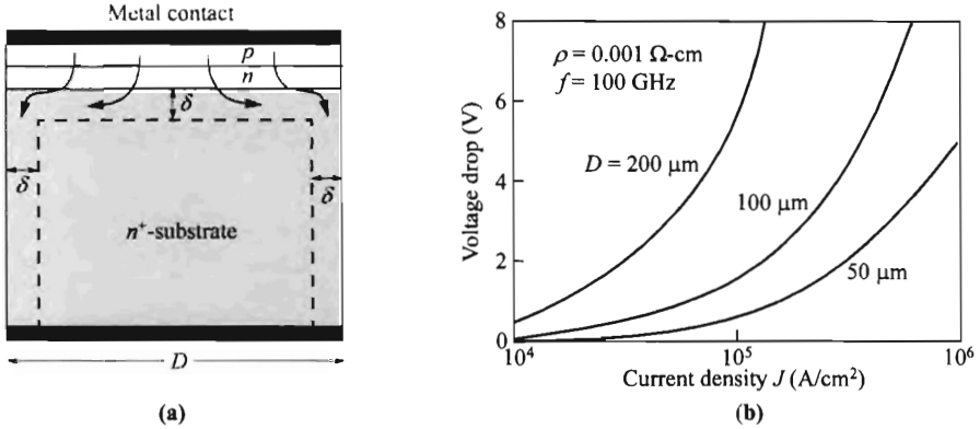
Fig. 12 Skin effect in IMPATT diode. (a) Current flow confined to a surface lamina of thickness \delta , causing nonuniformity and resistive loss. (b) Calculated voltage drop in the substrate at 100 GHz for several diode diameters D . (After Ref. 26.)
