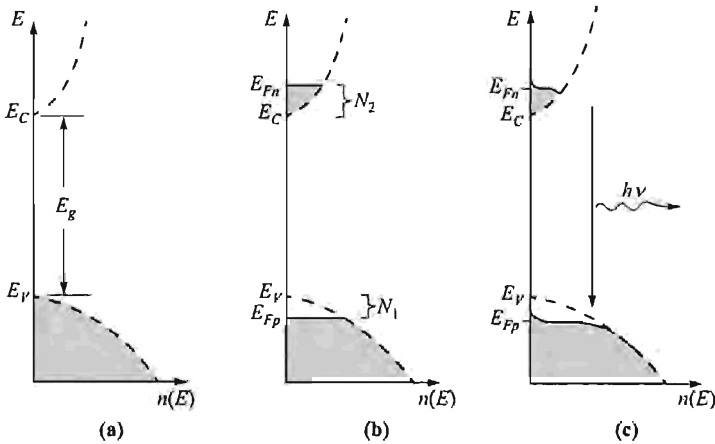
Fig. 17 Electron concentration as a function of energy in a semiconductor, determined by density of states (dashed) and Fermi-Dirac distribution. (a) Equilibrium, T = 0 K. With population inversion, (b) T = 0 K and (c) T > 0 K.
