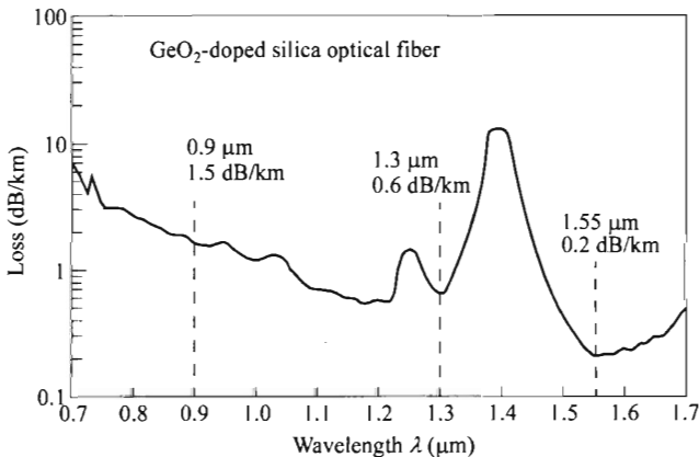
Fig. 23 Loss characteristics of silica optical fiber. The three wavelengths of interest are also shown. (After Ref. 46.)
