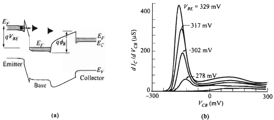
Fig. 31 (a) Energy-band diagram of THETA as a spectrometer. The collector voltage is negative with respect to the base to vary the effective collector barrier height. (b) Hot-electron energy spectrum. (After Ref. 70.)
