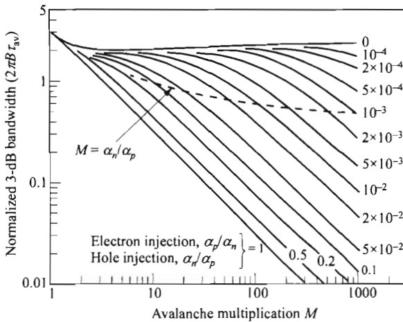
Fig. 12 Theoretical 3-dB bandwidth B (times 2\pi\tau_{av} ) of APD as a function of low-frequency multiplication M , for various values of \alpha_p/\alpha_n for electron injection (or \alpha_n/\alpha_p for hole injection). (After Ref. 19.)
