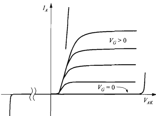
Fig. 28 Output characteristics of an n -channel IGBT.
