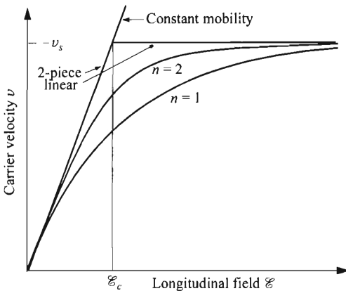
Fig. 11 v - \mathcal{E} relationship (Eq. 33) for n = 1 and 2, and two-piece linear approximation. The critical field \mathcal{E}_c \equiv v_s/\mu , where \mu is low-field mobility, is also indicated.
