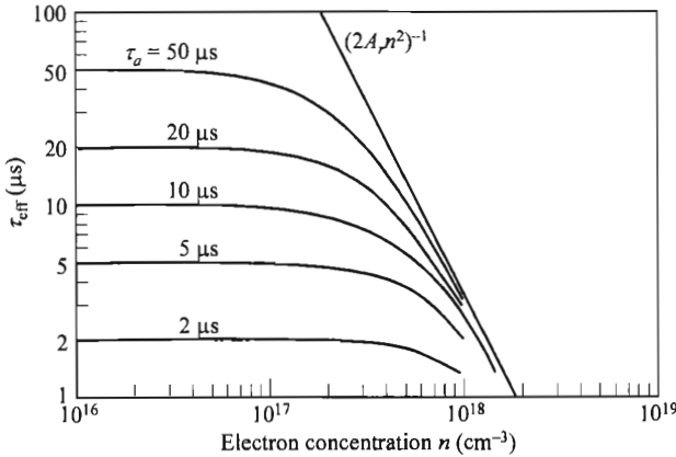
Fig. 13 Effective lifetime under high-injection condition. \tau_a is the ambipolar lifetime and A , is the Auger coefficient ( = 1.45 \times 10^{-31} \text{ cm}^6/\text{s} ). (After Ref. 8.)
