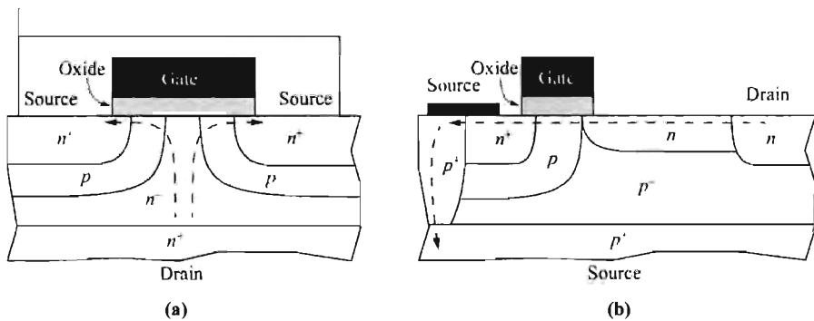
Fig. 39 (a) Vertical DMOS transistor and (b) LDMOS transistor. Current path is indicated by dashed line. In LDMOS transistors, it is common to connect the source to the substrate to reduce inductance of the bonding wire.
