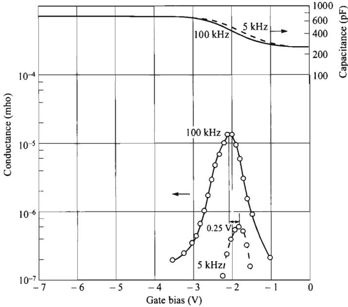
Fig. 16 Comparison of MIS capacitance and conductance measurement at two frequencies, showing that conductance is much more sensitive to frequency than to capacitance. (After Ref. 24.)
