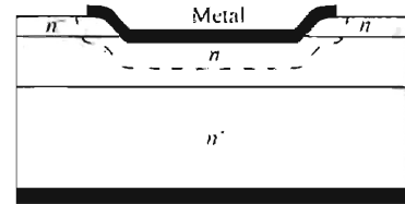
(g) High-resistivity guard layer
