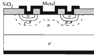
(f) Double-diffused guard ring
