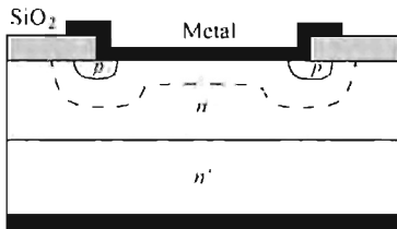
(e) Diffused guard ring
