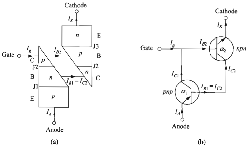
Fig. 8 (a) Two-transistor approximation of a three-terminal thyristor, bisected into (but connected) p-n-p and n-p-n bipolar transistors. (b) Its circuit representation using transistor notations.
