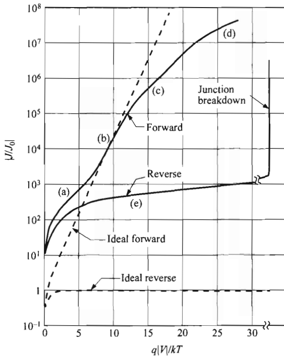
Fig. 11 Current-voltage characteristics of a practical Si diode. (a) Generation-recombination current region. (b) Diffusion-current region. (c) High-injection region. (d) Series-resistance effect. (e) Reverse leakage current due to generation-recombination and surface effects.
