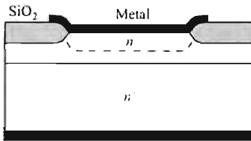
(c) Oxide isolated
