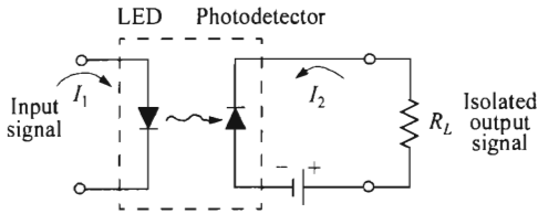
Fig. 8 An opto-isolator provides electrical isolation between input and output.
