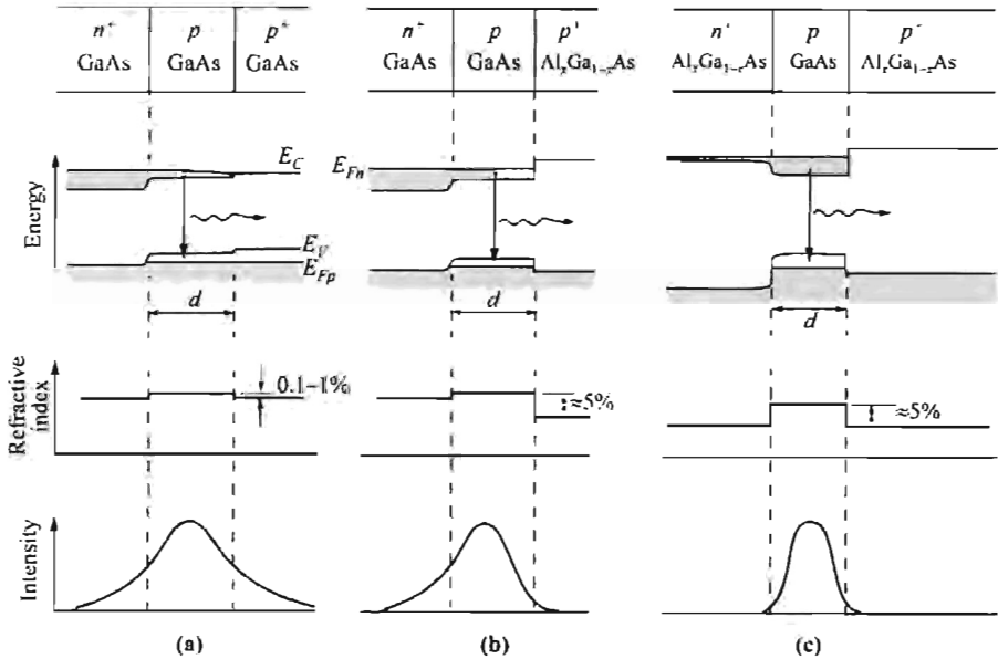
Fig. 25 Comparison of (a) homostructure, (b) single-heterostructure, and (c) double-heterostructure lasers. The top row shows energy-band diagrams under forward bias. n_c change for GaAs/ \text{Al}_x\text{Ga}_{1-x}\text{As} is about 5% while that due to doping is less than 1%. Confinement of light is shown at bottom. (After Ref. 48.)
