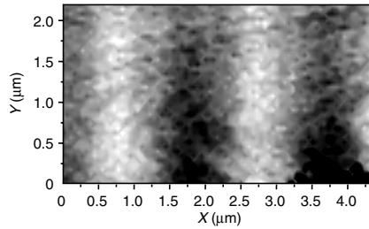
Fig. 5.20. Gray-scale image of optical disk tracking groove; intensity is proportional to profile
