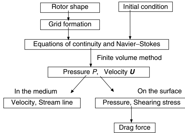
Fig. 4.22. Process for flow field and drag force analyses of optical rotor in water at room temperature by computational fluid dynamics (CFD)
