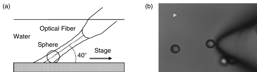
Fig. 3.36. Trapping performance by solitary optical fiber inserted at angle of 40^\circ
