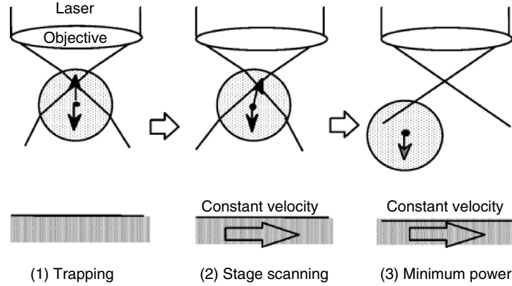
Fig. 3.30. Method of measuring transverse trapping power as minimum power for trapping a particle moving at the constant velocity of v in water
