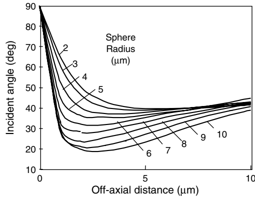
Fig. 3.24. Relationship between optimum fiber incident angle and radius of microsphere for F_{sz} = F_{gz} at maximum F_g on off-axial position
