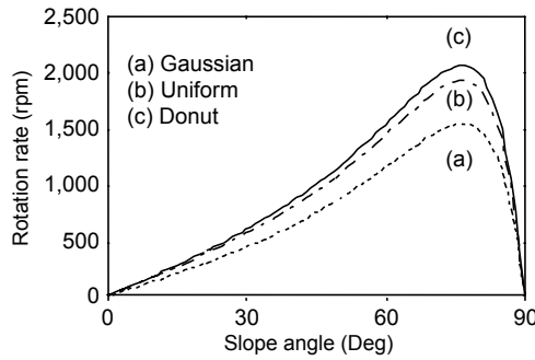
Fig. 4.15. Relationship between rotation rate and slope angle of the rotor of d = 3 \mu\text{m} , h = 10 \mu\text{m} , and n_2 = 1.53 in water at P = 100 \text{ mW} for the Gaussian (a), uniformly filled (b), and donut (c) beam intensity profiles
