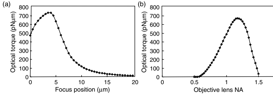
Fig. 4.6. Simulated optical torque dependence on focal position with objective lens \text{NA}=1.2 (a), and dependence on objective lens NA (b) with focus above 5\ \mu\text{m} , for shuttlecock rotor with uniform light beam profile
