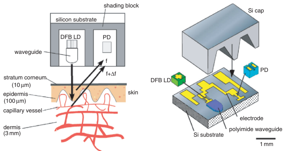
Fig. 1.34. The hybrid integrated structure of the blood flow sensor consists of an InGaAsP-InP distributed feedback laser diode (DFB-LD), a photodiode (PD) and a polyimide waveguide on a silicon (Si) substrate [1.70]. Courtesy of E. Higurashi, NTT, Japan
