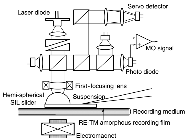
Fig. 5.38. Heat-assisted magnetic recording (HAMR), avoiding superparamagnetic limit of HDD. A SIL has a higher NA [5.39]. Courtesy of H. Sueda, Hitachi, Japan
