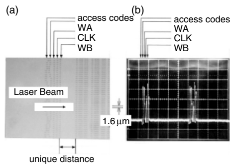
Fig. 2.37. Discrete block format (DBF) marks with a 1.6- \mu\text{m} track-pitch (a), and reproduced signals at 900 rpm. LD bias current is 40 mA (b)
