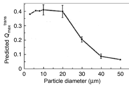
Fig. A.5. Dependence of predicted Q_{\text{max}}^{\text{trans}} on sphere diameter for polystyrene, which is derived from experimental data of Fig. 3.32. Q_{\text{max}}^{\text{trans}} decreases as diameter increases
