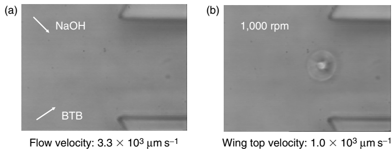
Fig. 4.66. Merging of the flows of NaOH solution ( 4\ \text{mmol/L} ) and BTB solution (a), and optical mixer ( d = 20\ \mu\text{m} ) with the rotation rate of 1,000 rpm at the power of 200 mW (b)
