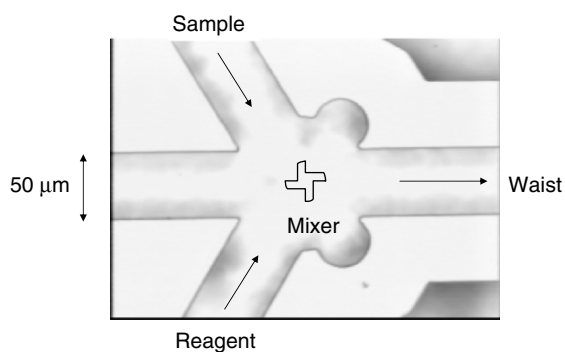
Fig. 4.65. Concept of an optical mixer for use in future \mu -TAS. The integrated system will have components such as inlets, fluidic channels with a mixing chamber, a detector (not shown) and outlets
