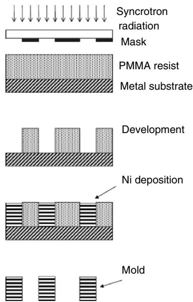
Fig. 1.6. Lithographic galvanoformung abformung (LIGA) involves X-ray lithography and electrodeposition processes
