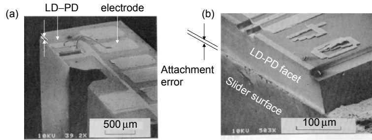
Fig. 2.12. Photograph of the back end of the slider in which an LD-PD chip is bonded to the electrode (a), and the LD-PD facet and the slider surface (b). The attachment error L_{\text{ex}}^1 is less than 1\ \mu\text{m} . Courtesy of H. Nakata, NTT, Japan
