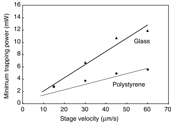
Fig. 3.37. Relationship between minimum trapping power obtained using solitary optical fiber and stage velocity for microspheres of 10 micrometer in diameter
