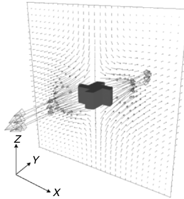
Fig. 4.23. Squint view of velocity vectors in the proximity of optical rotor for 200 rpm
