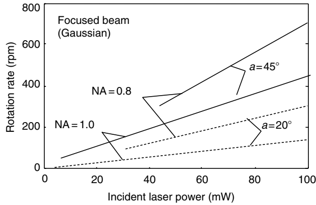
Fig. 4.14. Relationship between rotation rate and laser power for two NAs assuming M_{opt} = M_{drag}(= 4\pi\mu r^2 h\omega)
