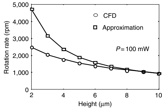
Fig. 4.34. Rotation rate obtained by CFD and approximation with parallel beam illumination at P = 100 \text{ mW} , a = 45^\circ , 2r = 3 \mu\text{m} with rotor height as a parameter
