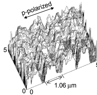
Fig. 5.27. SNOM images (scattered light intensity) of refractive index grating obtained by gold particle probe with p-polarized illumination
