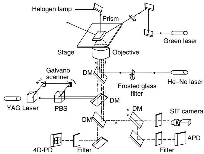
Fig. 3.42. Simultaneous measurement of individual ATPase and mechanical reactions of single myosin molecules. Reprinted from [3.26] with permission by T. Yanagida, Osaka University, Japan
