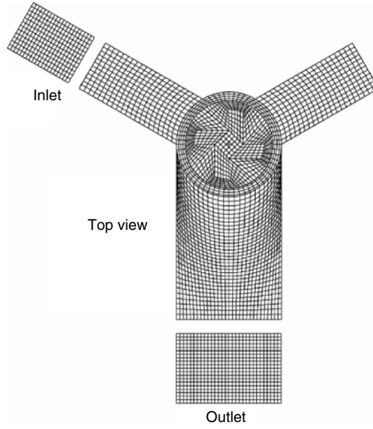
Fig. 4.36. Grid system of Y-shaped microchannel (inlet: 15\ \mu\text{m} width and 20\ \mu\text{m} depth, outlet: 30\ \mu\text{m} width and 20\ \mu\text{m} depth) and optical rotor ( d = 20\ \mu\text{m} , w = 4\ \mu\text{m} , t = 10\ \mu\text{m} ) [4.13]. Courtesy of Y. Ogami, Ritsumeikan University, Japan
