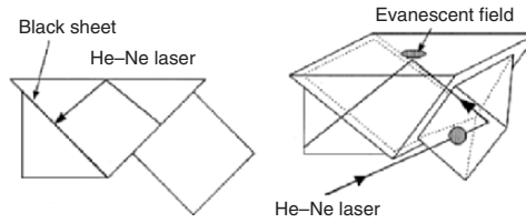
Fig. 5.17. Prism configuration consists of three corner prisms at 45°
