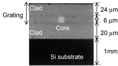
Fig. 5.25. Sectional view of refractive index grating fabricated by UV exposure through phase mask. The grating is formed in a clad layer on a PLC. Courtesy of T. Maruno and Y. Hibino, NTT, Japan
