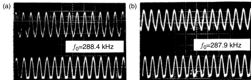
Fig. 2.31. Resonant frequency change of 500 Hz from 288.4 to 287.9 kHz, due to the mass increase of 54 ng for the 1\text{-}\mu\text{m} thick phthalocyanine deposition
