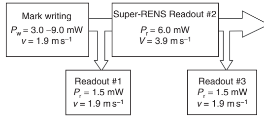
Fig. 5.41. Experimental analysis scheme to determine amorphous levels of both mask and recording layers for super-RENS disk
