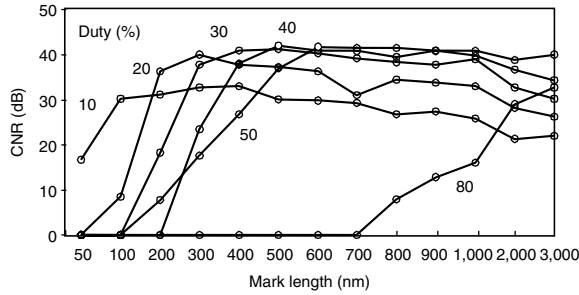
Fig. 5.60. Relationship between CNR and mark length for super-RENS readout ( P_r = 4 mW), with optical pulse duty as parameter
