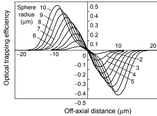
Fig. 3.22. Variation in transverse trapping efficiency at beam waist as function of off-axial distance, with microspore radius as a parameter
