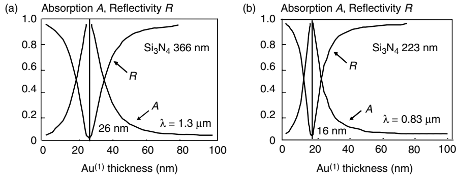
Fig. 2.52. Total absorption A and reflectivity R of Au/Si_3N_4/Au versus the Au thickness at the optimum Si_3N_4 thickness for wavelengths of 1.3 \mu\text{m} (a), and 0.83 \mu\text{m} (b)
