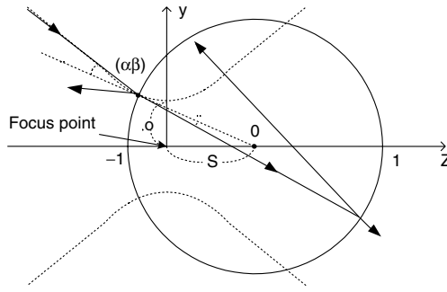
Fig. 3.14. Geometry for calculating exact axial trapping efficiency for microsphere considering beam waist
