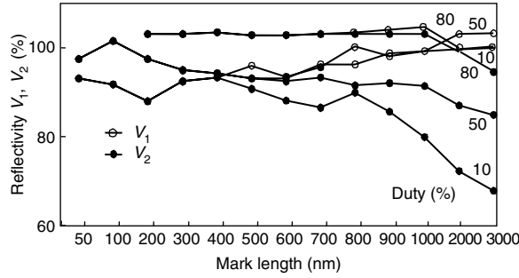
Fig. 5.59. Relationships between reflectivity V_1 (non-mark), V_2 (mark), and mark length for super-RENS readout ( P_r = 4 mW), with optical pulse duty as parameter
