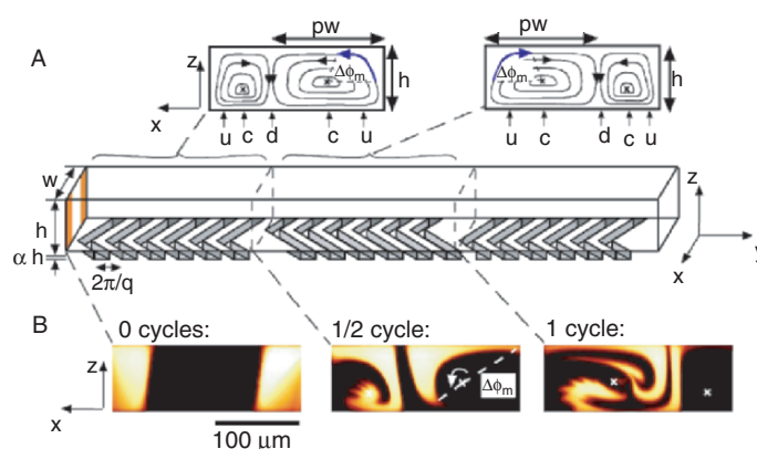
Fig. 4.63. Mixing by intersecting microchannels, which induces chaotic behavior of microflow [4.21]. Courtesy of A. Stroock, Cornell University, USA
