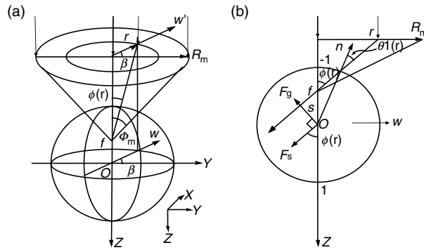
Fig. 3.11. Geometry for calculating axial trapping efficiency of polystyrene microsphere. The laser focus is on the optical axis which is parallel to the center line of the microsphere [3.4]
