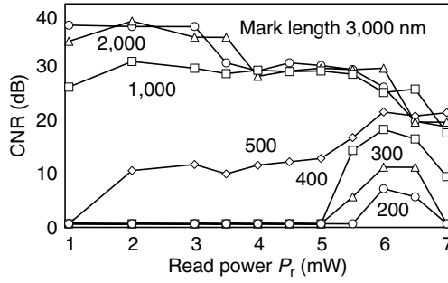
Fig. 5.43. Read power dependence of CNR for various mark lengths written at power of 7.0 mW for medium velocity of 1.9 m s -1
