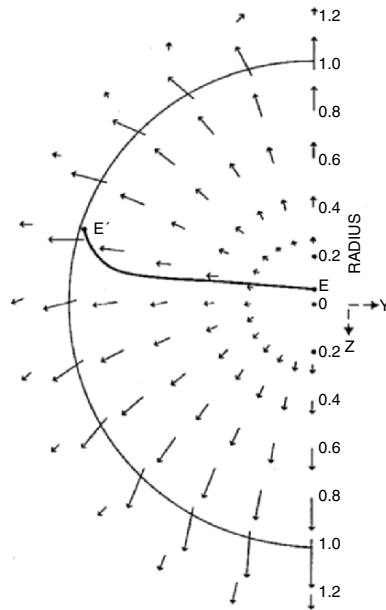
Fig. A.4. Magnitude and direction of total trapping efficiency (optical pressure force) for a microspore of relative refractive index of 1.2 at arbitrary focal position in the yz plane. A circularly polarized laser beam uniformly fills the objective aperture of NA = 1.25 [6.4]
