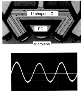
Fig. 1.31. Photograph of the optical encoder. Courtesy of R. Sawada, NTT, Japan
