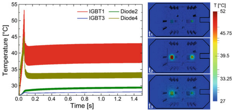
Fig. 5 Temperature as obtained from the ET simulations: waveforms (left), and maps (right)
