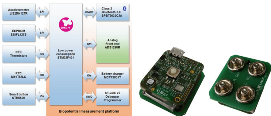
Fig. 1 Block diagram and picture of the proposed wearable system. The electronic system is based on two PCBs, one hosting the main electronics (left) and one exposing the 4 ECG electrodes and the thermistor (right). The battery is located in between the two PCBs
