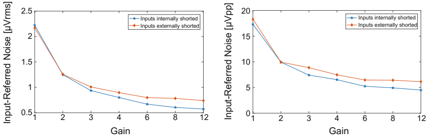
Fig. 2 Input-referred noise
