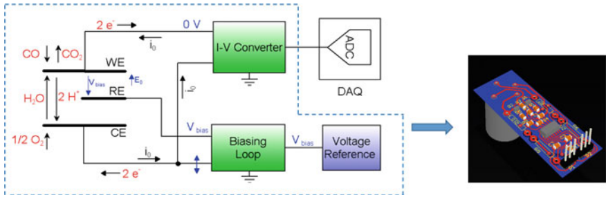
Fig. 2 Electrochemical front end block scheme
