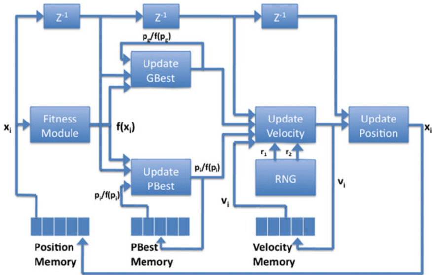
Fig. 2 Implementation of PSO on FPGA
