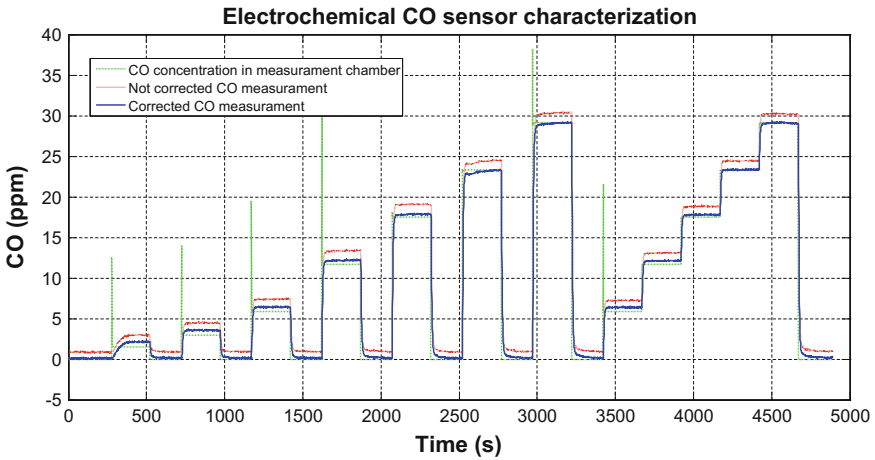
Fig. 4 CO-A4 sensor response to CO mixtures in air (RH=50%, flow rate 200 mL/min). Green: real CO concentration, blue and red: measured CO concentration corrected and not corrected for temperature, respectively
