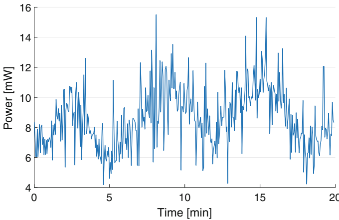
Fig. 6 Output power with 10°C temperature gradient
