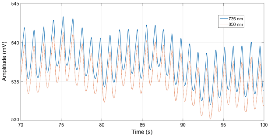
Fig. 4 Raw data waveform extracted from fNIRS system: solid line the measure at 735 nm, dotted line the measure at 850 nm. The AC component is due to heart beat while the DC offset represents the useful hemodynamic signal
