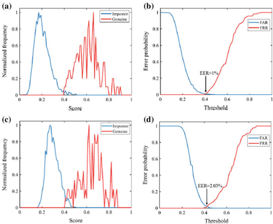
Fig. 4 Experimental impostor and genuine distributions (a) and FAR and FRR versus threshold (b) obtained with proposed procedure. Experimental impostor and genuine distributions (c) and FAR and FRR versus threshold (d) obtained with the procedure derived for wet acquisitions
