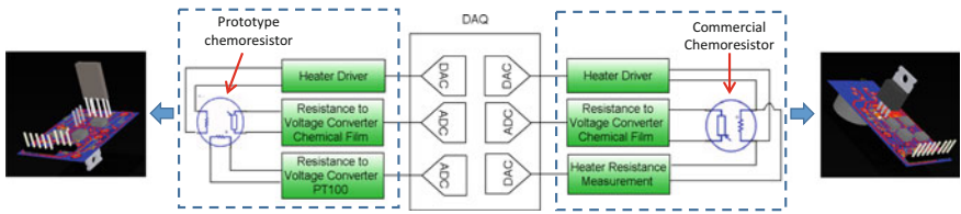
Fig. 3 Front end block diagrams for prototype (left) and commercial (right) chemoresistive sensors
