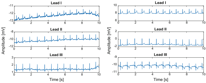
Fig. 3 ECG signal with gel electrodes. Left side: RLD not active. Right side: RLD active
