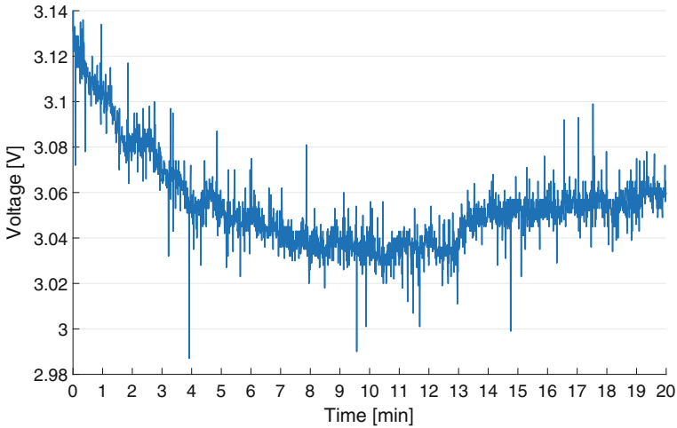
Fig. 8 Super-capacitor voltage trend of the complete system
