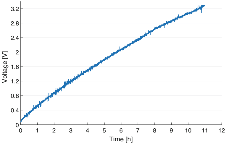
Fig. 9 Super-capacitor charge with the TEG
