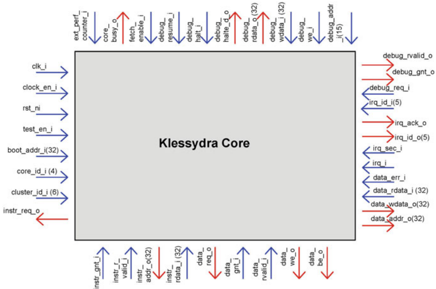
Fig. 2 Klessydra processing core pinout
