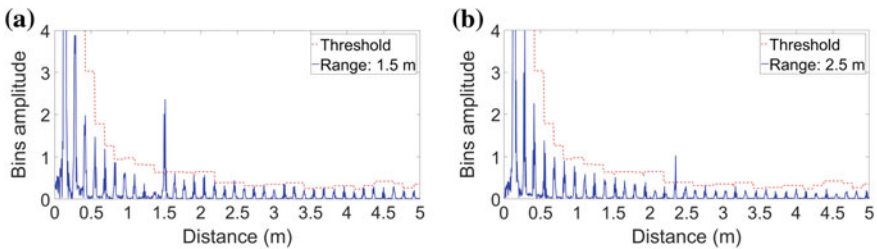
Fig. 3 IF signal (blue line) and threshold (red dashed line) for a target at 1.5 m (a) and 2.5 m (b) (Color figure online)
