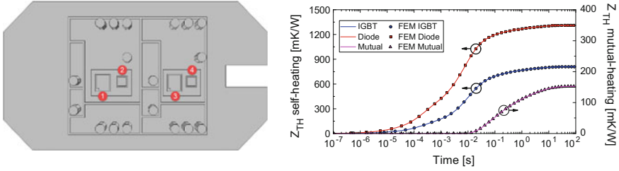
Fig. 2 (Left) Top-view of the FEM model of the commercial power module under test. IGBTs are denoted with #1 and #3, while their respective antiparalleled diodes as #2 and #4. (Right) Self-heating and mutual thermal impedances of an IGBT-diode pair: comparison between COMSOL (symbols) and TFB (solid lines) results
