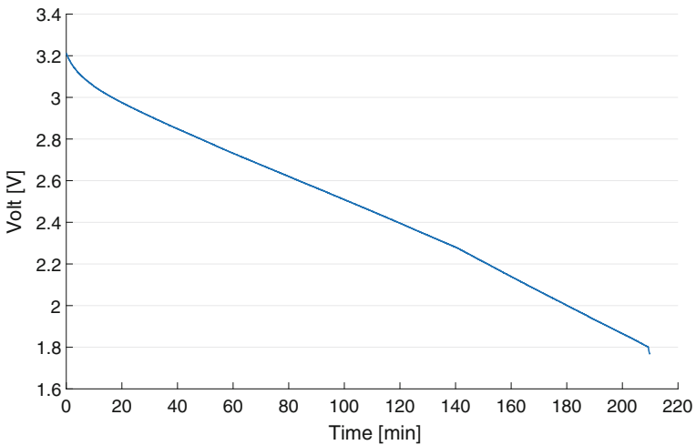
Fig. 10 Autonomy of the system without the TEG and with the super-capacitor fully charged
