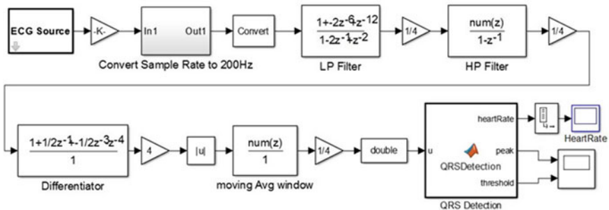
Fig. 3 Simulink fixed point model
