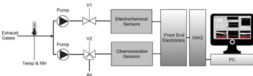
Fig. 1 System structure: the exhaust gases are pumped with a constant flow to sensors through two valves (V1 and V2); temperature and humidity are also measured
