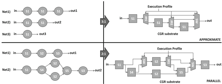
Fig. 1 Dataflow to hardware: Trade-off friendly CGR platforms
