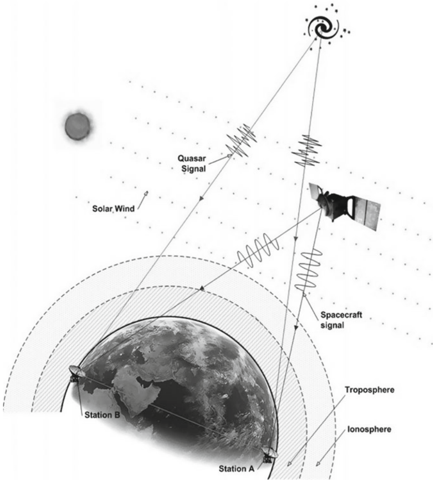
Fig. 1 \Delta DOR geometry
