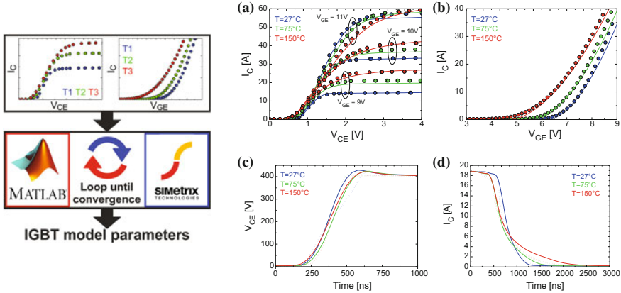
Fig. 3 (Left) Flow chart of the calibration procedure. The input is given by the measured isothermal (pulsed) static (e.g., I_C - V_{CE} , I_C - V_{GE} ) as well as dynamic (e.g., turn-off) characteristics measured at different temperatures. Optimization is performed by grouping parameters in small subsets depending on their impact on the IGBT behavior, and minimizing the error between measurement input and IGBT model output with a MATLAB-SIMETRIX coupling. (Right) a Static output I_C - V_{CE} , b transfer I_C - V_{GE} characteristics, as well as c and d turn-off of the IGBTs at T = 27^\circ C (blue), 75^\circ C (green) and 150^\circ C (red): excellent agreement is obtained between measurements (dots) and calibrated SPICE model (solid lines)
