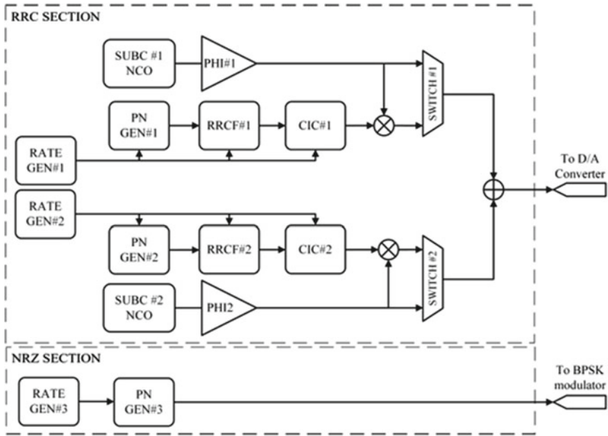
Fig. 2 Wideband \Delta DOR architecture
