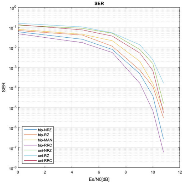
Fig. 4 Symbol error ratio of the system configurations at 10 Gbps, 1 cm distance and 2 dB receiver’s noise figure. As expected the best performance are achieved with bipolar symbols. The RRC and NRZ pulses have the lowest SER as expected from the g(t) pulse
