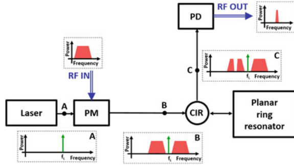
Fig. 1 Block diagram of the coherent microwave photonic band-pass filter. CIR: optical circulator. f_L is the laser frequency
