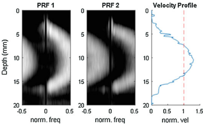
Fig. 3 Left: Aliased profile obtained at PRF1. Center: Aliased profile obtained at PRF2. Right: Reconstructed velocity profile
