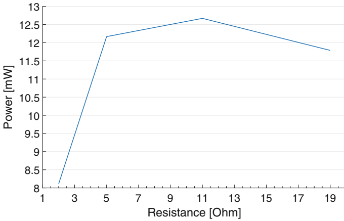
Fig. 5 Power characterization at different load conditions
