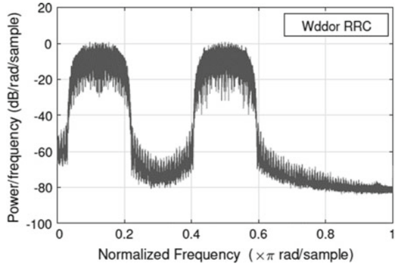
Fig. 4 RRC channels FLP, R_c = F_1/2
