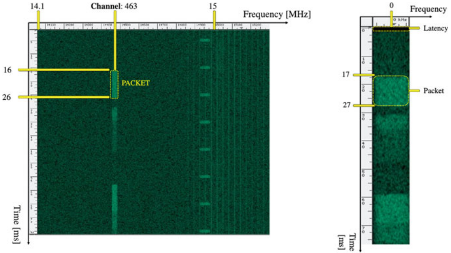
Fig. 3 The spectrogram of the input signal on the left and the spectrogram of an extract channel on the right
