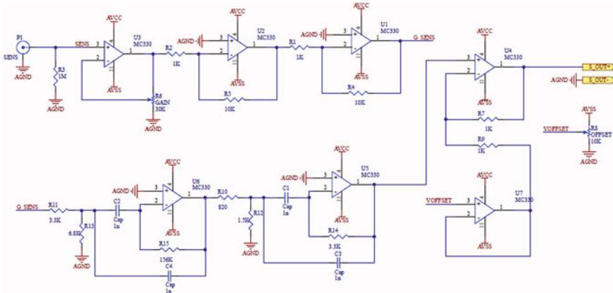
Fig. 4 Analog conditioning circuit
