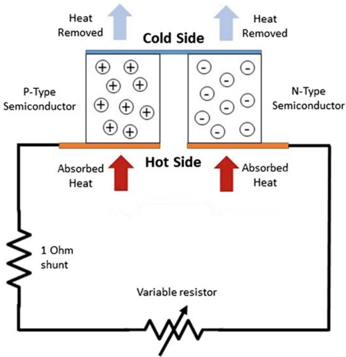
Fig. 3 Working principle of a thermoelectric generator and load setup
