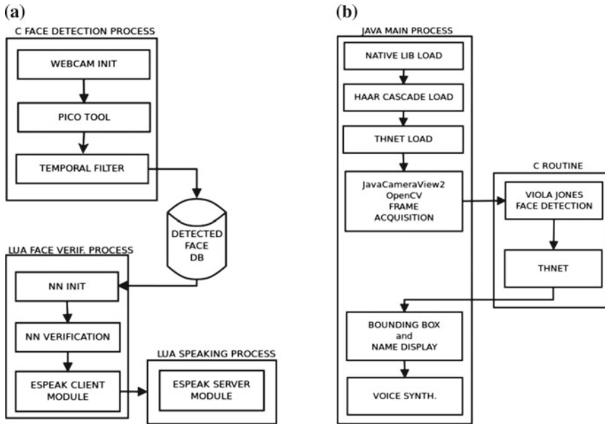
Fig. 1 Processing scheme for the tree prototypes: (a, left) Multiple process face verification system, PC/Odroid prototype; (b, right) Android prototype
