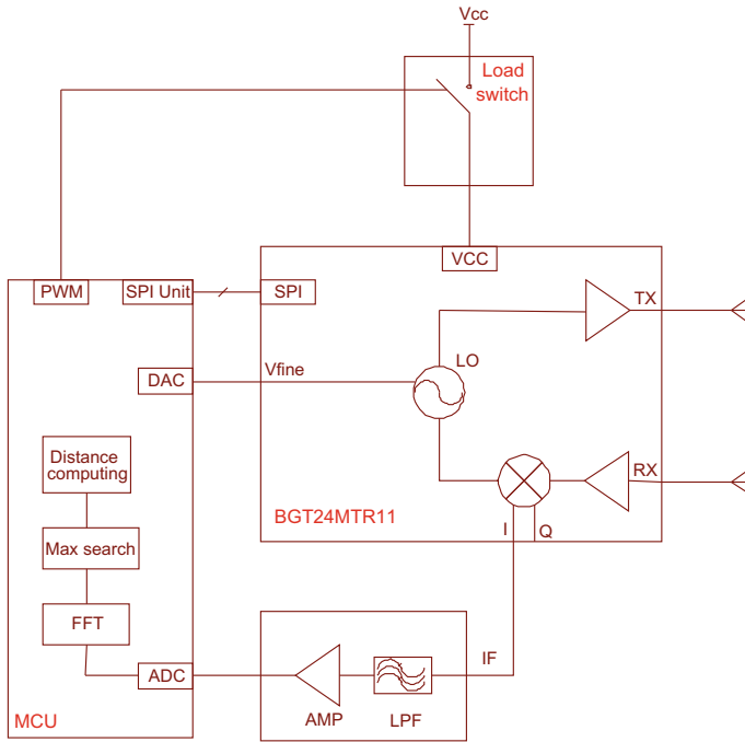
Fig. 1 Adopted radar architecture
