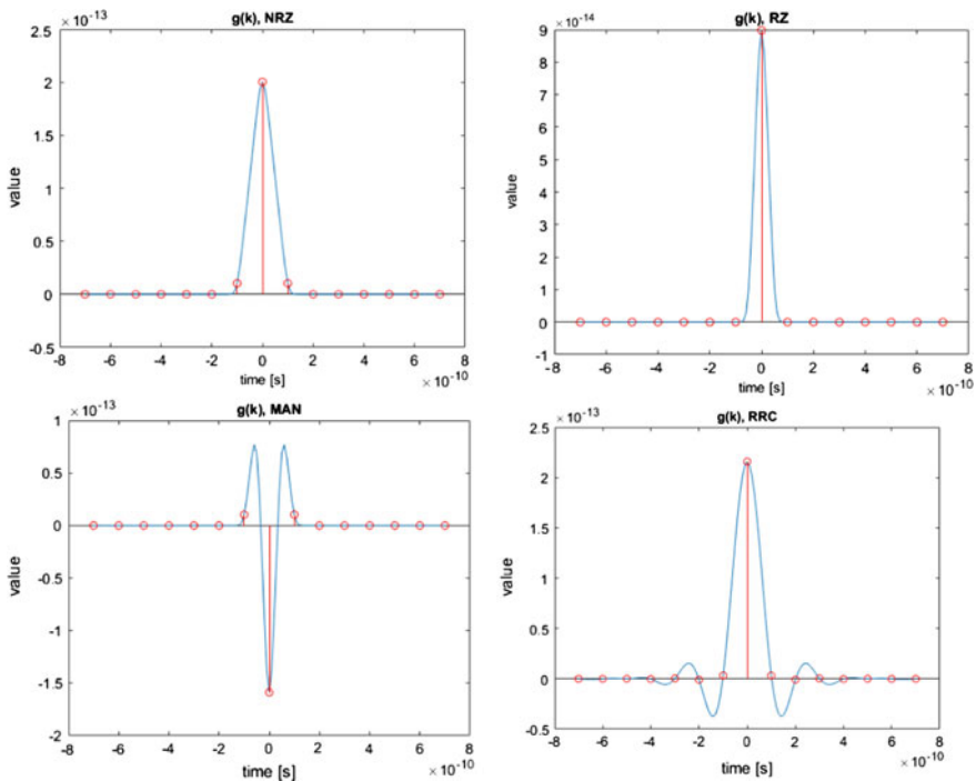
Fig. 3 Plots of g(t) and g(k) for the four pulse shapes taken into account in the paper
