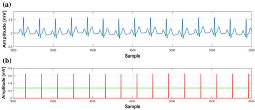
Fig. 2 In a is shown filtered ECG signal. In b are shown in red QRS detected, and in green the detection threshold
