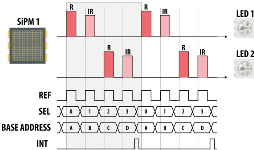
Fig. 3 Temporal diagram of the time-sharing scheme and an excerpt of related control signals
