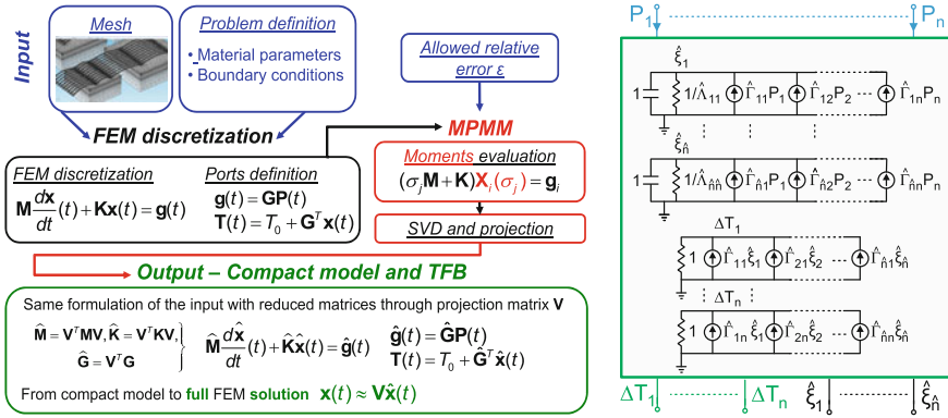
Fig. 1 Proposed TFB extraction procedure (left) and topology (right)
