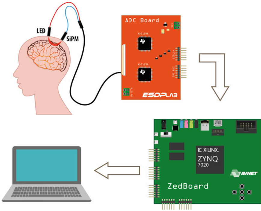
Fig. 1 Block diagram of the developed fNIRS acquisition system
