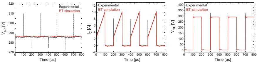
Fig. 4 ET (solid) versus measurement data (dots) for the boost steady-state behavior
