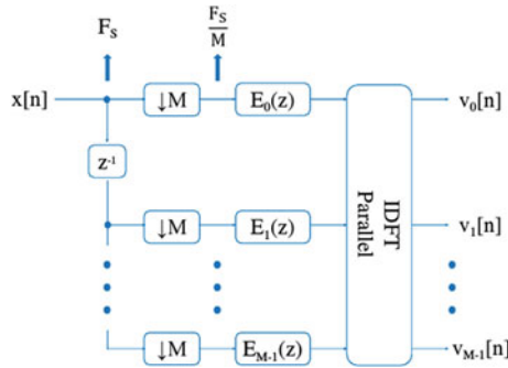
Fig. 1 Multistage implementation of digital filter bank
