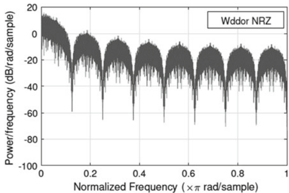
Fig. 3 NRZ channel FLP, R_c = F_1/2
