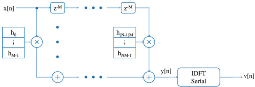
Fig. 2 Serial implementation of digital filter bank
