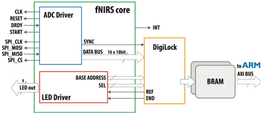
Fig. 2 Block diagram of the VHDL entities in the FPGA
