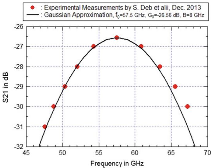
Fig. 2 Approximation of the antenna gain with a Gaussian gain shape
