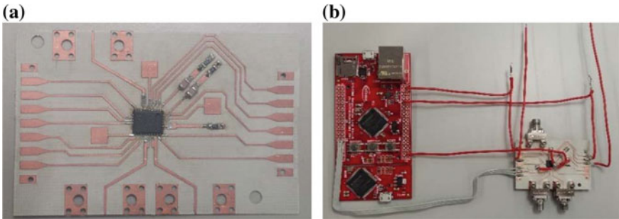
Fig. 2 Detailed pictures of the homemade board, alone (a) and with the XMC4500 development board (b)
