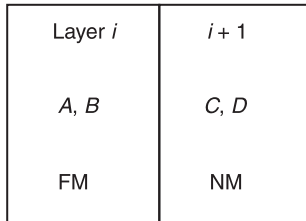
5.8 Two-layer schematic illustration of a typical multilayer spin valve comprising a core ferromagnetic–non-magnetic–ferromagnetic part. Notations A, B, C, D are spin accumulation amplitude at the different layers.
