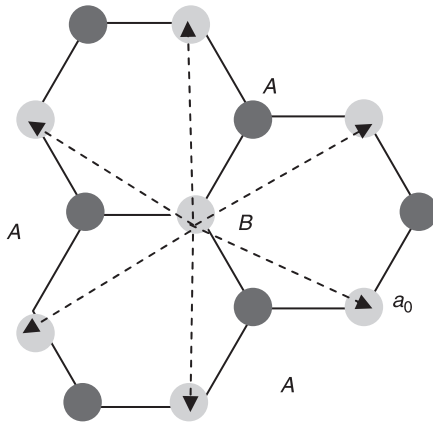
6.2 Nearest and second nearest neighbors in the graphene honeycomb lattice.
