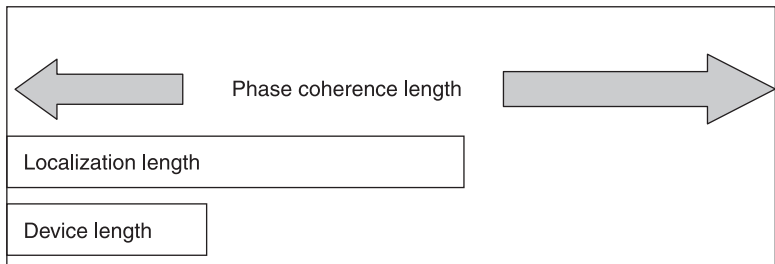
2.19 Illustration of localization effect occurring in a device with length scale in the above context.
