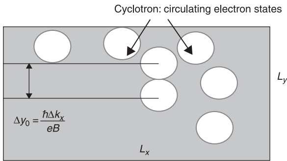
4.3 Physical imagination of electron bound states (cyclotron states) and their distribution in a two-dimensional system based on the Landau gauge under a strong magnetic field.
