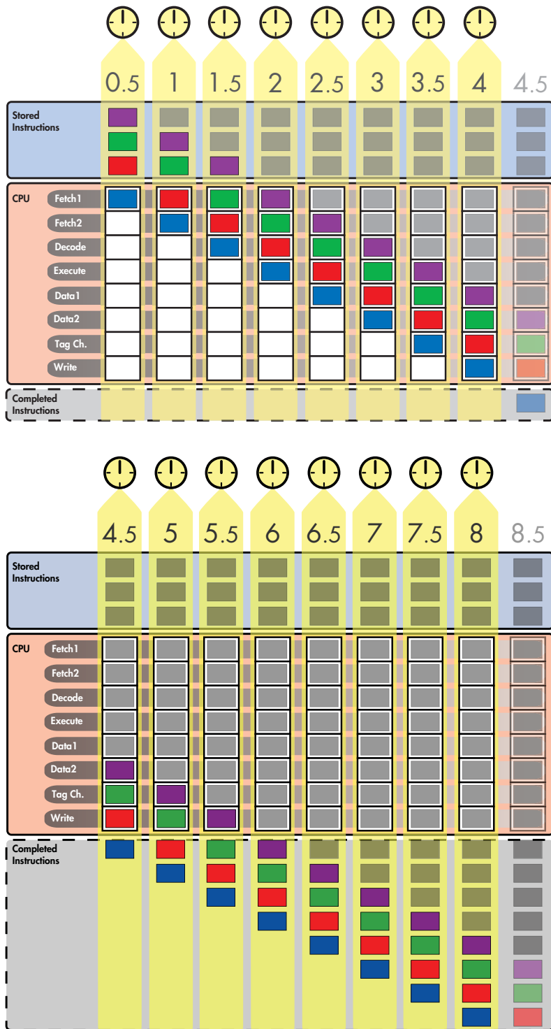
Figure 3-8: An eight-stage pipeline
