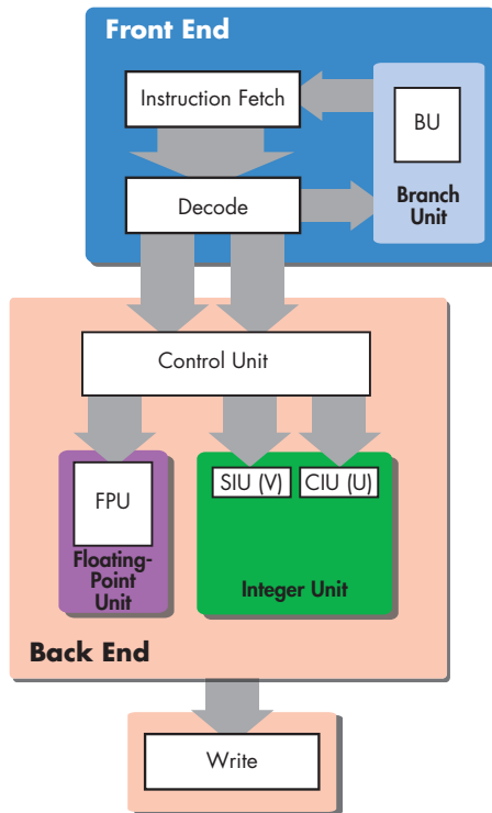
Figure 4-5: The Intel Pentium
