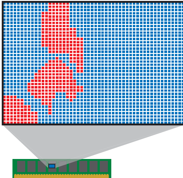
Figure 11-4: Spatial locality
