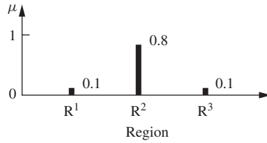
FIGURE 6.10 Membership function for data point (X_1, X_2 = (0.5, 0.5)) .
