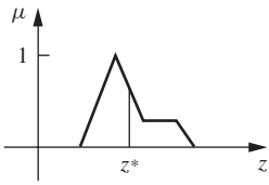
FIGURE 4.13 Centroid defuzzification method.
