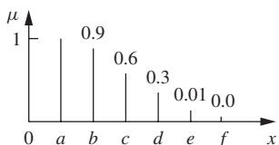
FIGURE 4.8 A discrete fuzzy set \underline{A} .
