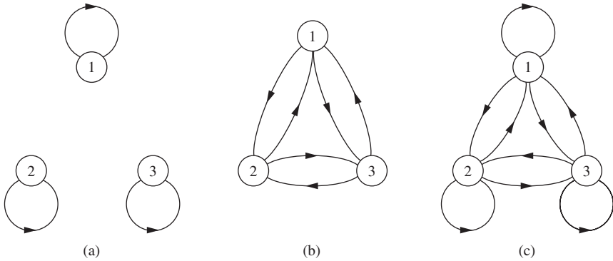
FIGURE 3.8 Three-vertex graphs for properties of (a) reflexivity, (b) symmetry, and (c) transitivity (Gill, 1976).
