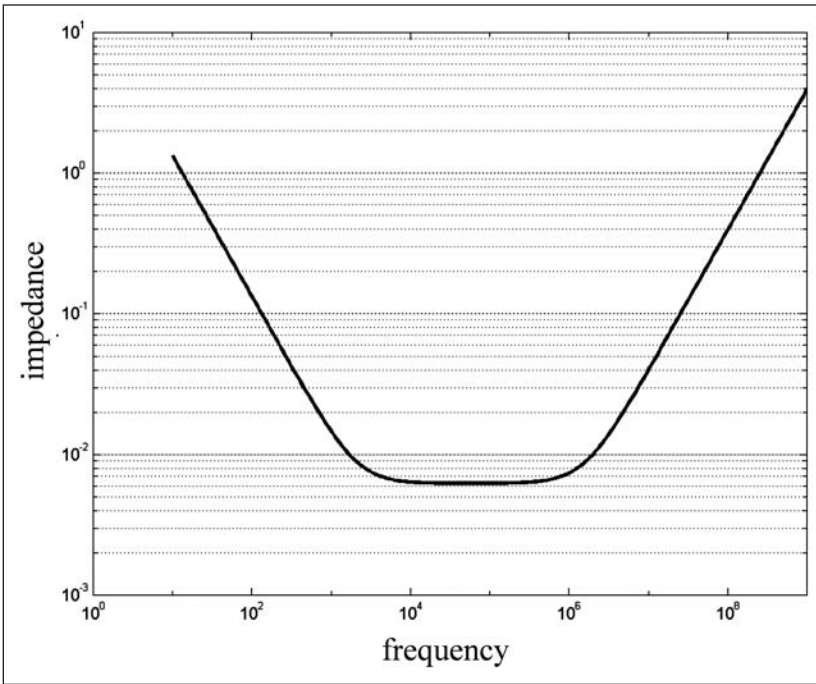
Figure 12.12 Frequency domain impedance of eight 1500μF capacitors.
