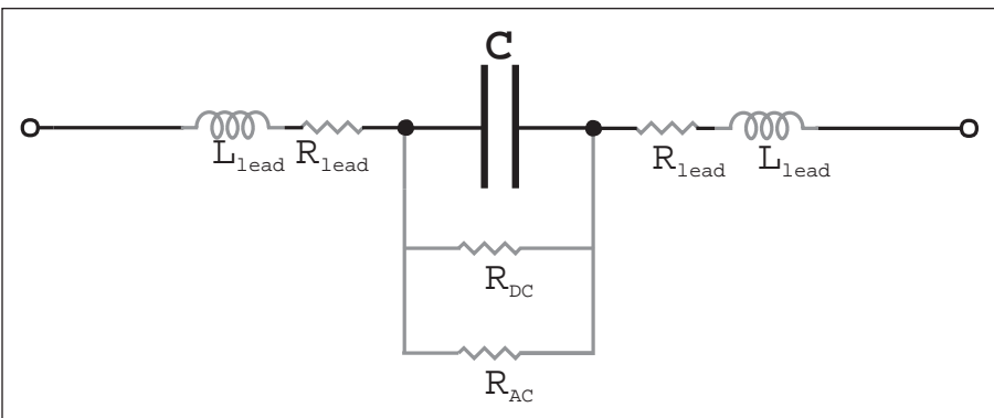
Figure 7.3 The hidden schematic of a real-world capacitor includes lead inductance ( L_{lead} ), lead resistance ( R_{lead} ), dielectric leakage ( R_{DC} ), and dielectric “frictional” loss ( R_{AC} ). The resistances are often combined and called Equivalent Series Resistance (ESR). Dielectric losses (and hence ESR) are typically frequency dependent.
