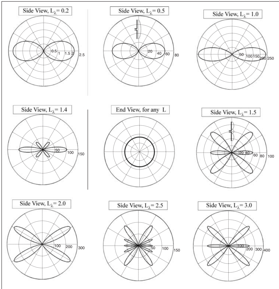
Figure 11.7 Radiation patterns for electric dipoles of various electrical lengths. In each case, the antenna is driven with 1 A. The current on the antenna is shown for lengths of 1/2 and 3/2. The center plot shows the end-view pattern for all lengths.
