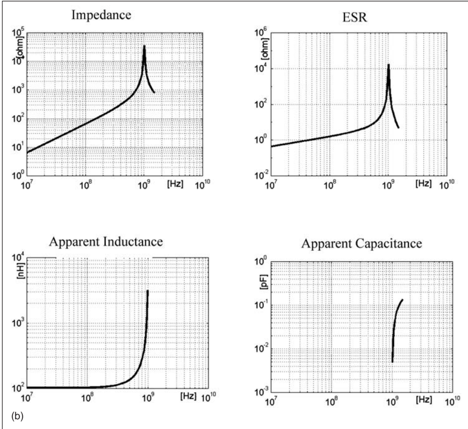
Figure 7.6 B) Frequency response of an air-core, 100nH surface-mount inductor ( C_p = 0.25\text{ pF} ; R_{DC} = 0.38\text{ ohm} ). The self-resonant frequency occurs at about 1 GHz. Above the self-resonant frequency, the device approaches the behavior of a \sim 0.25\text{ pF} capacitor.
