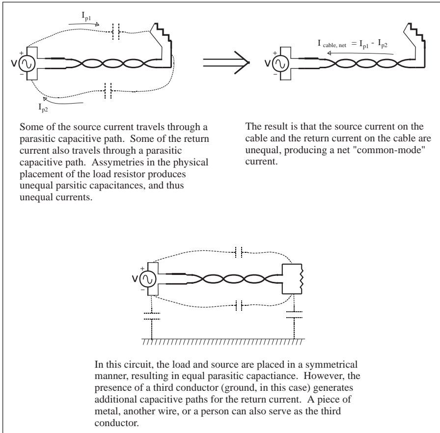
Figure 12.23 Common mode currents arise due to asymmetries in circuits. The circuit asymmetries give rise to asymmetric parasitic paths, leaving a net current on the cable. The net common mode current acts as an efficient antenna.
