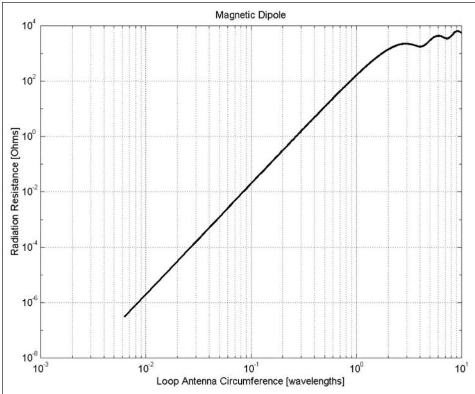
Figure 11.4 Radiation resistance versus magnetic dipole circumference. Below a wavelength, the radiation resistance is proportional to C_\lambda^4 . Power radiated can be determined using P = I \times R_{rad} . This plot assumes a constant current around the loop, and loses accuracy above a half wavelength. However, the general behavior of large loop antennas is similar.
