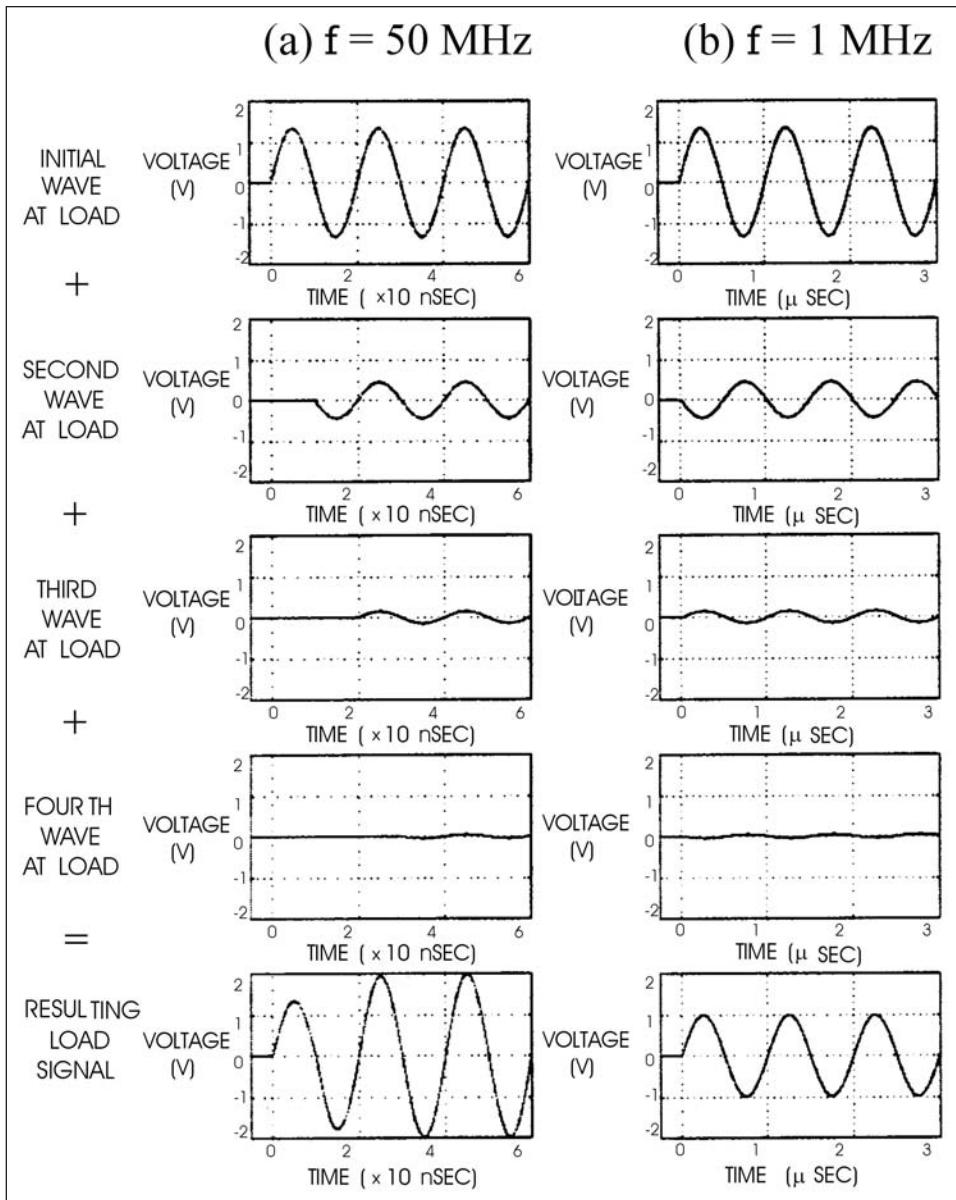
Figure 8.9 This figure illustrates the dependence of transmission line side-effects on signal frequency. In each case, a 1V sine wave signal is applied to the circuit of Figure 8.6. The reflections are of the same amplitude in each case, but the resulting load signals are quite different. Notice the relative phase between the reflections and the original signal in each case.
