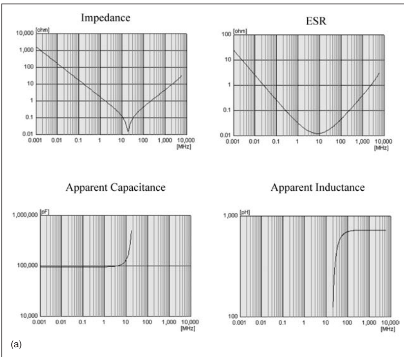
Figure 7.4 A) Frequency response of a 0.1 \mu\text{F} surface-mount, size 0805 (0.08" \times 0.05") capacitor ( L_{lead} = 0.73 \text{ nH} ). B) Frequency response of a 0.015 \mu\text{F} surface-mount, size 0805 (0.08" \times 0.05") capacitor ( L_{lead} = 0.88 \text{ nH} ). Above the self-resonant frequency (SRF) of \sim 40 \text{ MHz} , the device acts like a 0.88 nH inductor. C) Frequency response of a 0.001 \mu\text{F} surface-mount, size 0805 (0.08" \times 0.05") capacitor ( L_{lead} = 0.77 \text{ nH} ). Above the self-resonant frequency (SRF) of \sim 200 \text{ MHz} , the device acts like a 0.77 nH inductor. Plots were created with muRata's MCSIL software ( http://www.murata.com/ ).
