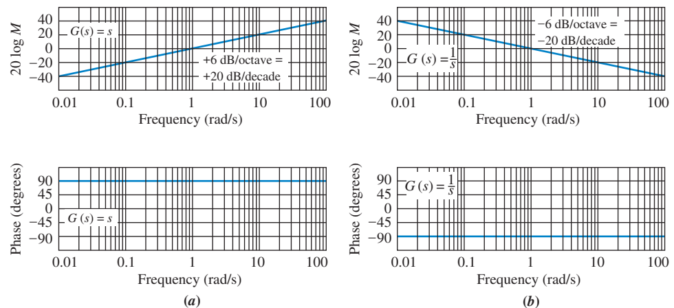
FIGURE 10.9 Normalized and scaled Bode plots for a. G(s) = s ; b. G(s) = 1/s ; (figure continues)
