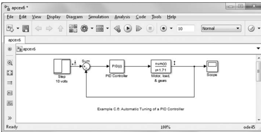
FIGURE C.23 Simulink block diagram showing closed-loop input and output points
