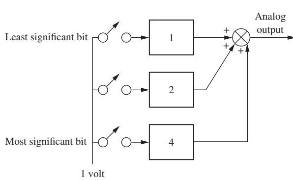
FIGURE 13.3 Digital-to-analog converter
