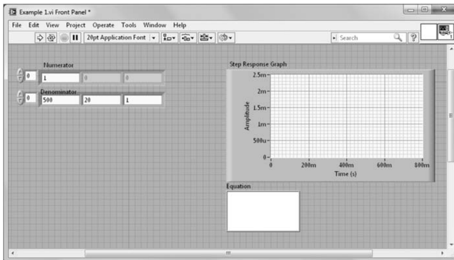
FIGURE D.8 Front Panel: a. for Block Diagram shown in Figure D.7(a); (figure continues)
