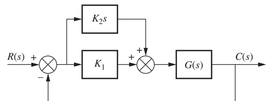
FIGURE 9.23 PD controller
