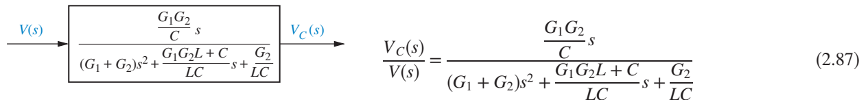
FIGURE 2.7 Block diagram of the network of Figure 2.6
