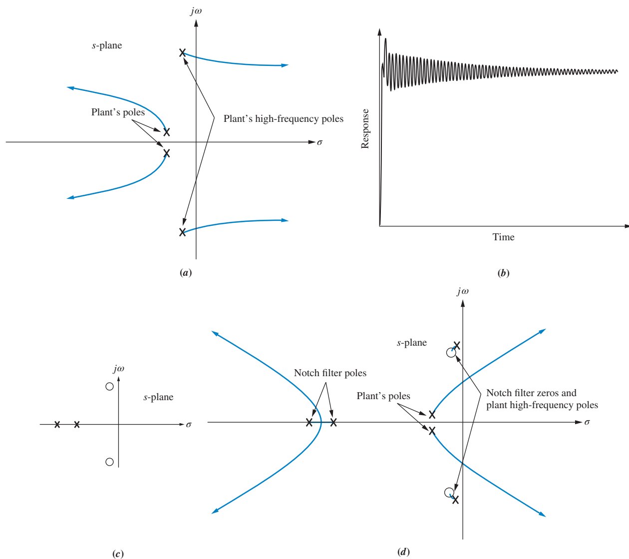
FIGURE 9.44 a. Root locus before cascading notch filter; b. typical closed-loop step response before cascading notch filter; c. pole-zero plot of a notch filter; d. root locus after cascading notch filter; (figure continues)
