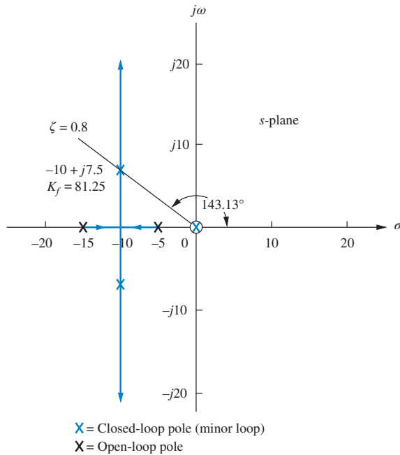
FIGURE 9.56 Root locus for minor loop of Example 9.8
