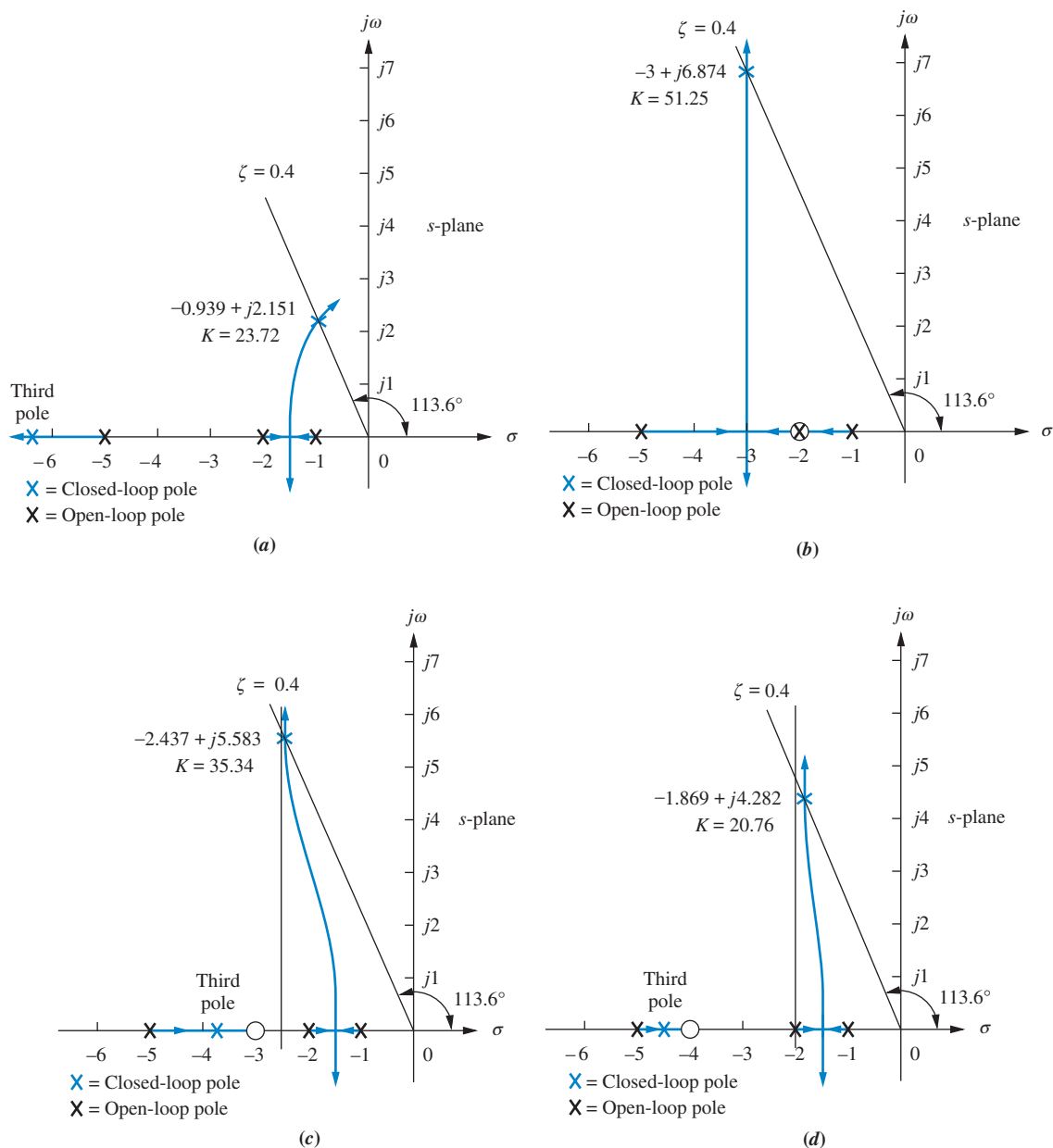
FIGURE 9.15 Using ideal derivative compensation: a. uncompensated; b. compensator zero at -2 ; c. compensator zero at -3 ; d. compensator zero at -4
