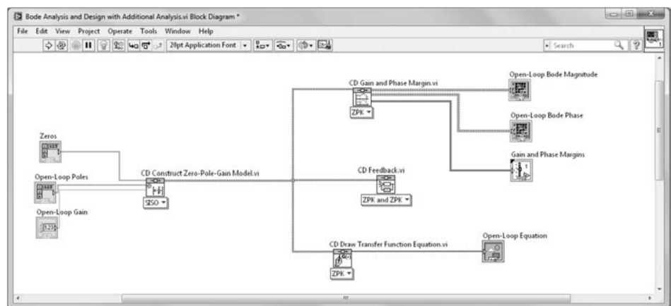
FIGURE D.17 Bode analysis with gain and phase margin: a. Block Diagram; (figure continues)
