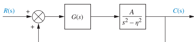
FIGURE P8.13 Linearized magnetic levitation system block diagram
