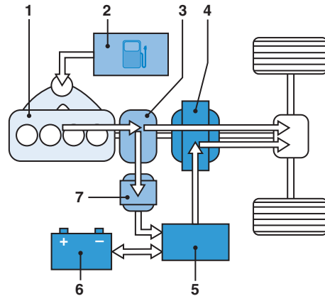
FIGURE P1.10 Split-power hybrid electric vehicle 11
