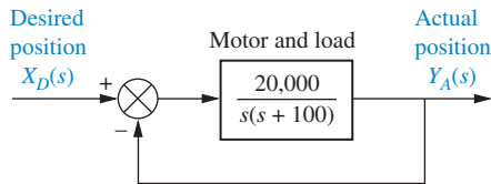
FIGURE P13.9 Simplified block diagram of a floppy disk drive
