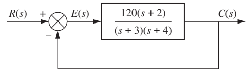
FIGURE 7.5 Feedback control system for Example 7.2
