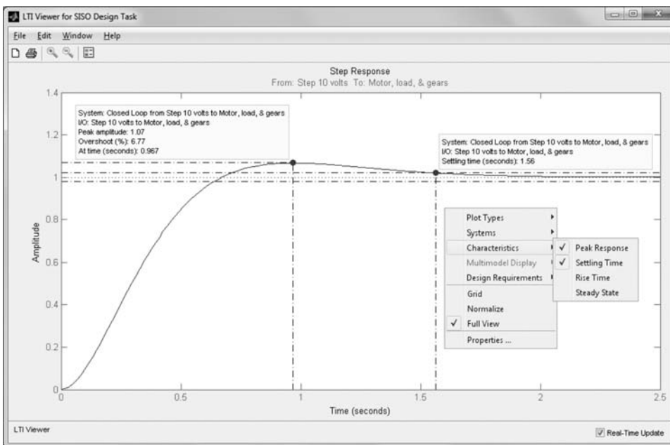
FIGURE C.26 LTI Viewer for SISO Design Task window showing closed-loop step response after automatic PID tuning
