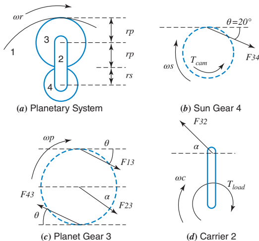
FIGURE P4.17 Free-body diagrams of planetary gear system components 12
