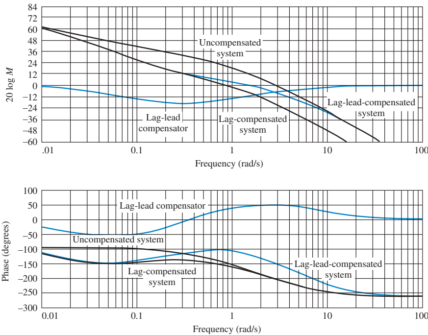
FIGURE 11.12 Bode plots for lag-lead compensation in Example 11.4
