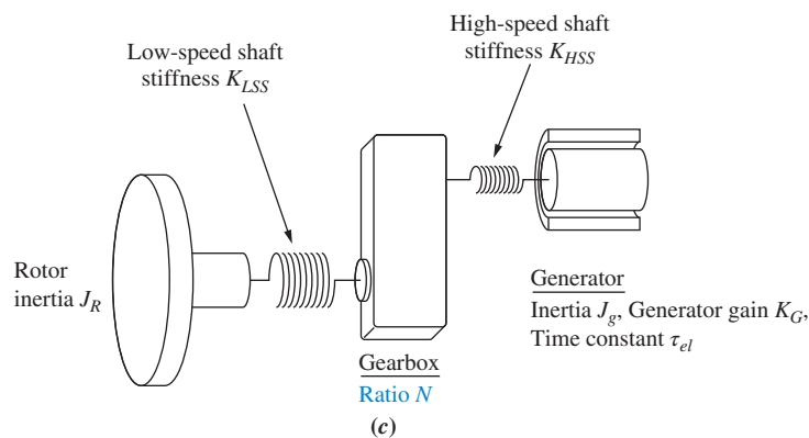
FIGURE P8.17 a. Wind turbines generating electricity near Palm Springs, California; b. control loop for a constant-speed pitch-controlled wind turbine; 5 c. drivetrain 5
