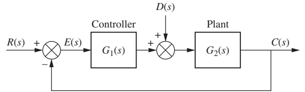
FIGURE 7.11 Feedback control system showing disturbance
