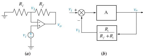
FIGURE P5.33 a. Noninverting amplifier; b. block diagram
