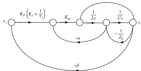
FIGURE P7.22 DVR Model
