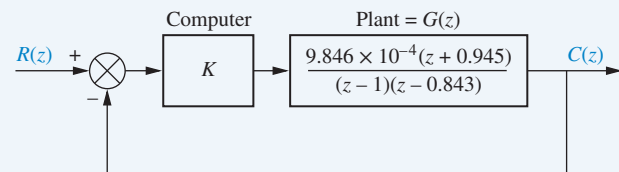
FIGURE 13.31 Analog antenna azimuth position control system converted to a digital system
