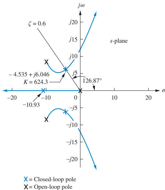
FIGURE 9.57 Root locus for closed-loop system of Example 9.8
