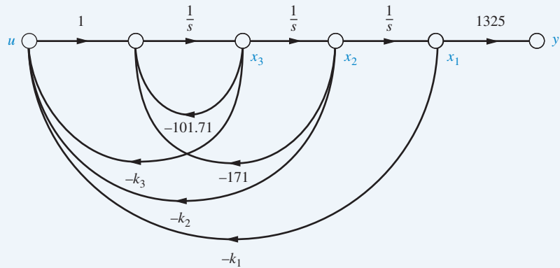
FIGURE 12.25 Plant with state-variable feedback for controller design
