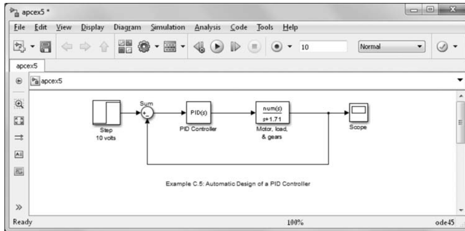
FIGURE C.19 Simulink block diagram for automated design of a PID controller
