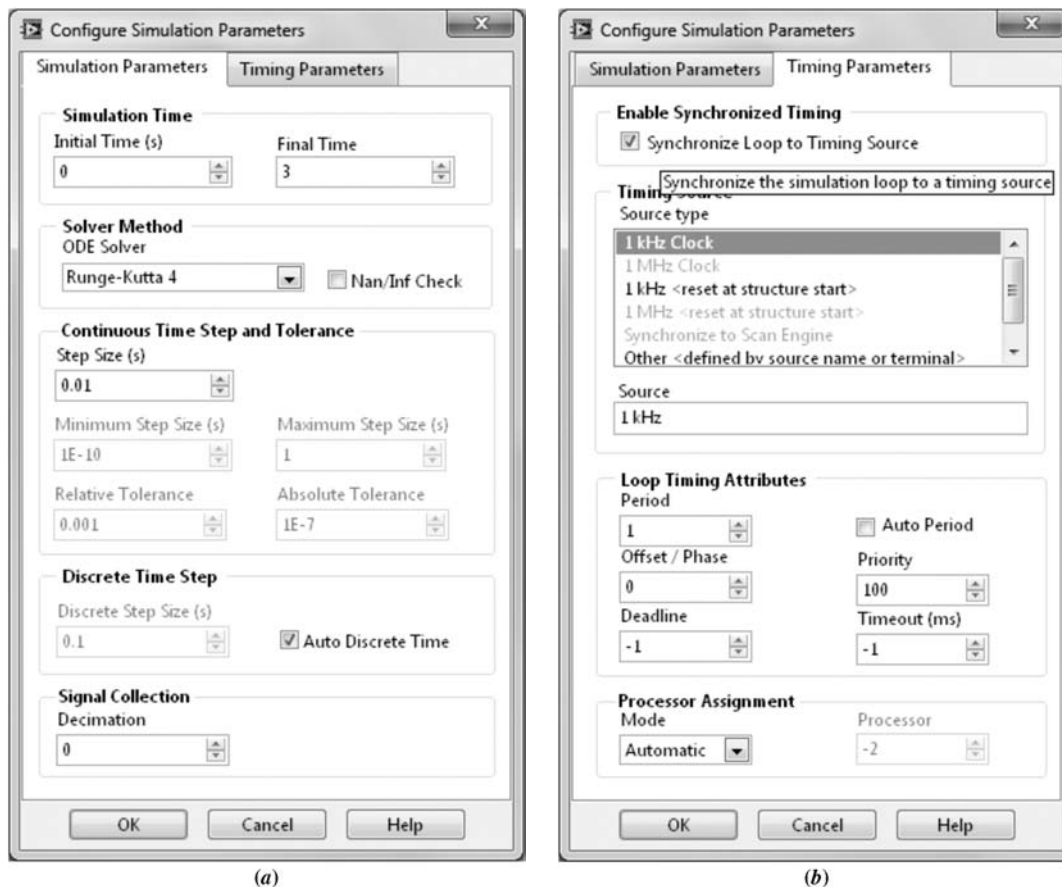
FIGURE D.19 Configuring the Simulation Loop parameters: a. Simulation parameters; b. Timing parameters
