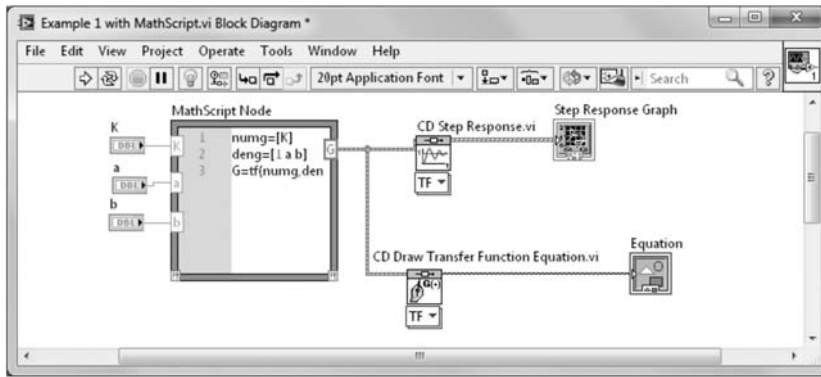
FIGURE D.7 (Continued) b. with MathScript block
