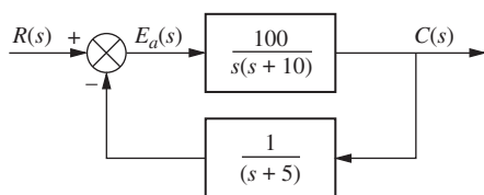
FIGURE 7.16 Nonunity feedback control system for Example 7.8
