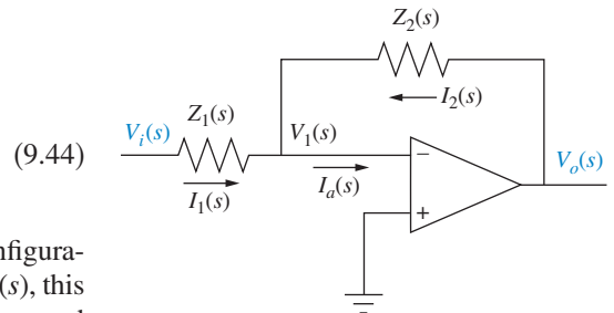
FIGURE 9.60 Operational amplifier configured for transfer function realization
