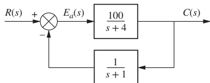
FIGURE 7.18 Nonunity feedback system for Skill-Assessment Exercise 7.5
