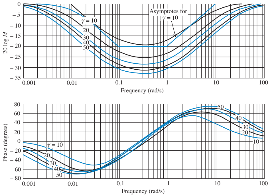
FIGURE 11.11 Sample frequency response curves for a lag-lead compensator,
