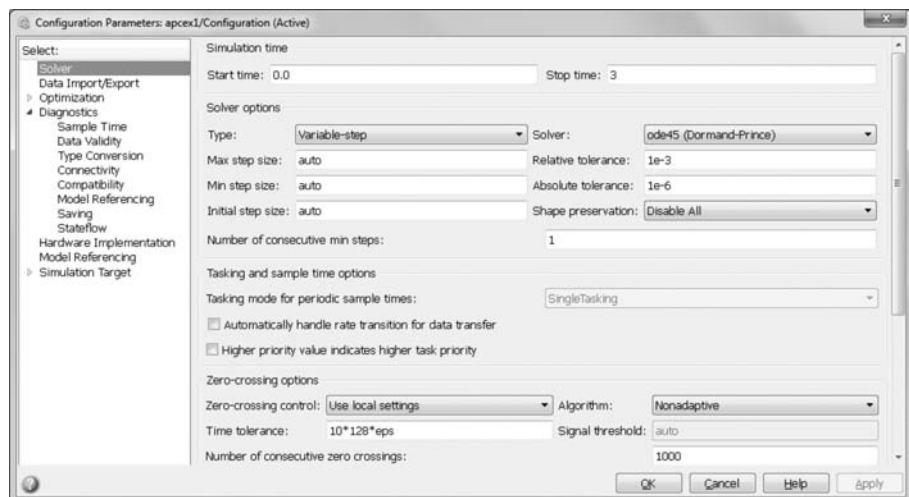
FIGURE C.8 Configuration Parameters window for Solver tab
