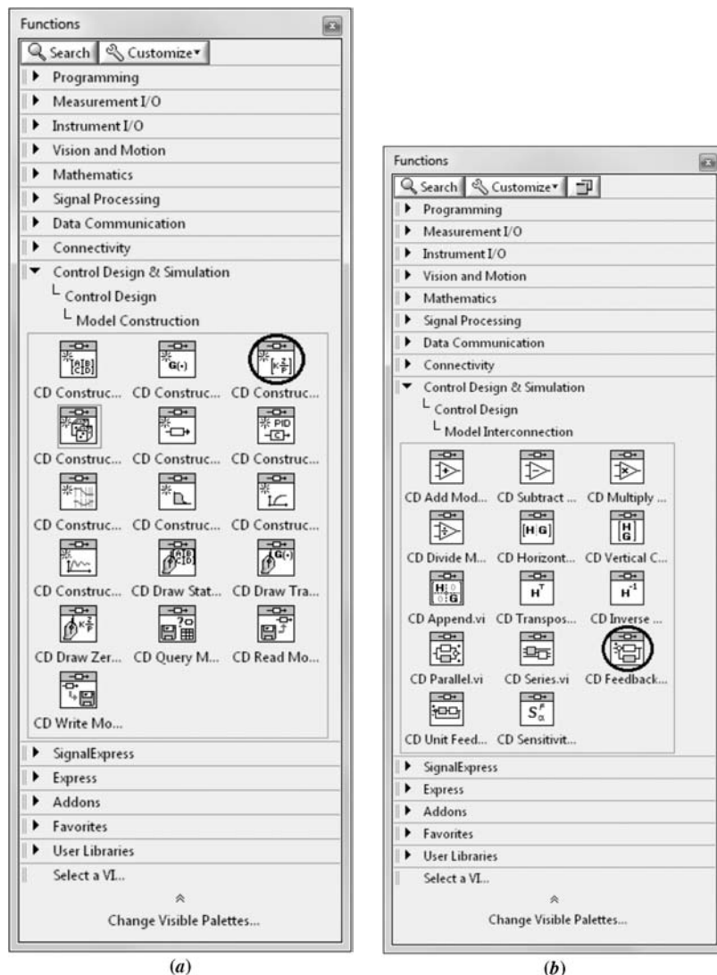
FIGURE D.11 a. Obtaining zero-pole-gain transfer function from the Functions palette; b. Obtaining Feedback interconnection from Functions palette
