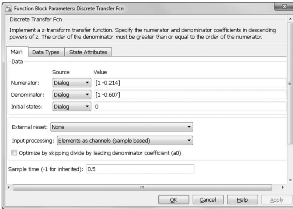
FIGURE C.17 (Continued) b. Discrete Transfer Fcn block
