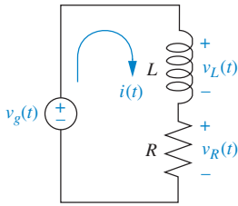
FIGURE P5.32 Solenoid coil circuit
