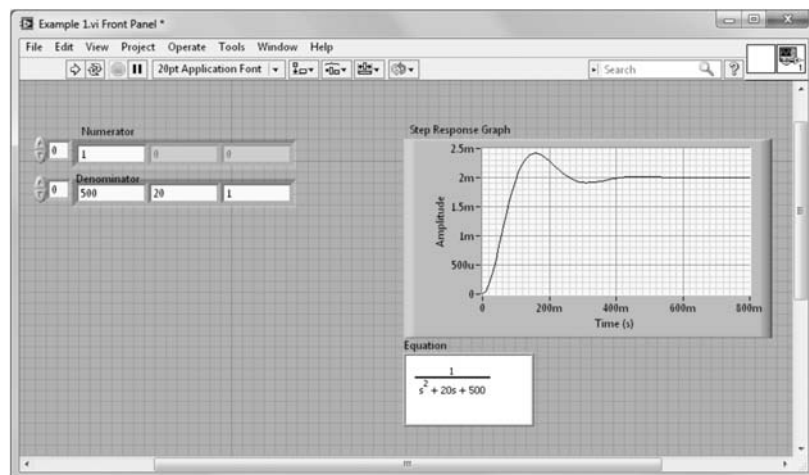
FIGURE D.9 Front Panel after execution: a. for block diagram in Figure D.7(a); (figure continues)
