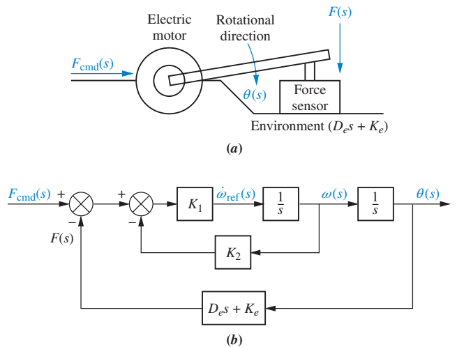
FIGURE P7.30 a. Force control mechanical loop under contact motion; 10 b. block diagram 10
