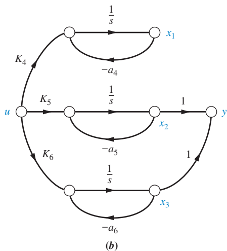
FIGURE 12.15 Comparison of a. observable, and b. unobservable systems
