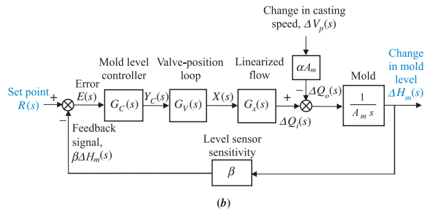
FIGURE P5.41 Steel mold process: a. process; 7 b. block diagram
