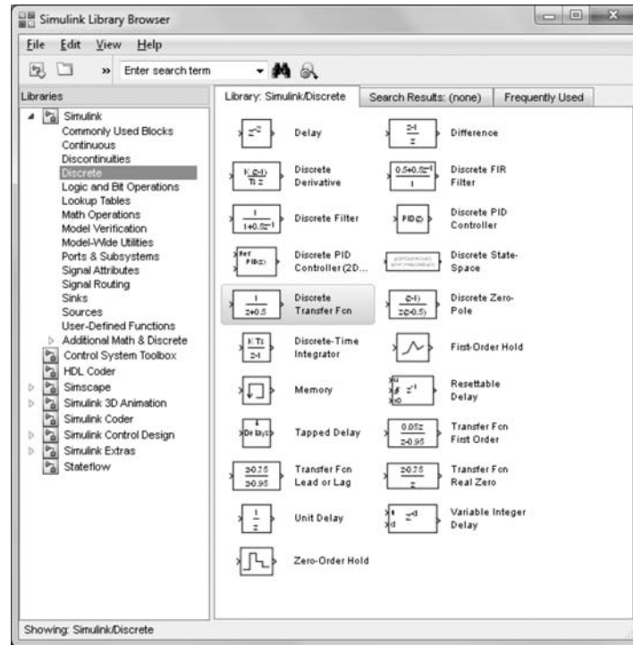
FIGURE C.16 Simulink library of discrete blocks
