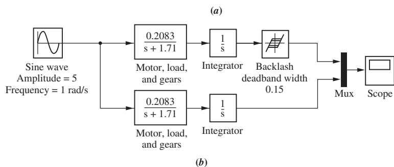
FIGURE 4.31 a. Effect of backlash on load angular displacement response; b. Simulink block diagram
