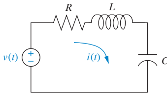
FIGURE P1.7 RLC network
