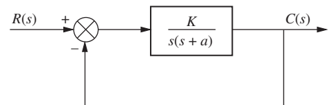
FIGURE 5.14 Second-order feedback control system
