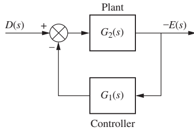
FIGURE 7.12 Figure 7.11 system rearranged to show disturbance as input and error as output, with R(s) = 0
