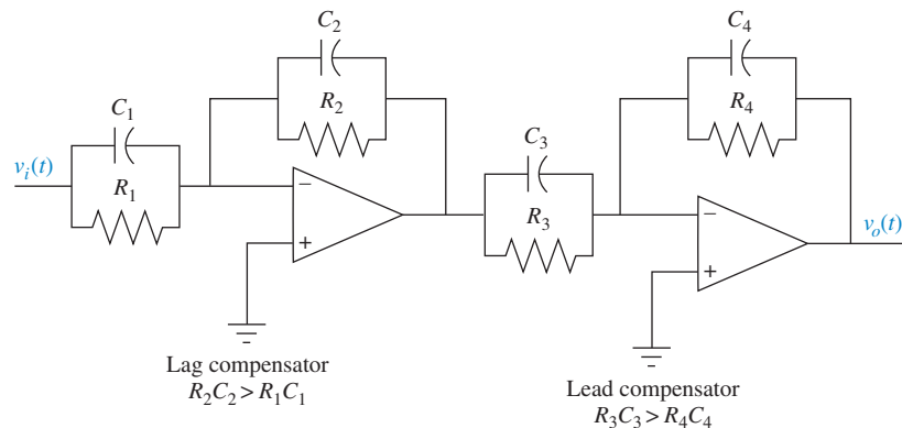
FIGURE 9.61 Lag-lead compensator implemented with operational amplifiers
