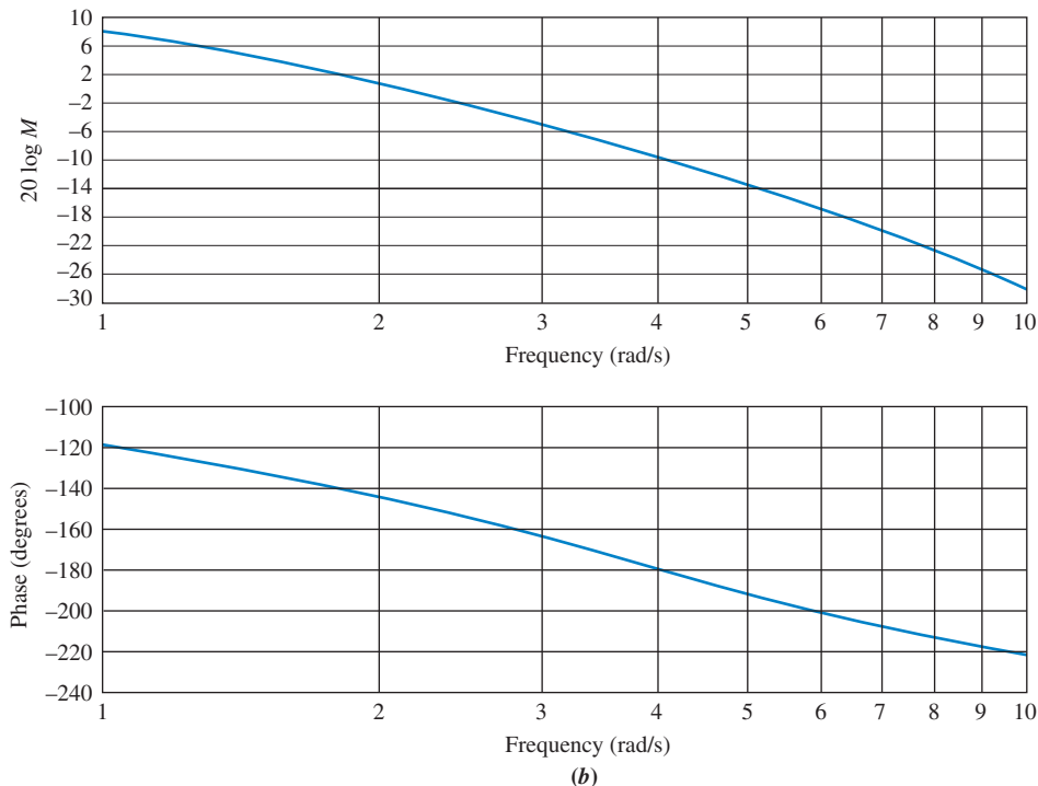
FIGURE 10.50 a. Block diagram; b. Bode diagrams for system of Example 10.13
