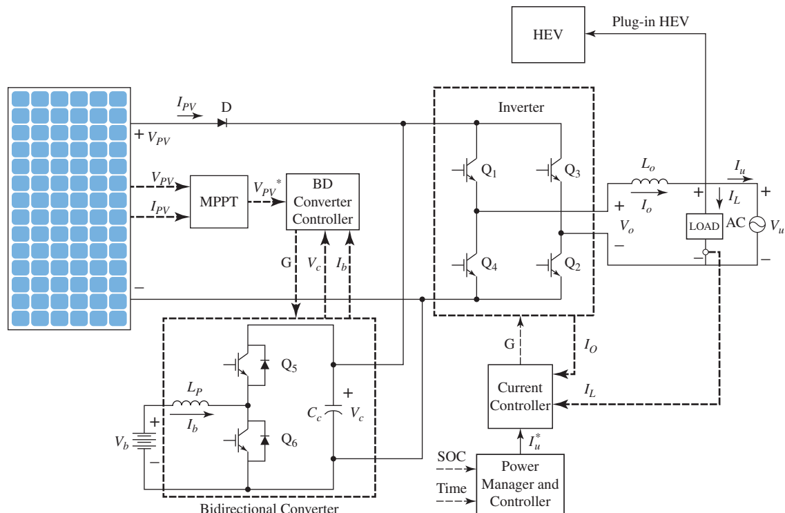
FIGURE P1.5 Proposed solar powered residential home with plug-in hybrid electric vehicle (PHEV) loads 8
