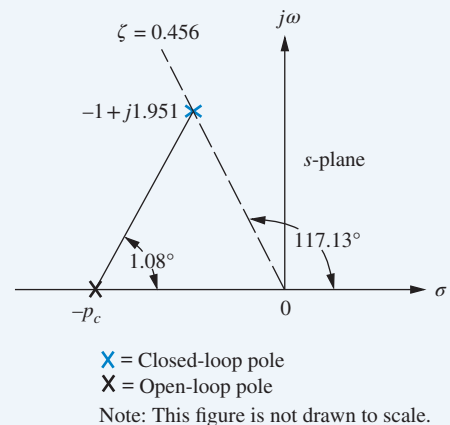
FIGURE 9.67 Locating compensator pole
