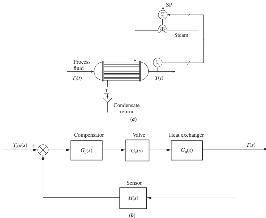
FIGURE P9.6 a. Heat-exchanger process; 7 b. block diagram
