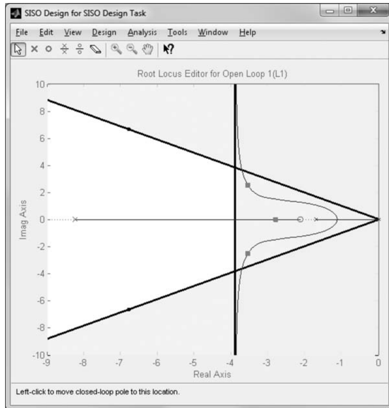
FIGURE C.27 Root locus showing design boundaries of 4% overshoot (radial lines) and 1 second settling time (vertical line) with adjustable gain, PID zero, and PID pole shown in red
