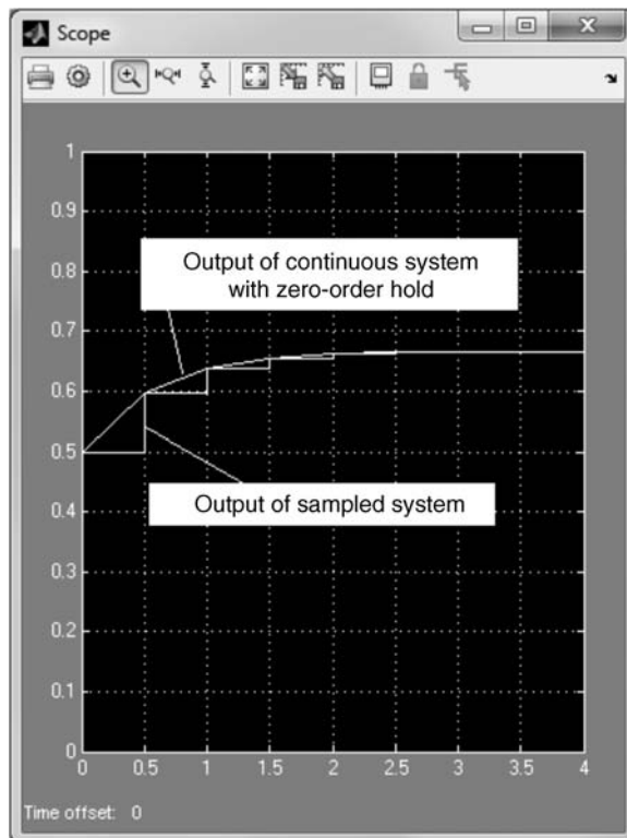
FIGURE C.18 Outputs of the digital systems
