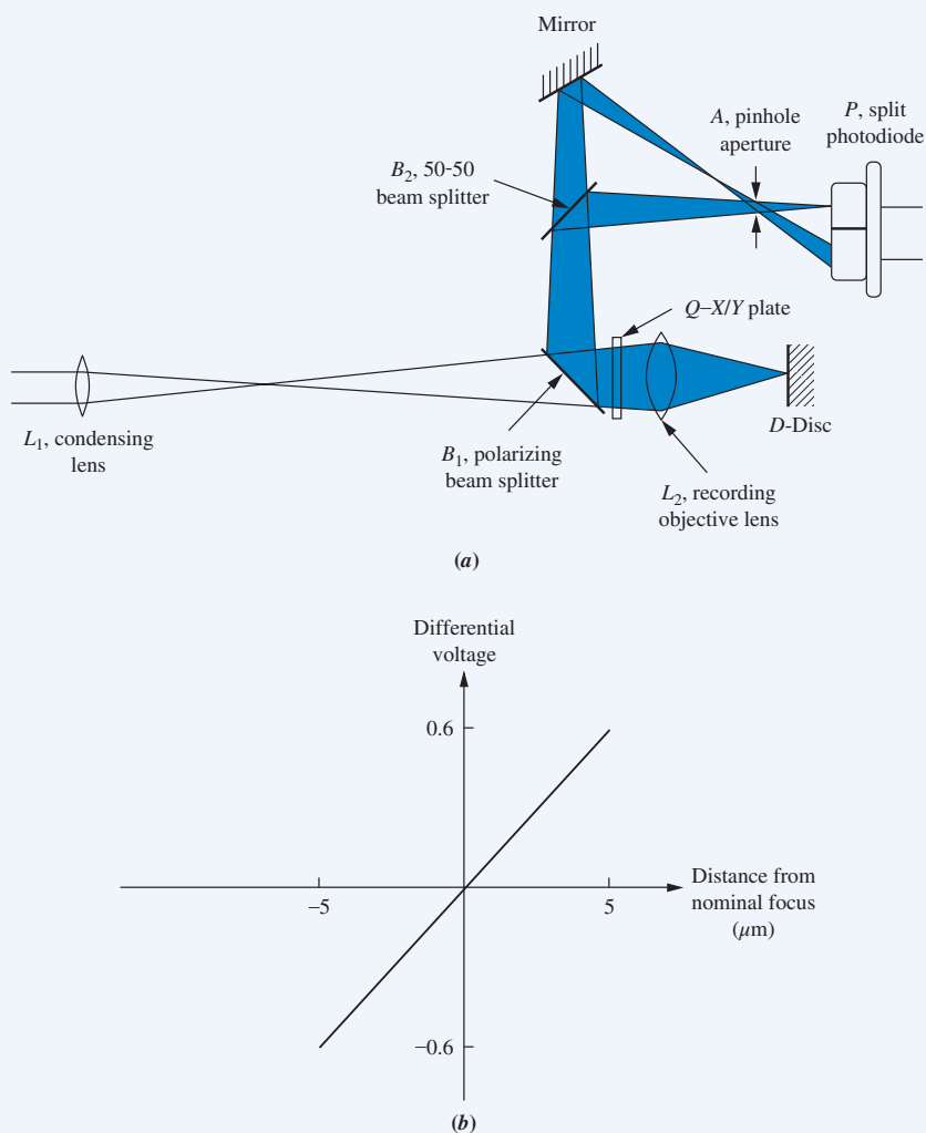
FIGURE 7.23 Video disc laser recording: a. focus detector optics; 6 b. linearized transfer function for focus detector 6
