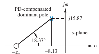
FIGURE 9.33 Calculating the PD compensator zero for Example 9.5
