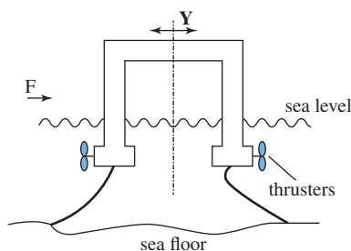
FIGURE P1.4 Tethered platform using side thrusters for positioning 6
