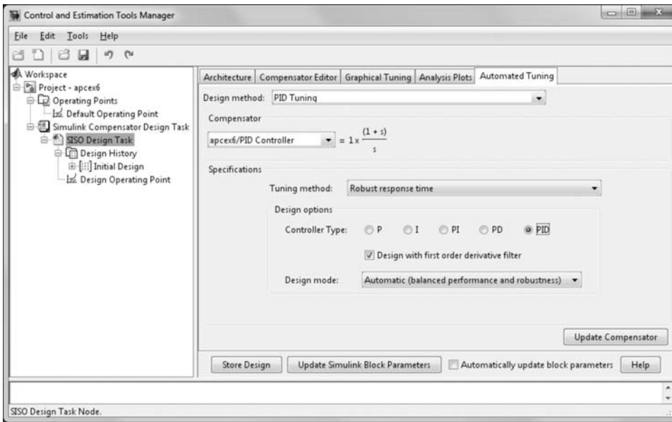
FIGURE C.25 Control and Estimation Tools Manager prepared for automatic PID tuning
