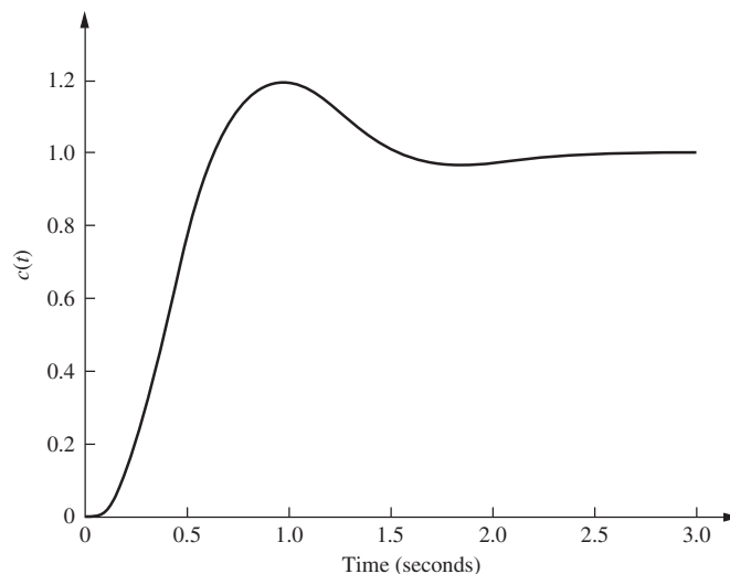
FIGURE 9.51 Step response for uncompensated system of Example 9.7
