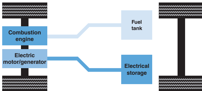
FIGURE P1.9 Parallel hybrid drive 10
