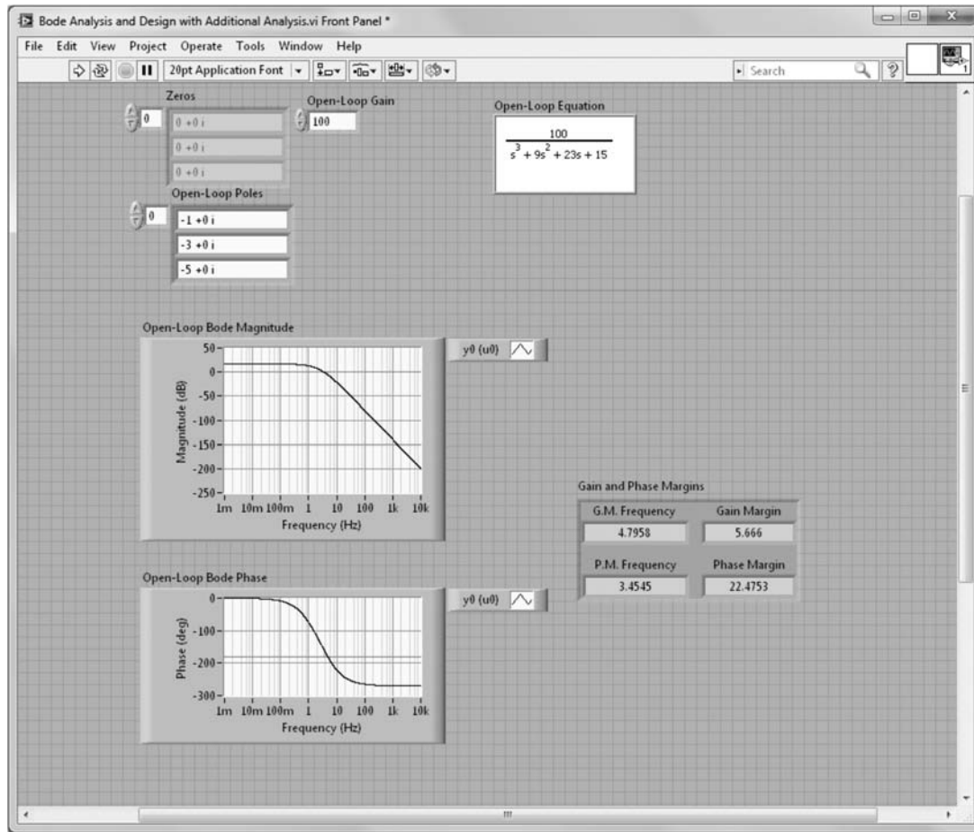
FIGURE D.17 (Continued) b. Front Panel
