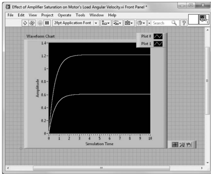
FIGURE D.20 (Continued) b. Front Panel
