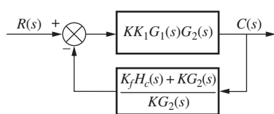
FIGURE 9.48 Equivalent block diagram of Figure 9.45
