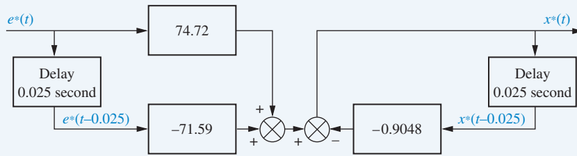
FIGURE 13.36 Flowchart for digital lead compensator 9
