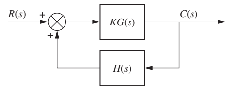
FIGURE 8.26 Positive-feedback system
