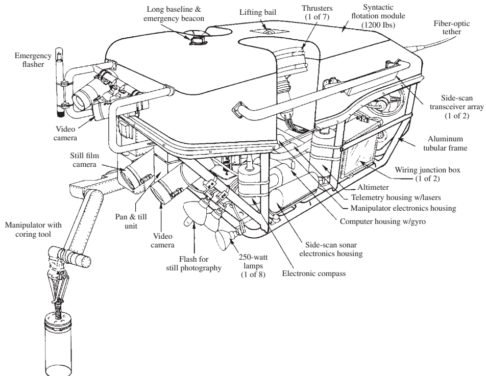
FIGURE 6.9 Jason is an underwater, remote-controlled vehicle that has been used to explore the wreckage of the Lusitania . The manipulator and cameras comprise some of the vehicle's control systems (Courtesy of Woods Hole Oceanographic Institution)
