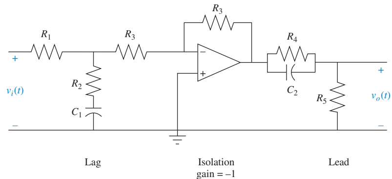
FIGURE 9.63 Lag-lead compensator implemented with cascaded lag and lead networks with isolation
