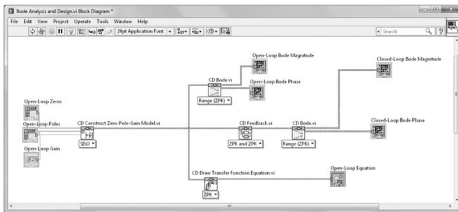
FIGURE D.16 Bode analysis via LabVIEW: a. Block Diagram ; (figure continues)
