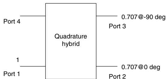
Figure 5-2. Quadrature hybrid operation.
