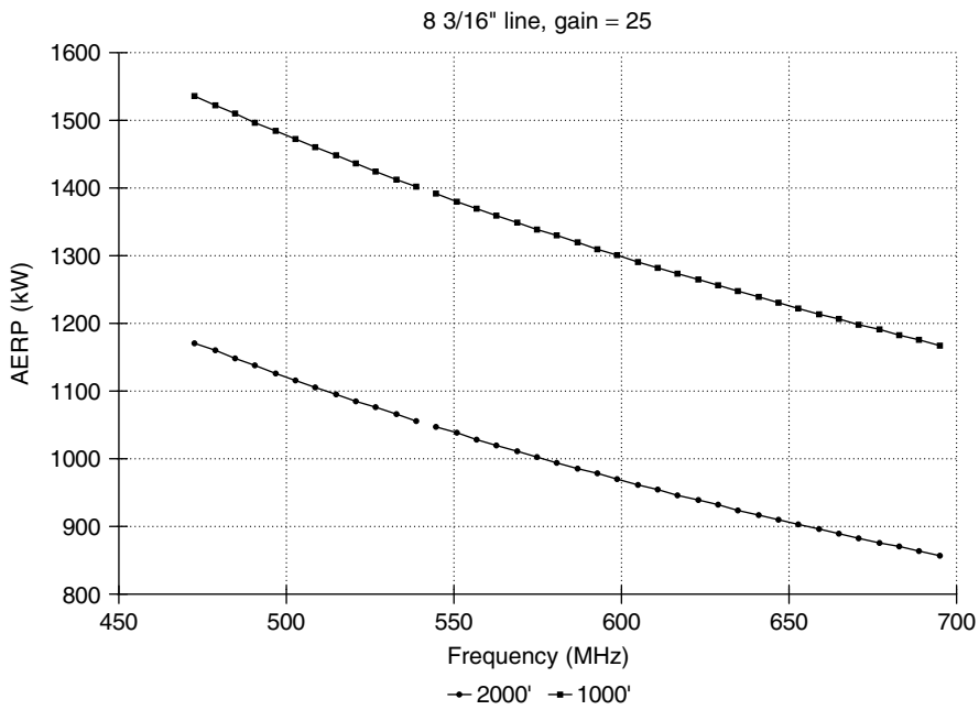
Figure 6-4. Maximum AERP.
