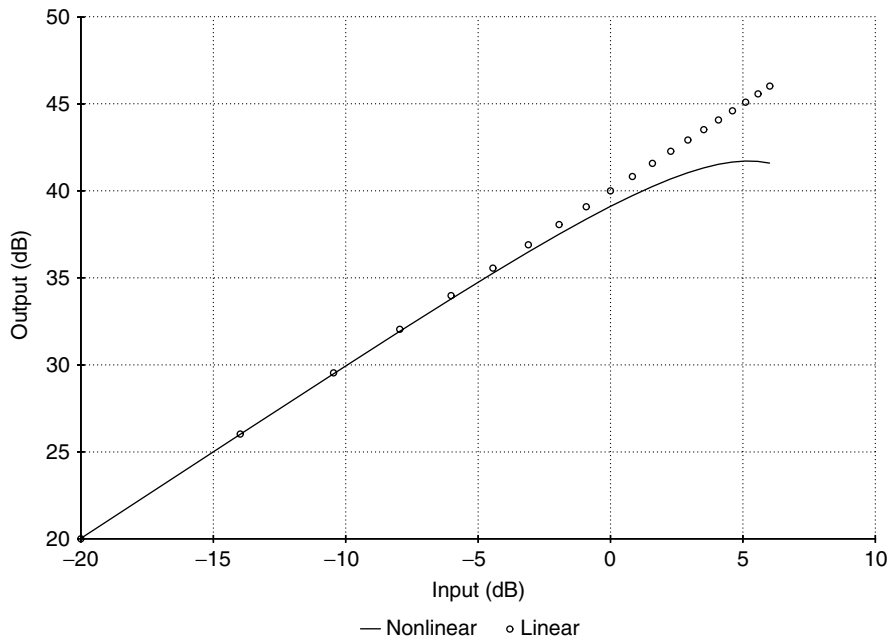
Figure 2-10. Nonlinear amplification.
