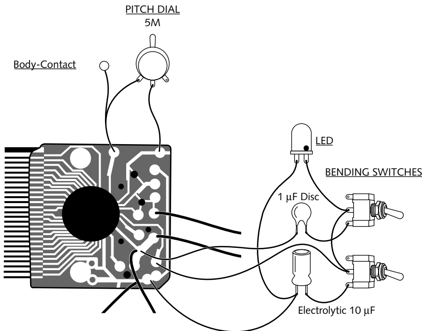
FIGURE 28-2: Bending diagram for the Cool Keys Music Stick. Note that the two capacitors can be soldered to the switch lugs. In this application their polarity is noncritical.
