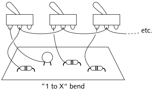
FIGURE A-2: Many of the circuits in this book look to the "1 to X" bend for their basic bent functions. The "X" number is the direct result of how many good bends the traveling end of your bending probe uncovers as it searches the circuit. Accordingly, the "1" in the "1 to X" equation represents the circuit point that the stationary end of the probe rested on while the traveling end of the probe made its tour. Any number of points may be discovered by the traveling end; the final number of switches needed to implement the "X" side of things often exceeds the area available to mount them. Also see the patch bay drawing in this appendix.
