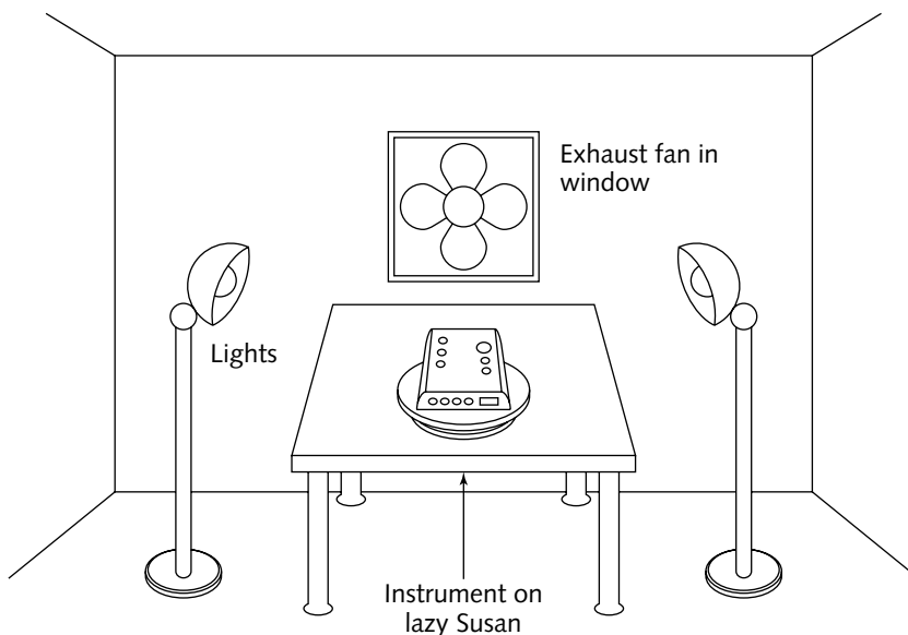
FIGURE 12-4: Simple painting setup for venting fumes
