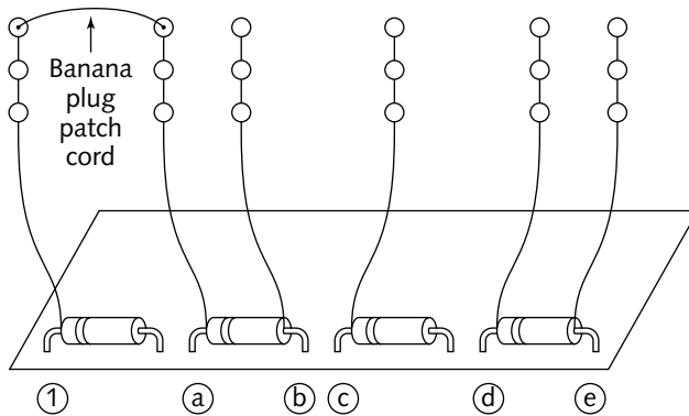
FIGURE 9-16: Patch bay making the same connection as the first toggle switch in Figure 9-14 ("1" to "a").
