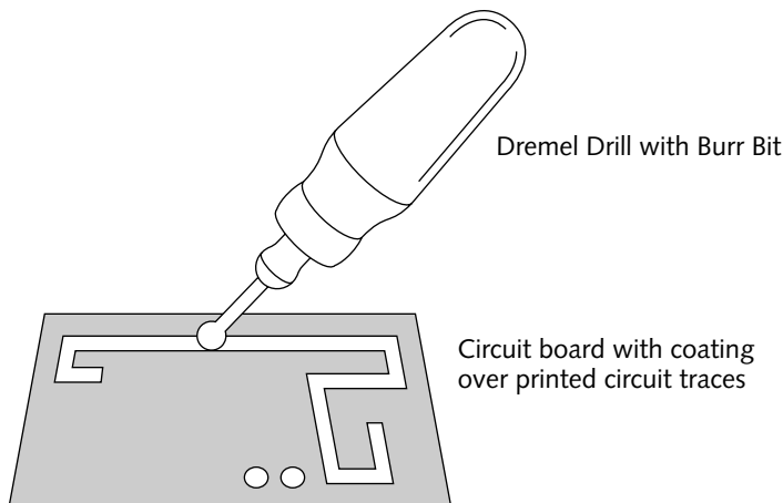
FIGURE 8-14: Use only the lightest pressure to remove a printed circuit's top coating.
