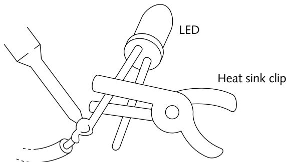
FIGURE 8-13: Heat sink goes between soldering iron tip and component.
