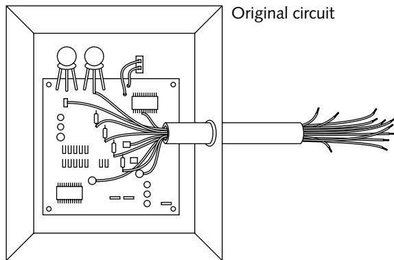
FIGURE 11-5: Insert cable through grommet and solder wires to the bending connections.
