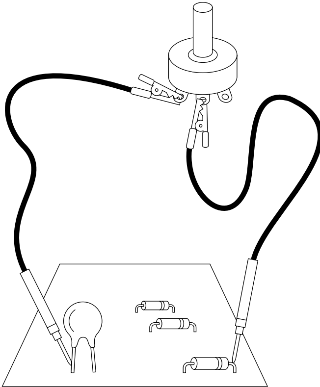
FIGURE 9-19: Probe set with potentiometer in the middle
