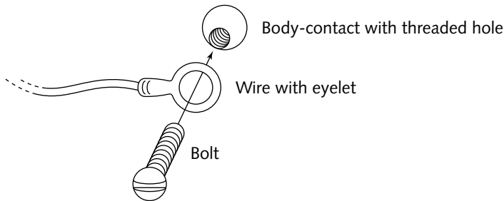
FIGURE 12-9: Wire-to-body-contact
