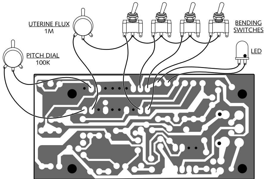
FIGURE 29-2: Bending diagram for the Electronic Womb
