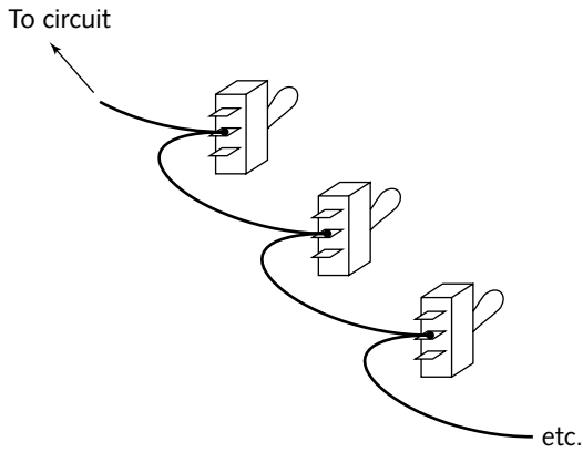
FIGURE 6-22: Bus wire used to connect common contact in a row of switches
