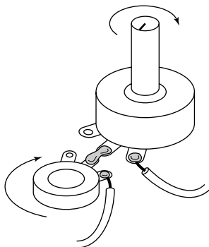
FIGURE 9-24: Turn trimmer dial away from an outside wired lug; turn main pot shaft toward an outside wired lug.
