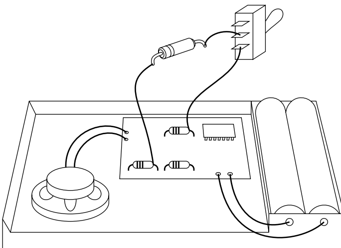
FIGURE 6-10: Circuit-bending wire with resistor and toggle switch
