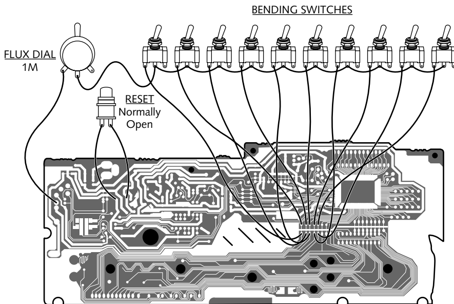
FIGURE 21-2: Bending diagram for the Casio SK-60
