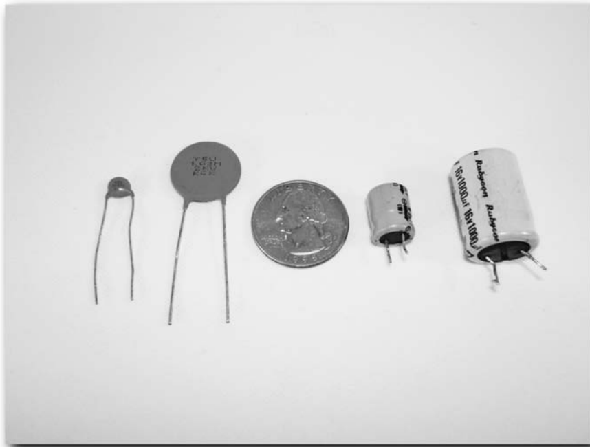
FIGURE 6-16: Assorted capacitors
