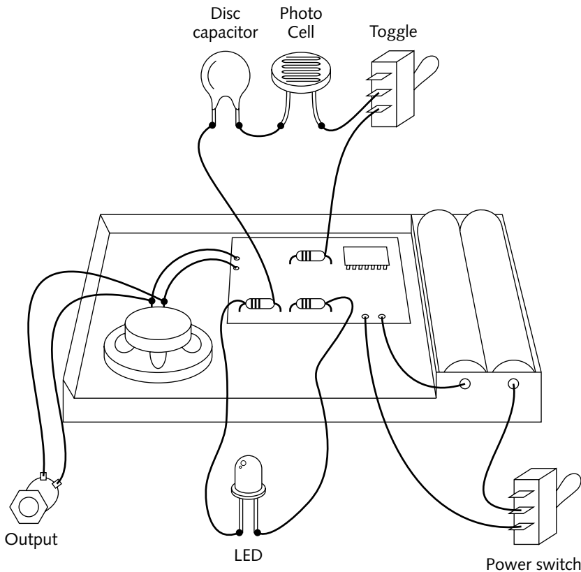
FIGURE 6-19: Circuit with photo cell, capacitor, bend switch, power switch, LED, and line output
