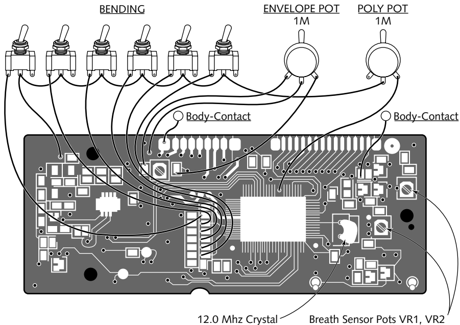
FIGURE 31-2: Bending diagram for the Casio DH 100. Experiment with other potentiometer values for different effects.
