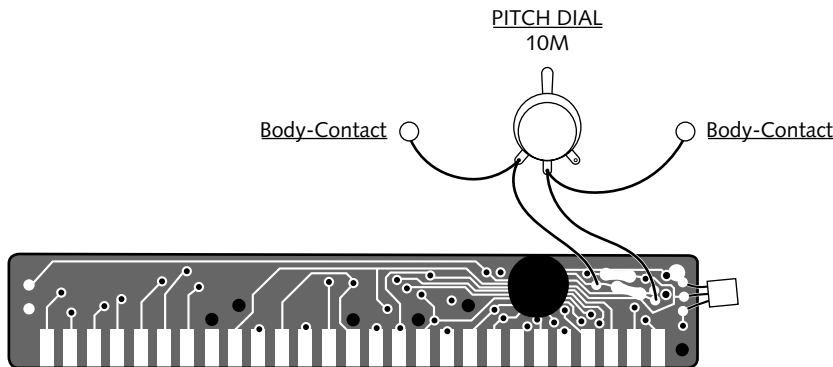
FIGURE 27-3: Bending diagram for the Noisiest Day book strip
