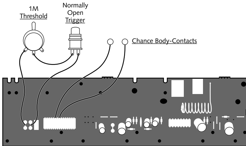
FIGURE 20-1: Bending diagram for the Radio Shack Concertmate 380
