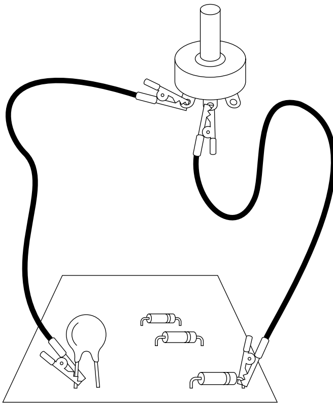
FIGURE 9-20: Leads with alligator clips at each end being used as the probe set
