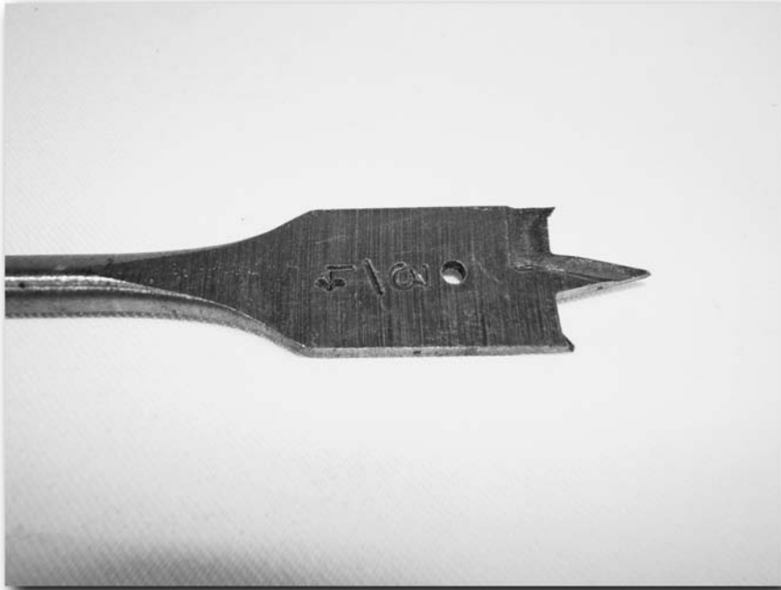
FIGURE 10-5: Spade bits can be used, with caution, on thicker plastic.
