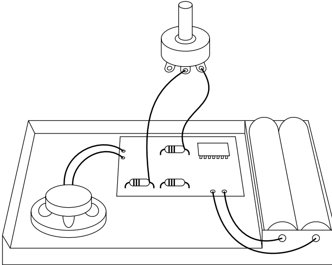
FIGURE 6-13: Circuit-bending wire with potentiometer
