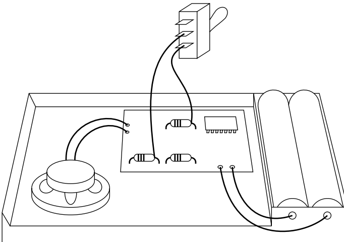
FIGURE 6-4: Circuit-bending wire with three-pole on/off switch
