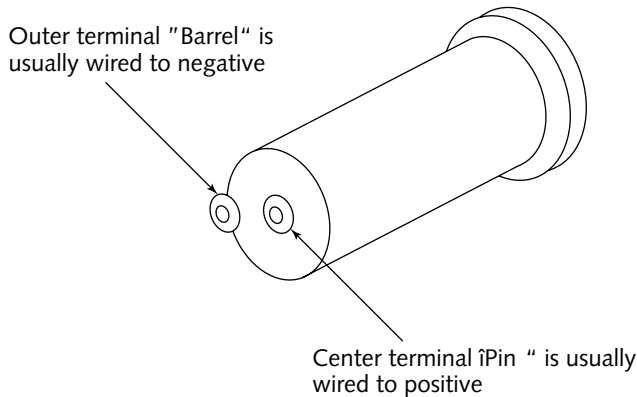
FIGURE 10-12: Power jack soldering terminals
