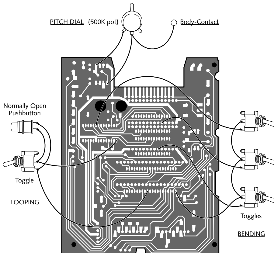
FIGURE 14-2: Bending diagram for the original Speak & Spell circuit board
