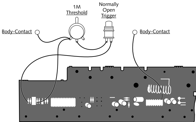
FIGURE 18-2: Bending diagram for the Casio SA-2 Aleatron. Capacitor C2's upper lead is the same as the IC pin that one of the body-contacts connects to (C2 is two capacitors to the right of the target IC pin). If C2's lead that is closest to the chromed battery spring is accessible, you can solder the body-contact wire there instead.
