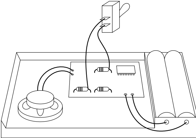
FIGURE 6-3: Circuit-bending wire with two-pole on/off switch
