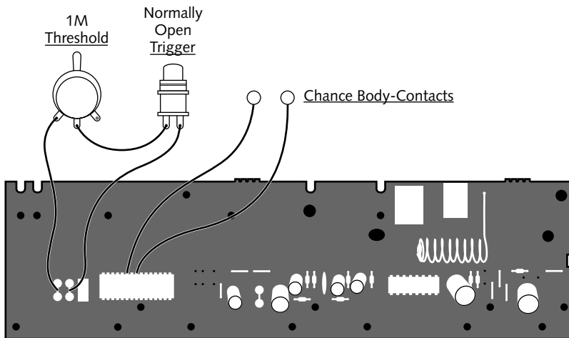
FIGURE 19-2: Bending diagram for the Casio SA-5 Aleatron
