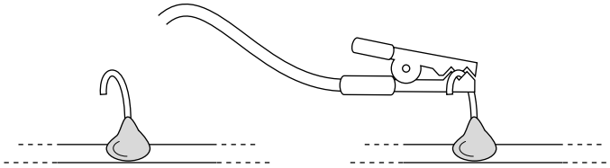
FIGURE 9-21: Soldering a wire to a hard-to-clip area will give you something to clip a test probe to.
