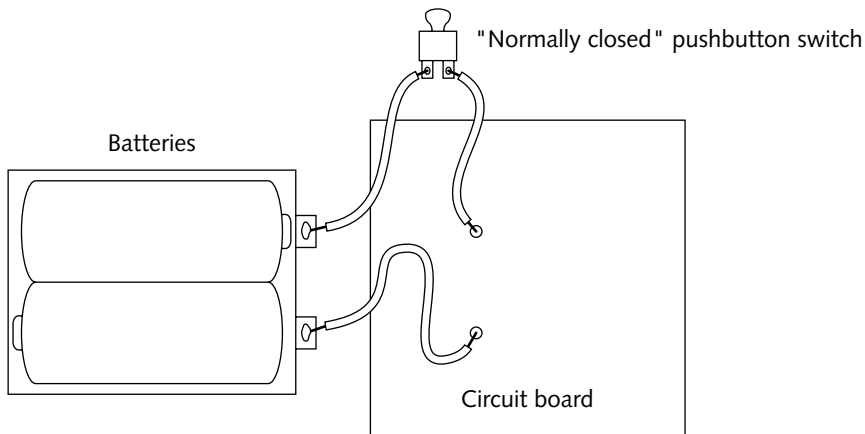
FIGURE 9-28: A normally closed pushbutton switch on a battery compartment wire
