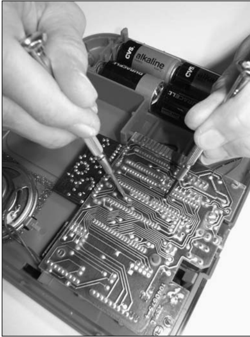
FIGURE 9-12: Using screwdrivers to search for body-contacts
