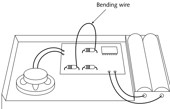
FIGURE 6-2: Circuit-bending wire soldered in place
