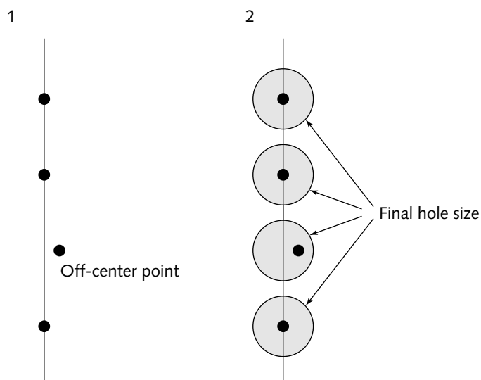
FIGURE 10-7: An off-center pilot hole can be enlarged back onto center.
