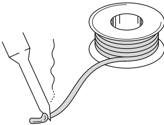
FIGURE 8-24: Cutting solder off the roll with your soldering tip
