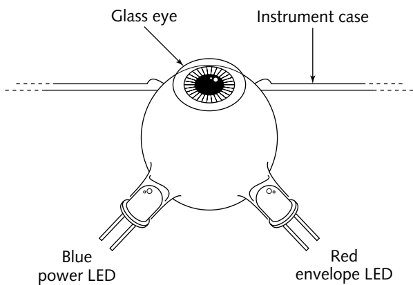
FIGURE 12-18: Back lighting a glass eye with LEDs glued in place
