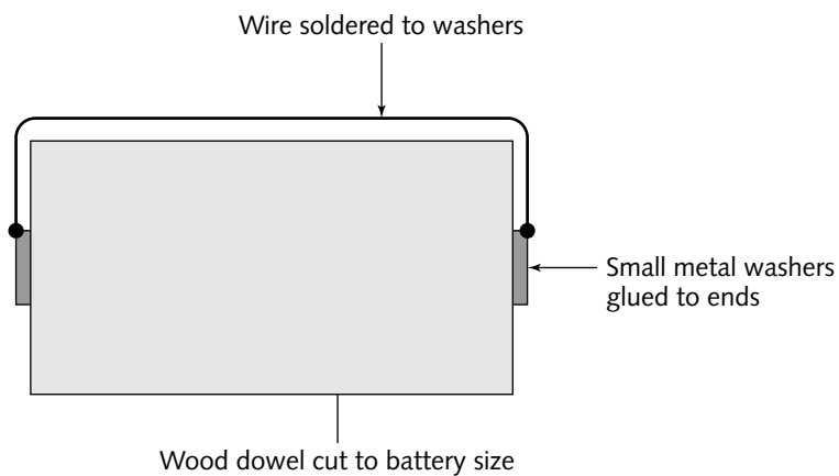
FIGURE 6-28: Making your dummy cells
