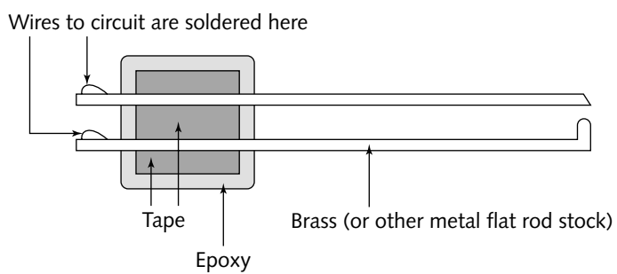
FIGURE 6-8: Cutaway of homemade reed switch
