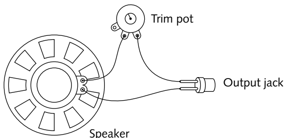
FIGURE 9-27: Put a trimmer in-line with an output wire to tame your line outputs.
