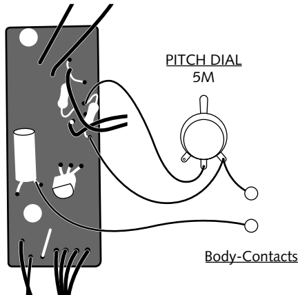
FIGURE 26-2: Bending diagram for the Electronic Rap Pad. The 5M potentiometer replaces the resistor to its left (see Appendix A for a drawing of resistor replacement).
