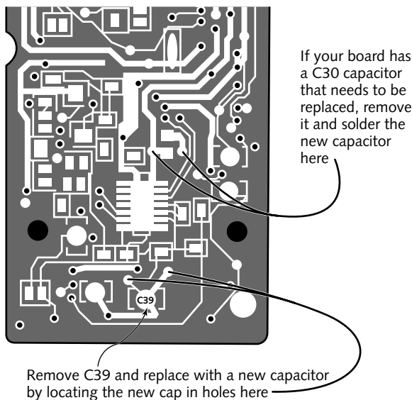
FIGURE 31-3: The two suspect capacitors behind the common DH 100 squeal are C39 (shown) and C30 (absent from the board illustrated). After the offending capacitors are removed, the new caps can be soldered into the locations (holes) shown.
