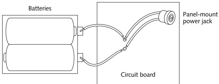
FIGURE 10-13: Solder extension wires to the wires already coming from the battery compartment.
