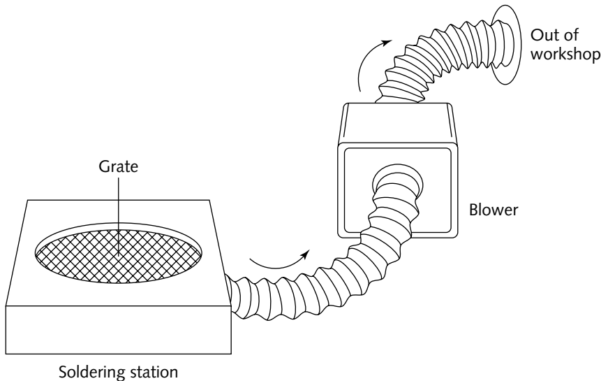
FIGURE 7-4: Design of the DIY down-draft soldering station
