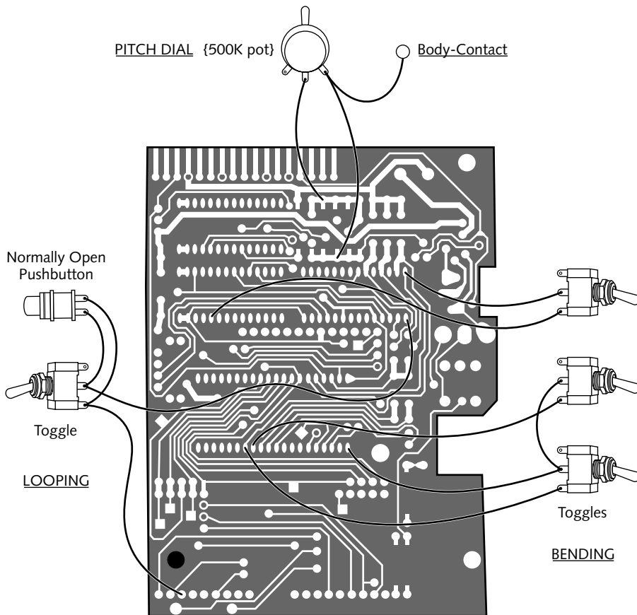
FIGURE 17-2: Bending diagram for the Speak & Math circuit board
