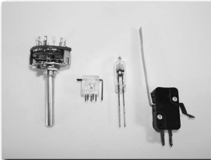
FIGURE 6-7: Specialty switches: rotary, ball, mercury, and micro-switch
