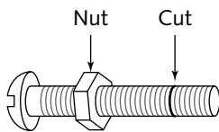
FIGURE 12-10: Put a nut on the bolt you're cutting and unscrew after you're done.
