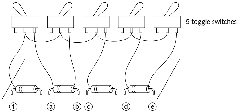
FIGURE 9-14: The “1 to X” bend. In this example, X=five, with each of the five bends running through its own toggle switch, the first of which is turned on.
