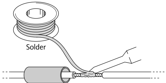
FIGURE 9-5: Twist bare wires together and solder.
