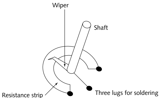
FIGURE 6-12: The potentiometer in action
