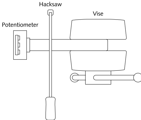
FIGURE 10-10: Use a hacksaw to shorten potentiometer shafts if needed.
