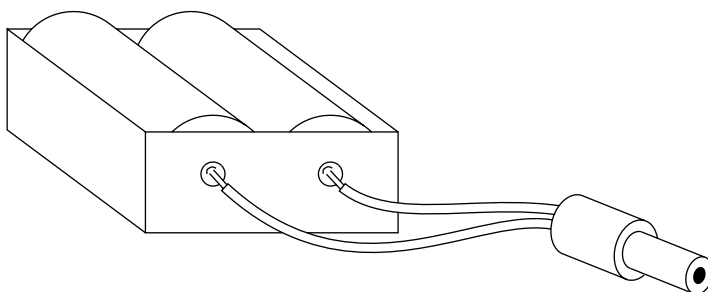
FIGURE 10-11: Battery compartment with power plug soldered on
