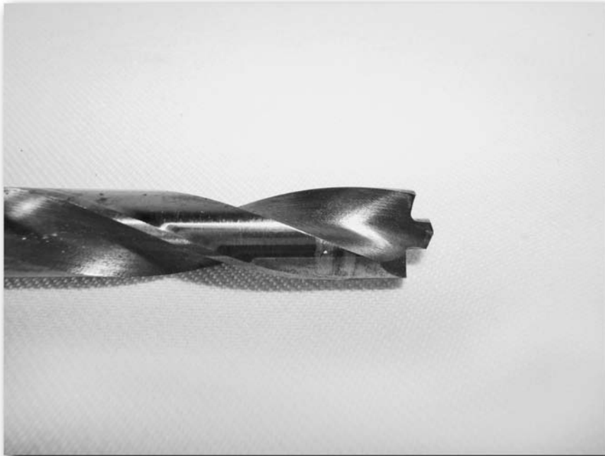
FIGURE 10-4: Spiral bit with self-tapping tip
