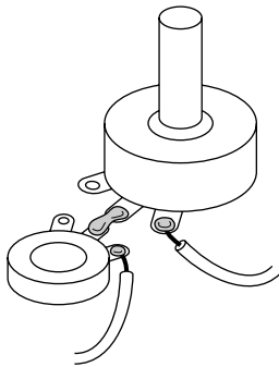
FIGURE 9-23: Solder the pots’ middle terminals together and solder a wire to an outside lug of each, as shown.
