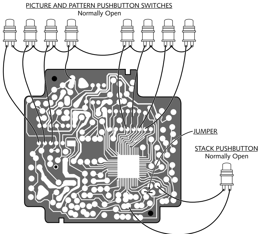
FIGURE 30-4: Bending diagram for the Harmonic Window. Wire your new Record and Play pushbuttons to the points where the originals connected (not shown in illustration; just follow the original wires and solder to the same points).
