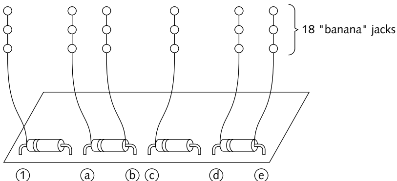
FIGURE 9-15: The same “1 to X” bend configured as a patch bay
