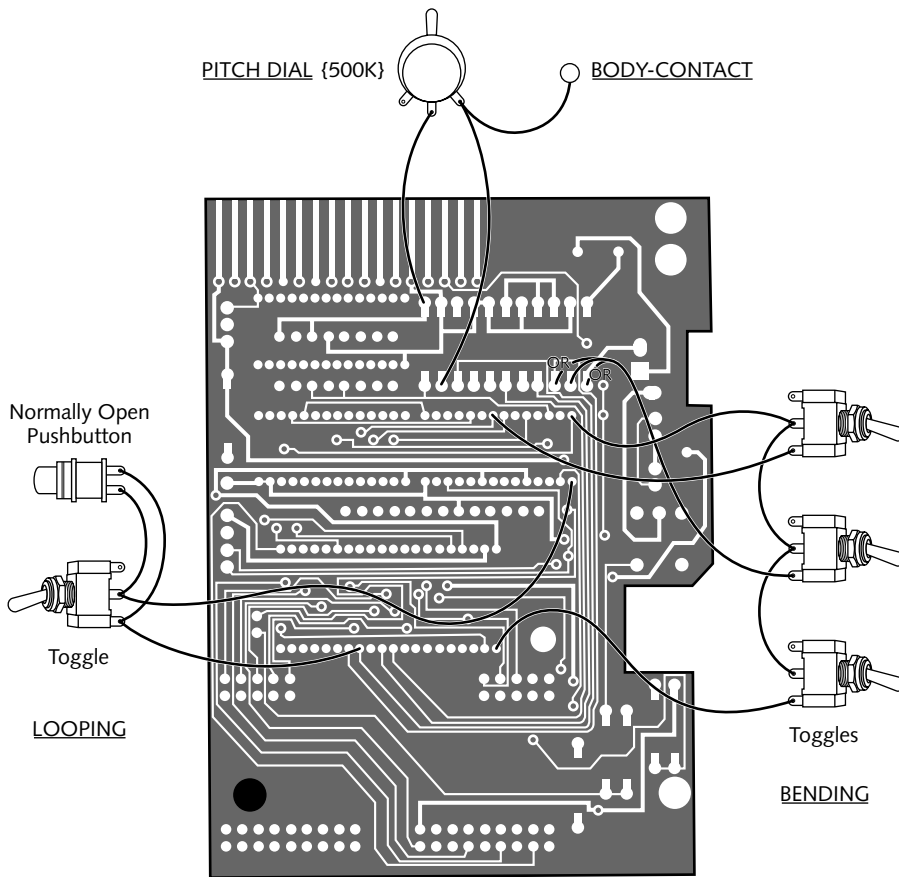
FIGURE 16-2: Bending diagram for the Speak & Read circuit board. Note alternate soldering points for middle bending switch. Using the wrong point will speed up the circuit or otherwise interfere with normal operation.
