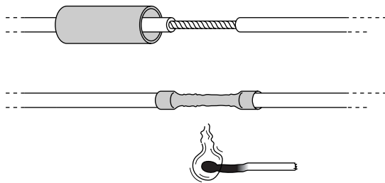
FIGURE 6-29: Slip section of heat-shrink tubing over wire (top), cover soldered connection, and heat the tubing with a lighter or flame to shrink it over the connection.
