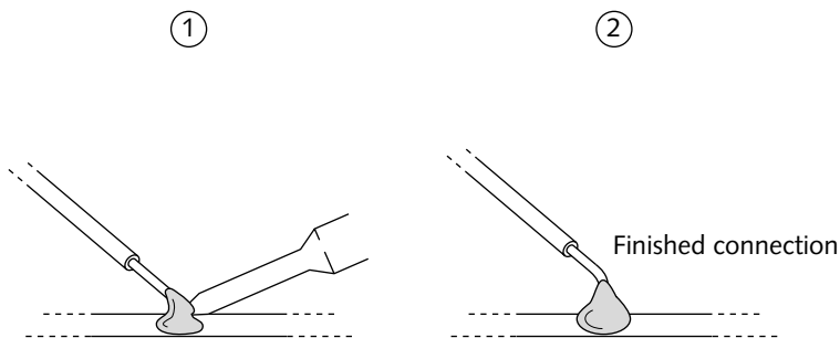
FIGURE 8-16: Solder your wire to solder bump on printed circuit trace.
