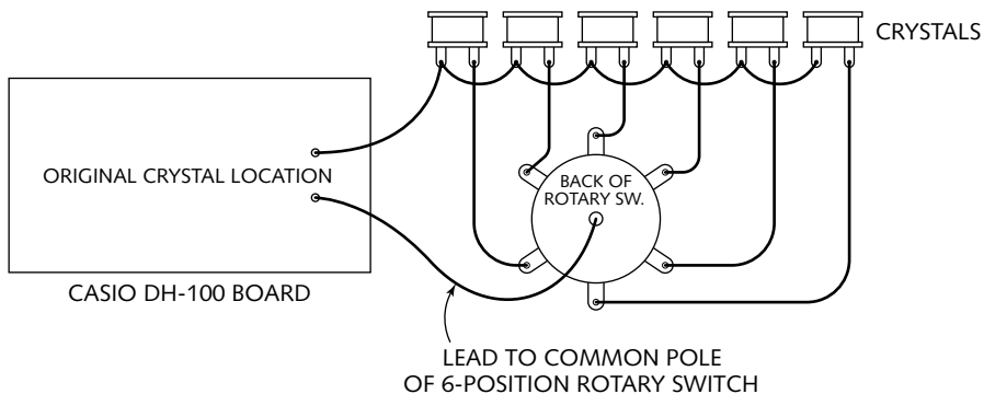
FIGURE 31-4: Use a multiposition rotary switch to select crystals and therefore expand frequency coverage for your DH 100 Hyper Sax.
