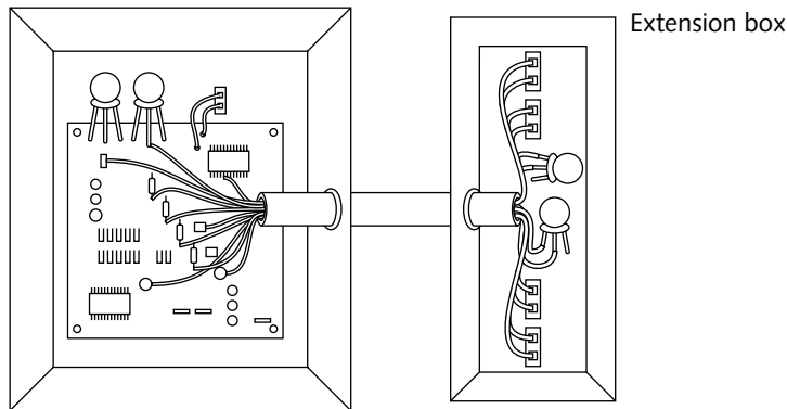
FIGURE 11-6: Insert the cable's other end into the extension box and solder wires to extra components.
