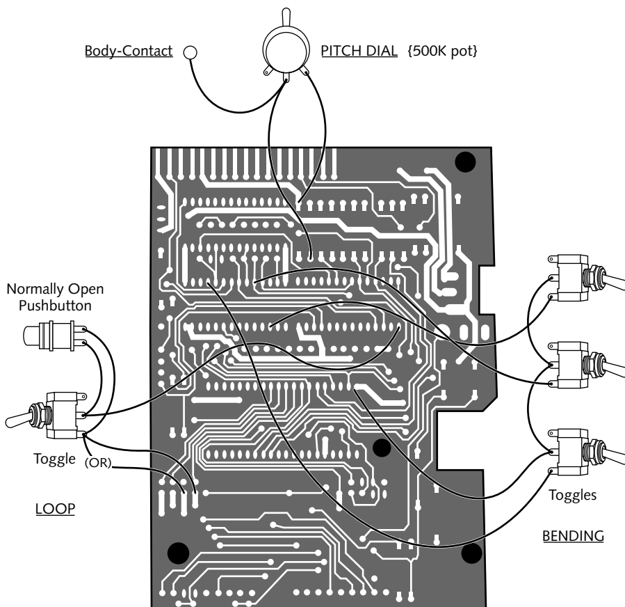
FIGURE 15-2: Bending diagram for the common, membrane-keypad Speak & Spell circuit board. Note alternate soldering point for one of the two looping connections. If the main point doesn't work, try the alternate.
