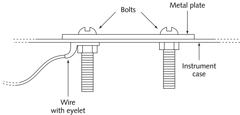
FIGURE 12-12: Wire-to-plate connection
