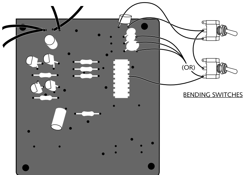
FIGURE 24-2: Bending diagram for the Mall Madness Machine. Note that there are three alternate points, all capacitor leads, that the bottom bending switch can connect to in case you'd rather not solder to the IC pin. Any of the four points works just the same.
