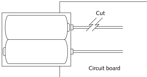
FIGURE 9-29: Cut power supply trace.
