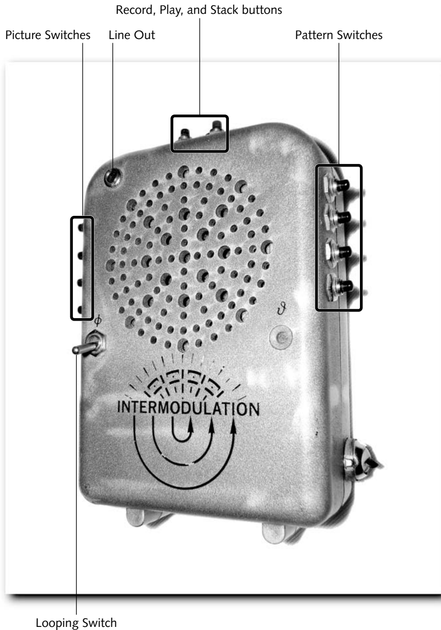
FIGURE 30-1: Miniature Harmonic Window made from the battery compartment/circuit of a sampling teddy bear
