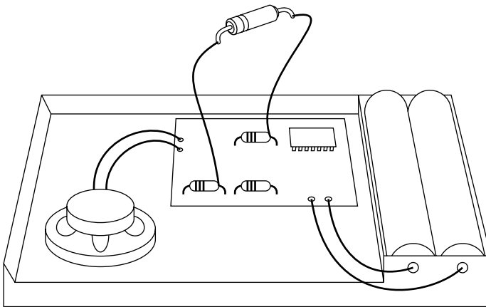
FIGURE 6-9: Circuit-bending wire with resistor
