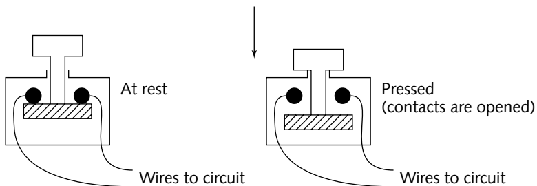
FIGURE 6-6: A normally closed pushbutton switch in action
