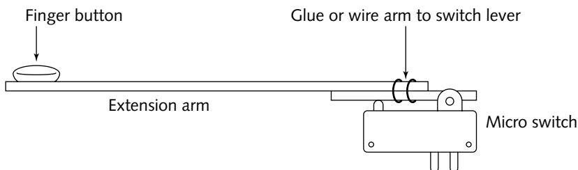
FIGURE 12-13: Extending the feeler lever on a micro switch
