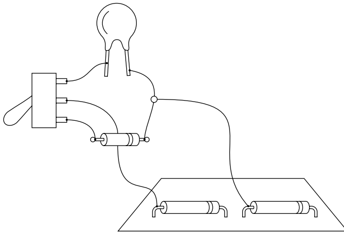
FIGURE 9-25: Simple circuit for using a three-lug toggle switch to choose between two components. This two-way circuit can be used for any two components, including the noteworthy pair of potentiometer and photo cell mentioned in the text.
