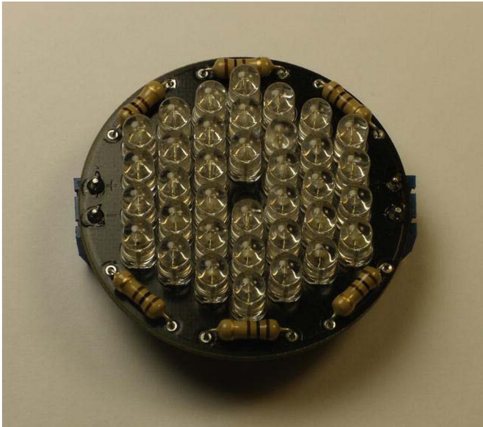
Figure 5-22. An array of six parallel strings of six infrared LEDs in series. These infrared spotlights are used for covert surveillance and security applications.
