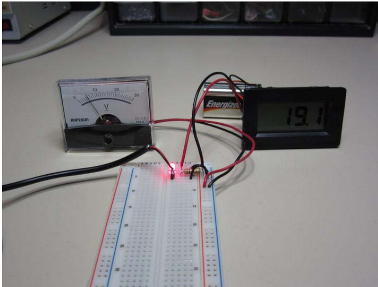
Figure A-12. A digital voltage meter is used to read the voltage across the shunt resistor installed in the circuit. Because the shunt resistor has a 1.0\Omega value, Ohm's Law dictates that the reading in millivolts on the digital meter correspond exactly to the number of milliamps flowing through the circuit. Math is useful, sometimes.
