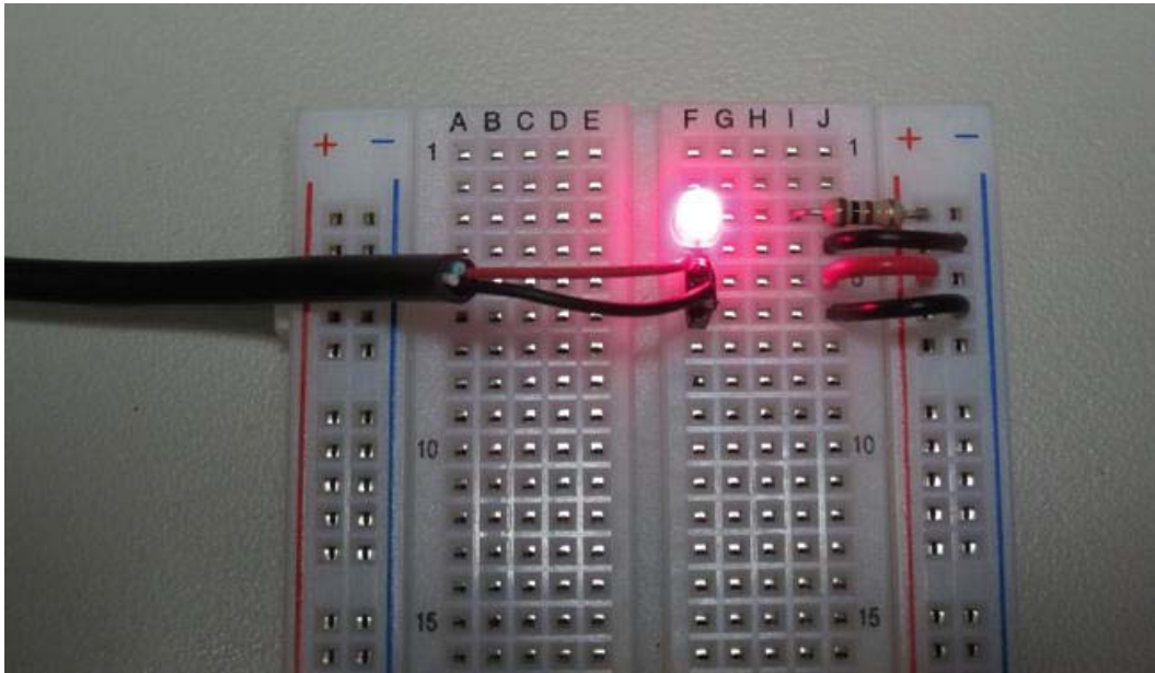
Figure A-10. Add an LED and a current-limiting resistor across the power rails of the solderless breadboard to give an at-a-glance power indicator, right where the action is taking place.
