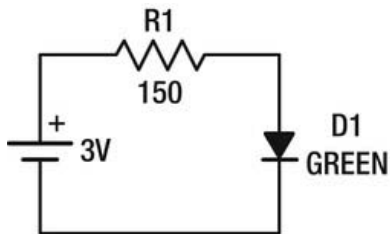
Figure 4-7. The schematic diagram of the LED circuit as built on the solderless breadboard. Schematics are intentionally simpler than reality (most of the time) in order to help convey the very basic idea of how things are to be wired and the relationships between the components, without bogging you down in all the inevitable details that are involved.
