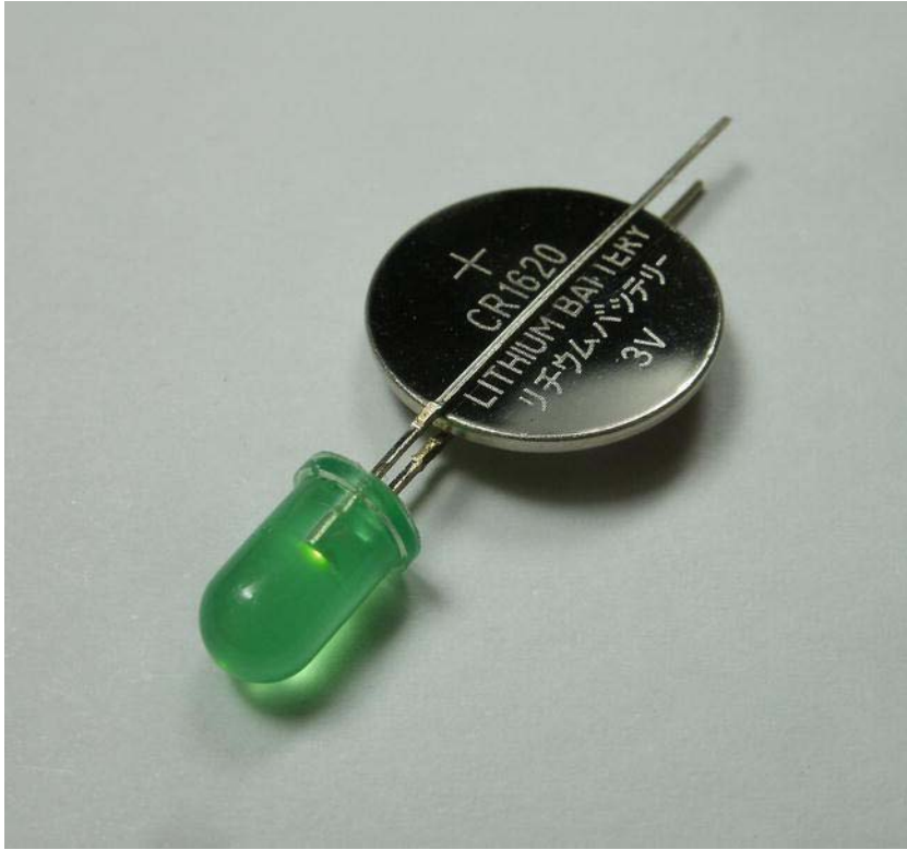
Figure 4-3. A typical LED lights up when attached to a lithium coin cell. No extra wires needed!
