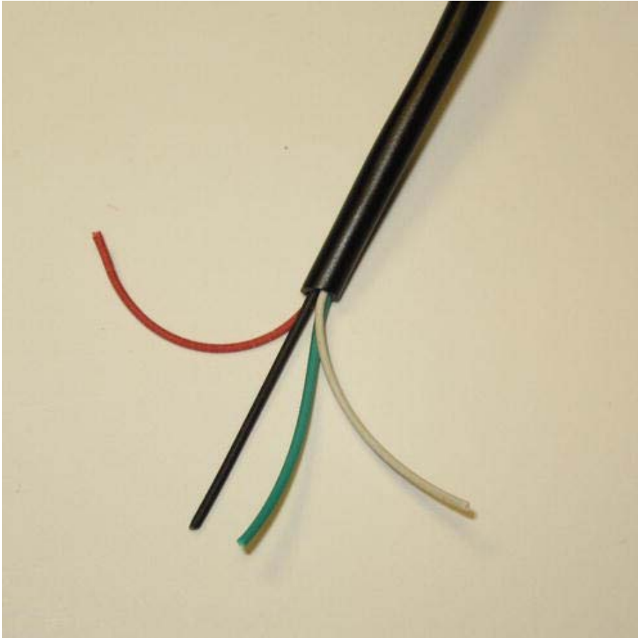
Figure A-6. The four internal wires within the USB cable. From left to right they are red (VBUS or +5V), black (ground), green (USB D+), and white (USB D-). Use the red and black wires to pull a regulated +5V from the charger.
