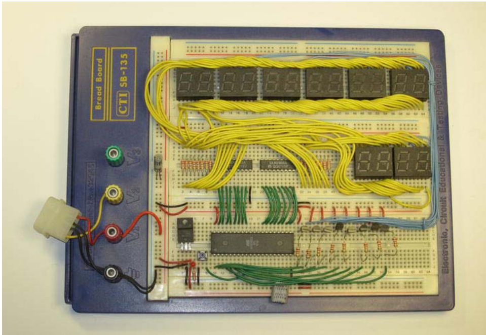
Figure 3-8. A prototype LED display with computer control, built on a solderless breadboard. That's a lot of wires!
