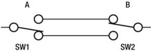
Figure 5-19. A three-way switch circuit built using two SPDT switches. Power is either carried by the upper wire or the lower wire, as long as both switches are in the same position. If not, then no power flows across this part of the circuit. As shown, the three-way switch is effectively off. Flip either switch to turn it on.
