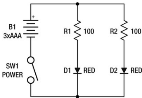
Figure 5-13. The traditional schematic diagram of the two-LED circuit. This diagram should convey the very basic information needed to build the circuit, as well as understand the important aspects of how the circuit is supposed to work, without going into much detail at all about the actual implementation or assembly of the components.
