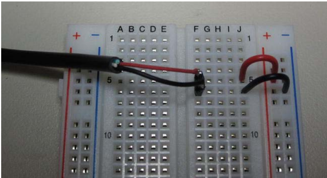
Figure A-9. The regulated power coming from the USB charger is no longer directly connected to the breadboard's power rails. Instead, it is routed to some internal tie points and then connected to the power rails via two short jumpers.
