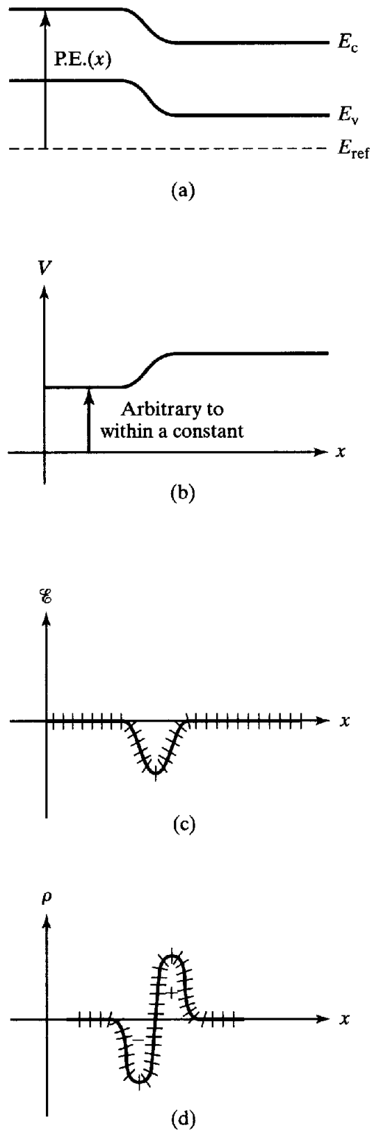
Figure 4.9 Relationship between “band bending” and the electrostatic variables inside a semiconductor. (a) Sample energy band diagram exhibiting band bending. (b) Electrostatic potential, (c) electric field, and (d) charge density versus position deduced from and associated with the part (a) diagram.
