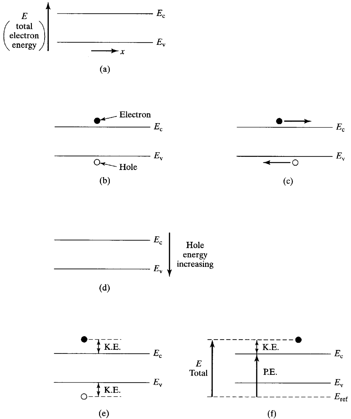
Figure 4.8 The energy band model or diagram. (a) Basic diagram. (b) Representation of carriers. (c) Representation of carrier motion. Diagram interpretation of (d) increasing hole energies, (e) carrier kinetic energies, and (f) the carrier potential energy.
