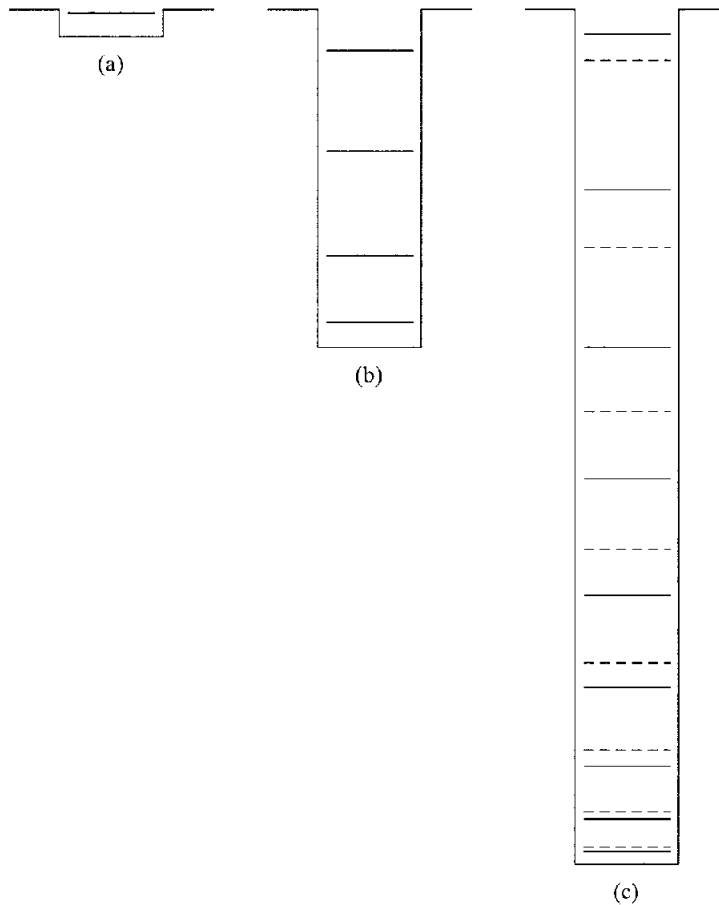
Figure 2.8 Allowed particle energies as a function of potential well depth. (a) Shallow well with single allowed level ( \alpha_0 a = \pi/4 ). (b) Increase of allowed levels when \alpha_0 a exceeds \pi ( \alpha_0 a = 3\pi + \pi/4 ). (c) Comparison of the finite-well (—) and infinite-well (----) energies ( \alpha_0 a = 8\pi + \pi/4 ). All plots are drawn to scale.
