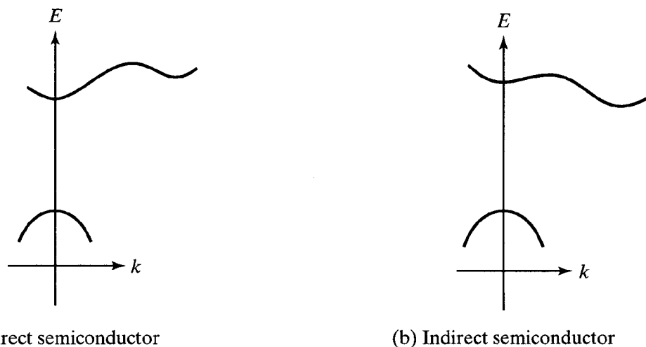
Figure 5.3 General forms of E - k plots for direct and indirect semiconductors.
