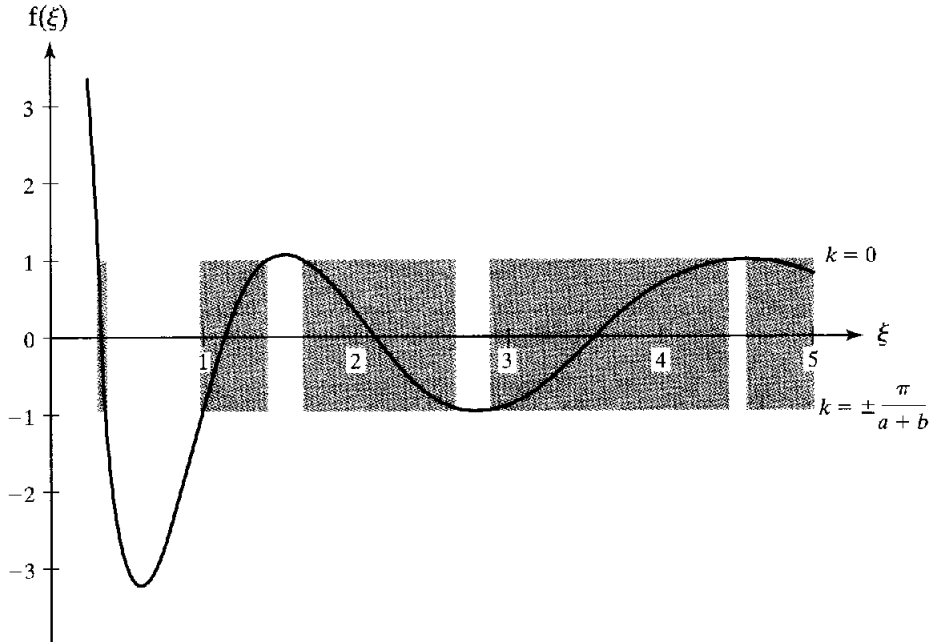
Figure 3.3 Graphical determination of allowed electron energies. The left-hand side of the Eqs. (3.18) Kronig-Penney model solution is plotted as a function of \xi = E/U_0 . The shaded regions where -1 \leq f(\xi) \leq 1 identify the allowed energy states ( \alpha_0 a = \alpha_0 b = \pi ).
