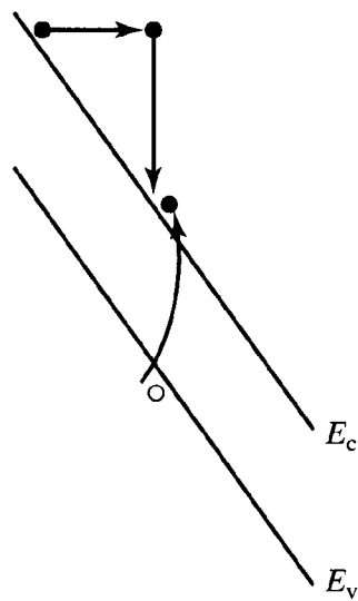
Figure 5.2 Energy-band visualizations of generation processes.
