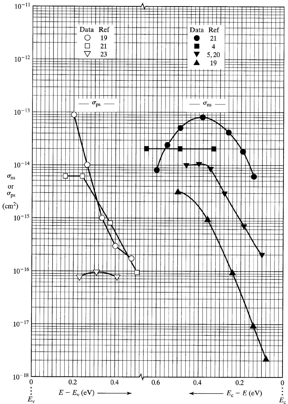
Figure 5.14 Measured electron and hole surface capture cross sections [4,5,19-21,23] characteristic of an optimally processed, (100)-oriented, thermally oxidized Si surface.
