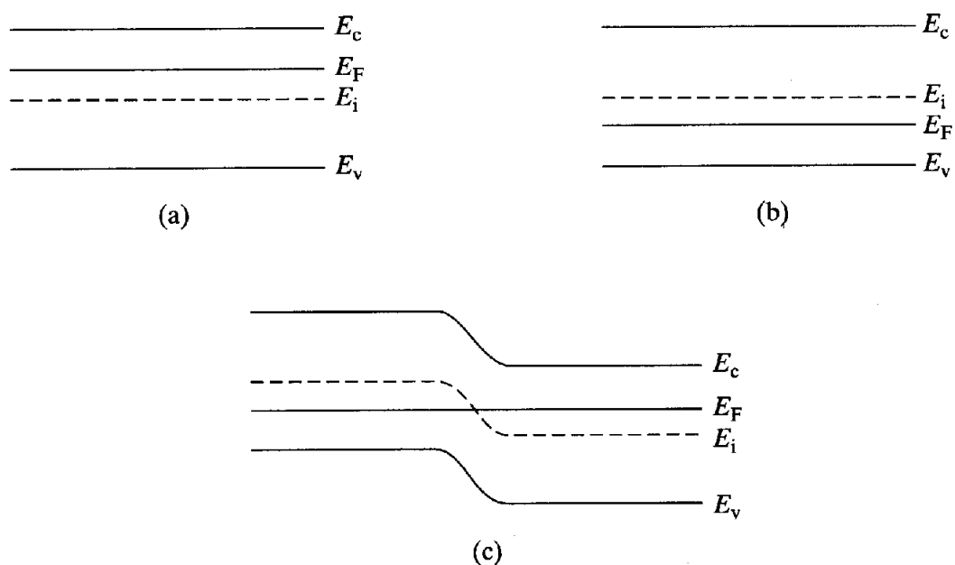
Figure 4.10 Working versions of the energy band diagram containing E_F and E_i . Representations of (a) an n -type semiconductor, (b) a p -type semiconductor, and (c) a pn junction.
