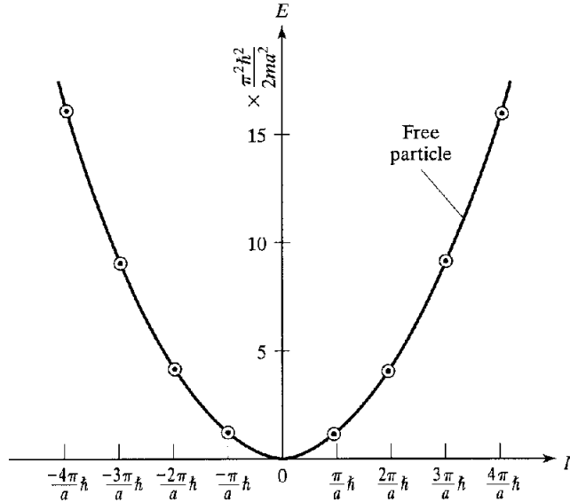
Figure 2.5 Allowed infinite-well particle energy versus counterpropagating wave momentum (discrete points) referenced against the free particle E-(p) relationship.
