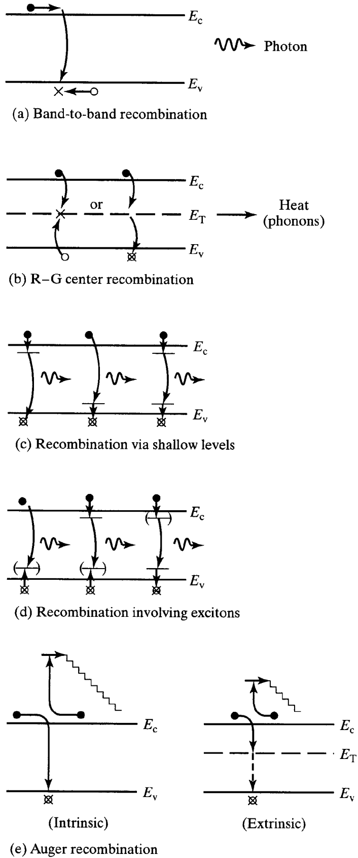
Figure 5.1 Energy-band visualizations of recombination processes.
