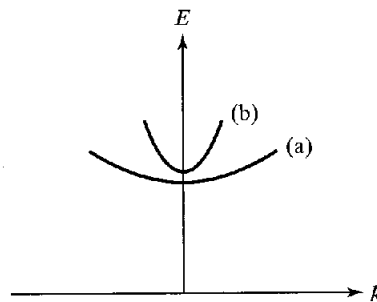
Figure 3.7 Hypothetical band segments used to illustrate how the relative magnitudes of the effective masses can be deduced from curvature arguments. By inspection, m_a^* > m_b^* near k = 0 .
