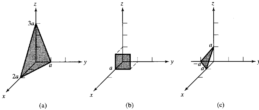
Figure 1.7 Sample cubic crystal planes. (a) The (362) plane used in explaining the Miller indexing procedure. (b) The (100) plane. (c) The ( \bar{1}\bar{1}\bar{1} ) plane.
