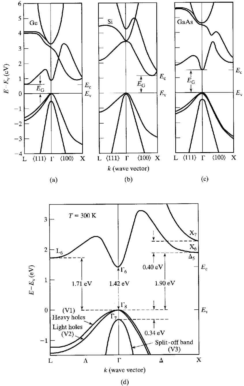
Figure 3.13 \langle 100 \rangle / \langle 111 \rangle E - k diagrams characterizing the conduction and valence bands of (a) Ge, (b) Si, and (c, d) GaAs. [(a-c) after Sze [2] ; (d) from Blakemore. [1] Reprinted with permission.]
