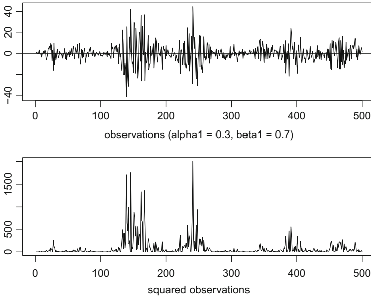
Fig. 6.5 IGARCH(1,1) with \alpha_0 = 1 , \alpha_1 = 0.3 and \beta_1 = 0.7
