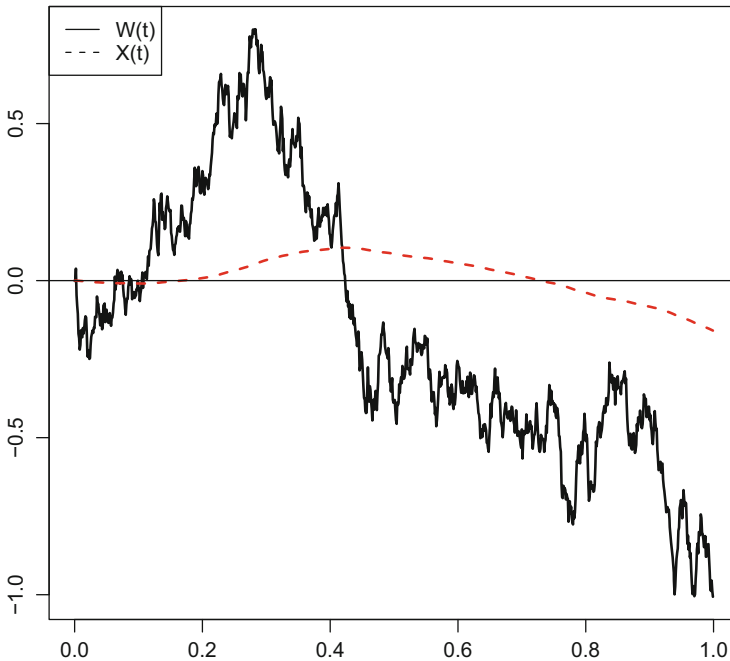
Fig. 7.10 WP and integrated WP
