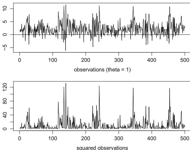
Fig. 6.6 GARCH(1,1)-M from (6.11) with \alpha_0 = 1 , \alpha_1 = 0.3 and \beta_1 = 0.5
