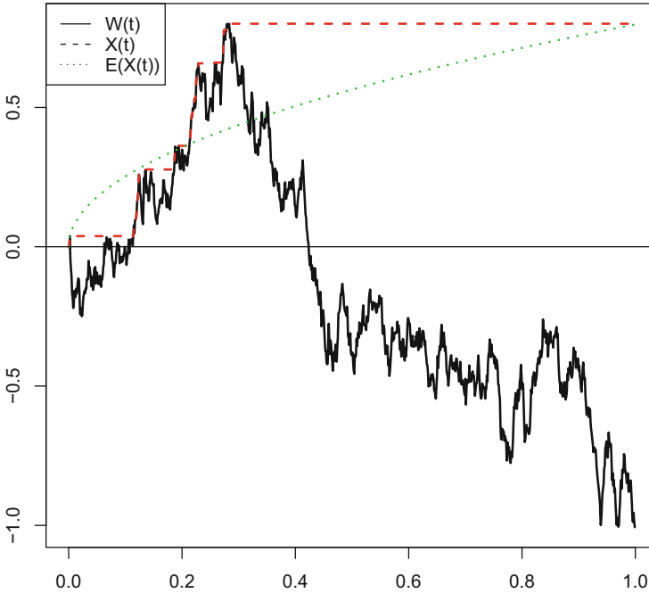
Fig. 7.9 WP and maximum process along with expectation
