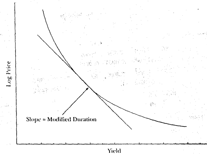
Figure 10.4. The Price-Yield Relationship
