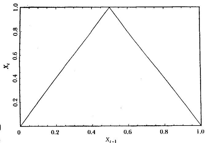
Figure 12.1. The Tent Map
