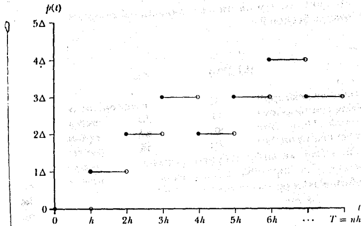
Figure 9.1. Sample Path of a Discrete-Time Random Walk
