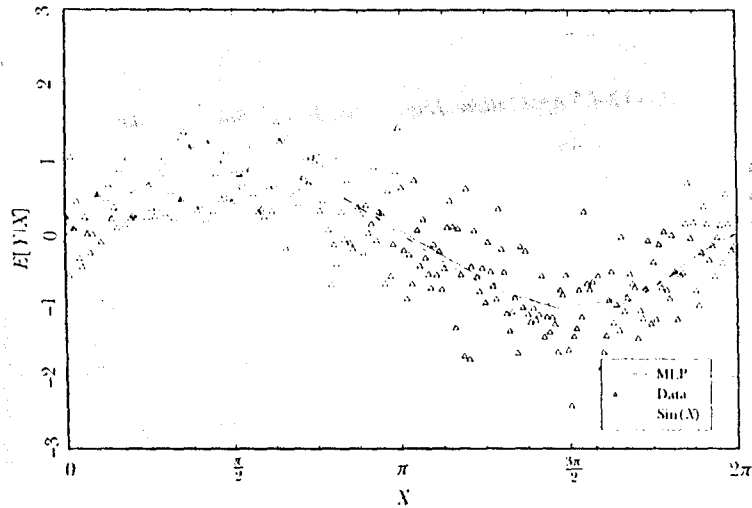
Figure 12.10. MLP(1,5) Model of Y_t = \text{Sin}(X_t) + 0.5\epsilon_t
