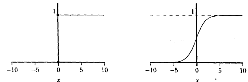
Figure 12.8. Comparison of Heaviside and Logistic Activation Functions
