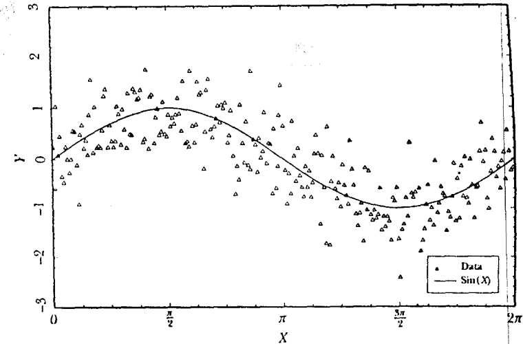
Figure 12.4. Simulation of Y_i = \text{Sin}(X_i) + 0.5\epsilon_i
