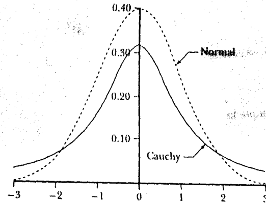
Figure 1.2. Comparison of Stable and Normal Density Functions
