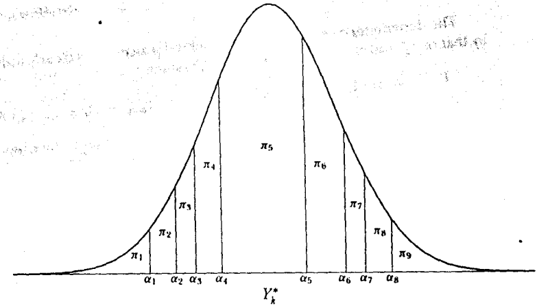
Figure 3.4. The Ordered Probit Model
