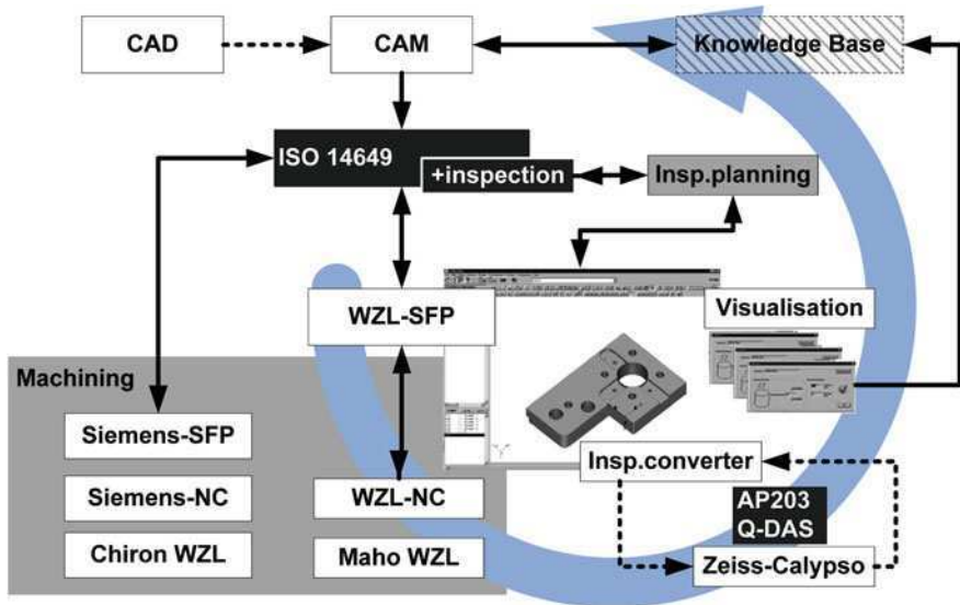
Fig. 4.12 Prototype implementation of the STEP enabled CLM
