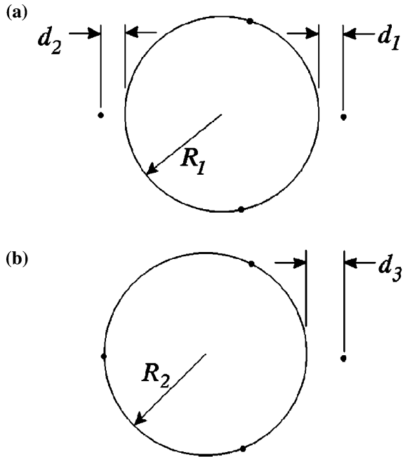
Fig. 6.6 Circles of one-sided minimax; (a) and largest inscribed; (b) fits
