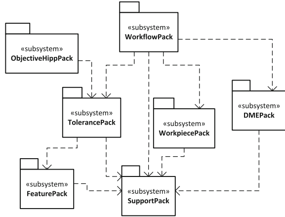
Fig. 4.18 UML support data classes of HIPP data model
