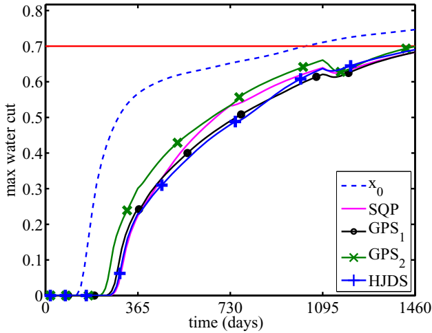
Fig. 2.4 Maximum well water cut for the initial guess x_0 and the four solutions found for the production optimization case. The maximum water cut at a given time is the maximum of the water cut values for all producer wells at that time. The red line indicates the maximum water cut allowed for any producer well. GPS 1 and GPS 2 denote GPS with the penalty function and the filter method, respectively (from [28]); see online version for colors.
