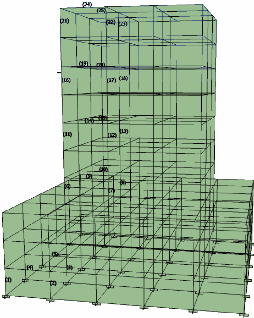
Fig. 6.6 3-D view of ten-story, four-bay steel space frame
