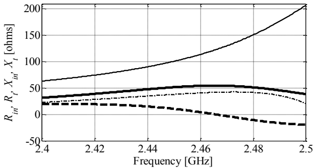
Fig. 3.22 Antenna impedance: resistance R_m (thick solid) and reactance X_m (thick dash) at the antenna input (Fig. 3.19(b)); R_i (solid) and X_i (dash-dot) at the driving element terminals (Fig. 3.19(a)).
