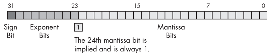
Figure 2-22: Single-precision (32-bit) floating-point format
