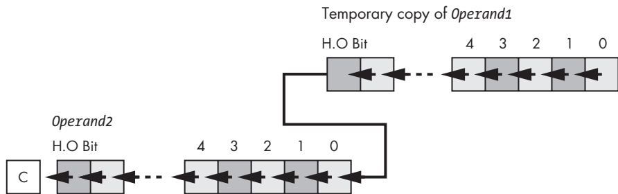
Figure 8-6: shld operation
