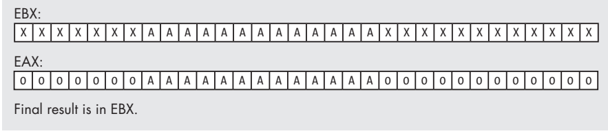
Figure 10-2: Inserting bits 0..12 of EAX into bits 12..24 of EBX
