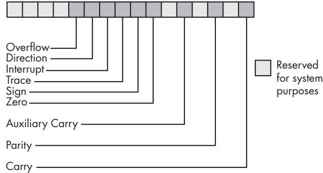
Figure 2-20: EFLAGS register as packed boolean data
