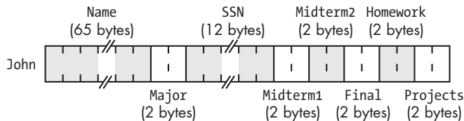
Figure 12-1: student record implementation in memory
