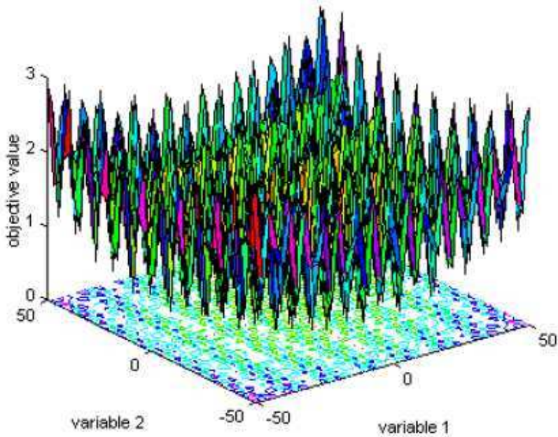
Fig. 12. Griewank's functions
