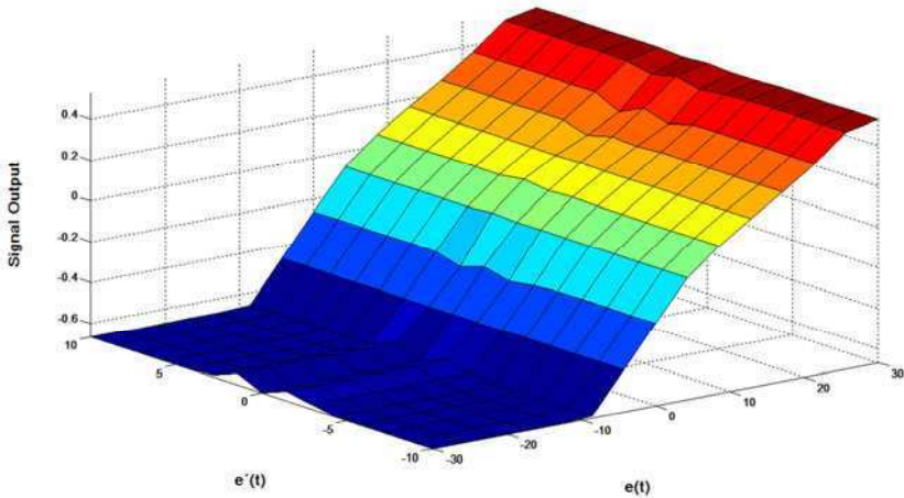
Fig. 22. Control Surface
