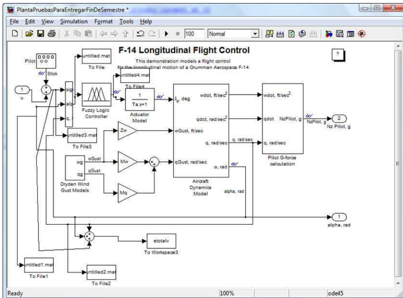
Fig. 8. Simulation Plant with Fuzzy Controller
