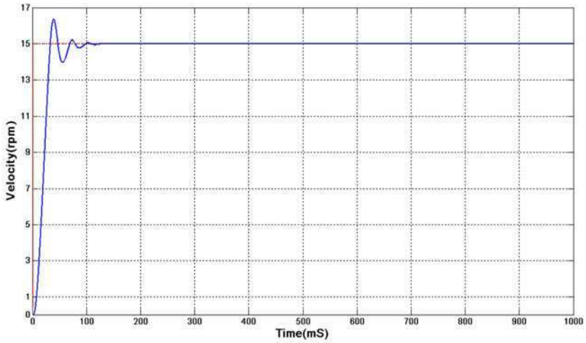
Fig. 23. Experiment 2 Velocity
