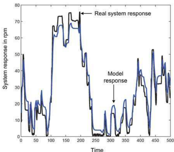
Fig. 4. A pseudorandom sequence to achieve the system identification process was used
