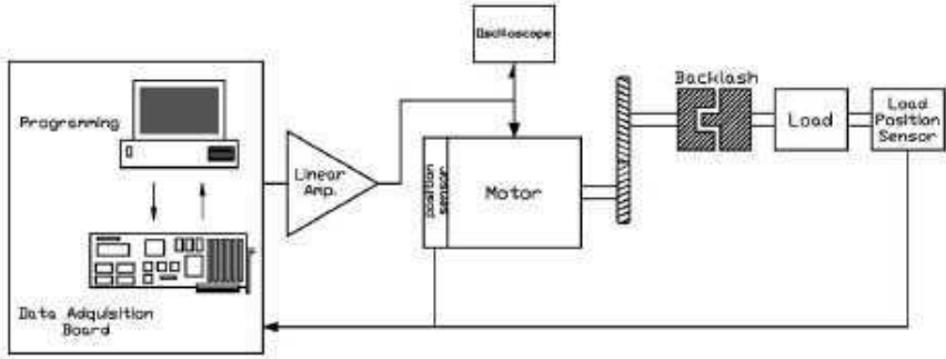
Fig. 4. Control diagram
