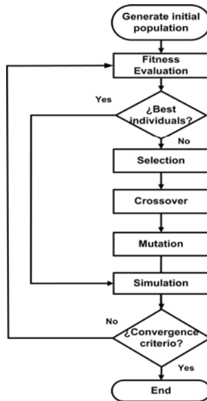
Fig. 10. Optimization GA
