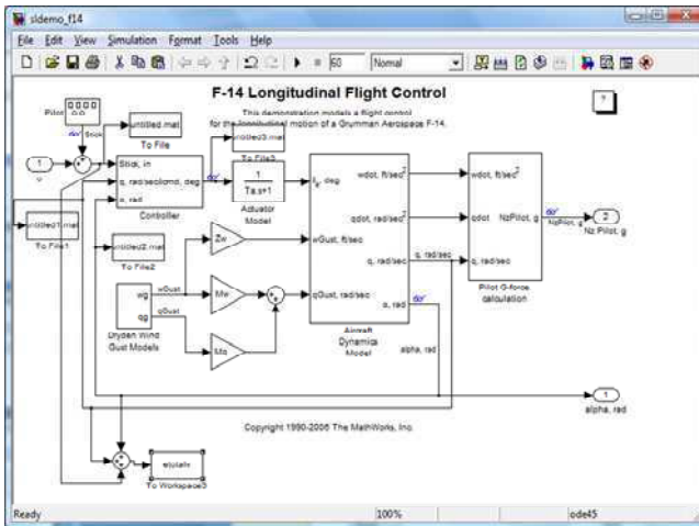
Fig. 4. Simulation Plant with PID Controller
