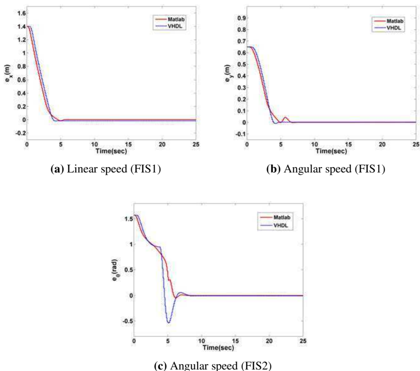
Fig. 12. Performance comparison of modules “LPC-smk” and “LPC-vhdl”. Note that the module coded in VHDL introduces a small error in orientation; however, it can be reduced increasing the length words to represent numbers.
