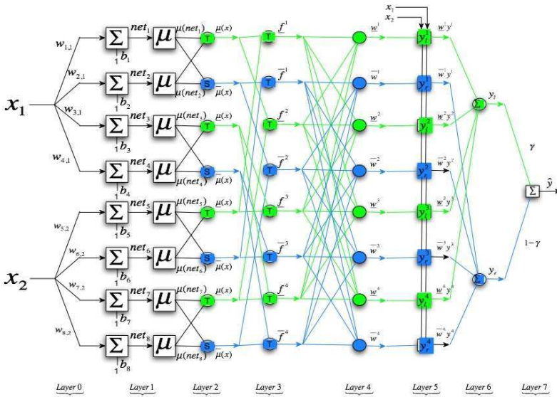
Fig. 3. IT2FNN-0 Architecture
