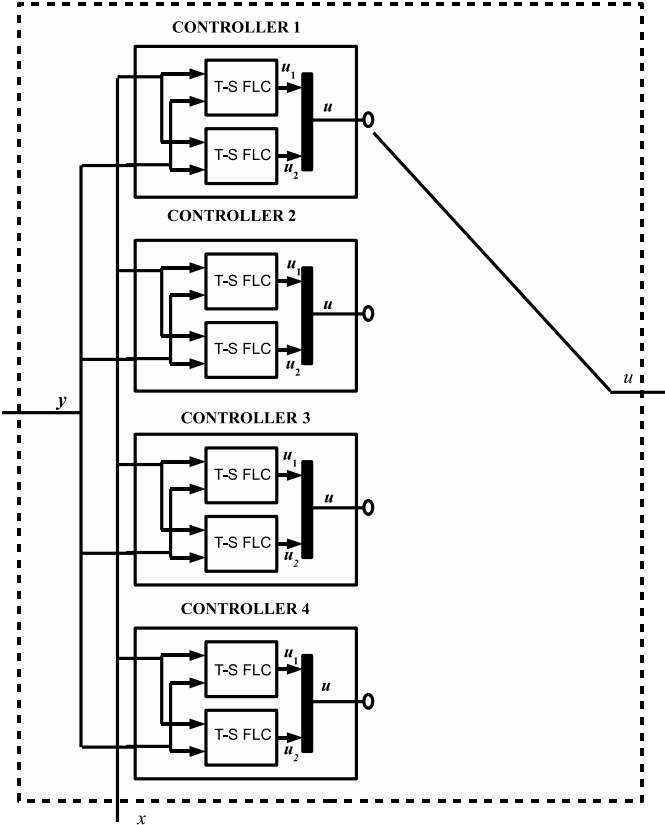
Fig. 2. Controller Structure
