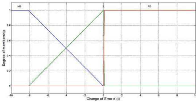
Fig. 12. FIS modified by the GA e'(t)
