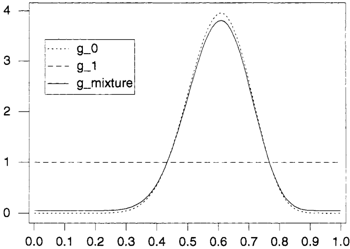
Figure 16.3 Ben's mixture prior and components.
