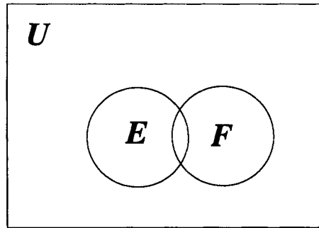
Figure 4.4 E and F are intersecting events.
