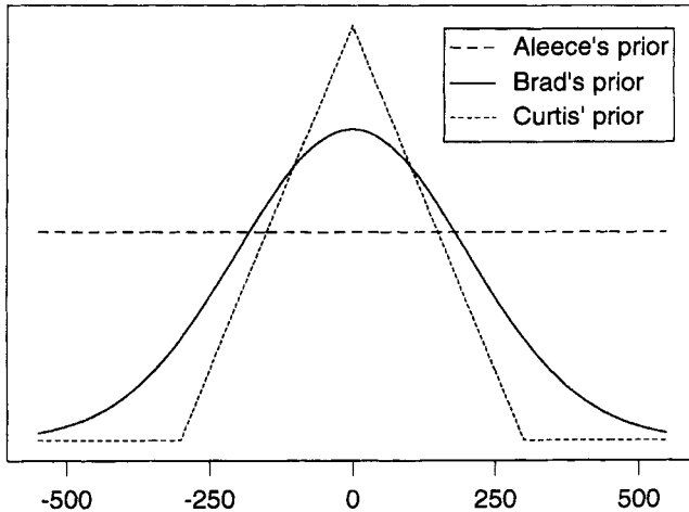
Figure 13.1 The shapes of Aleece's, Brad's, and Curtis' prior distributions.
