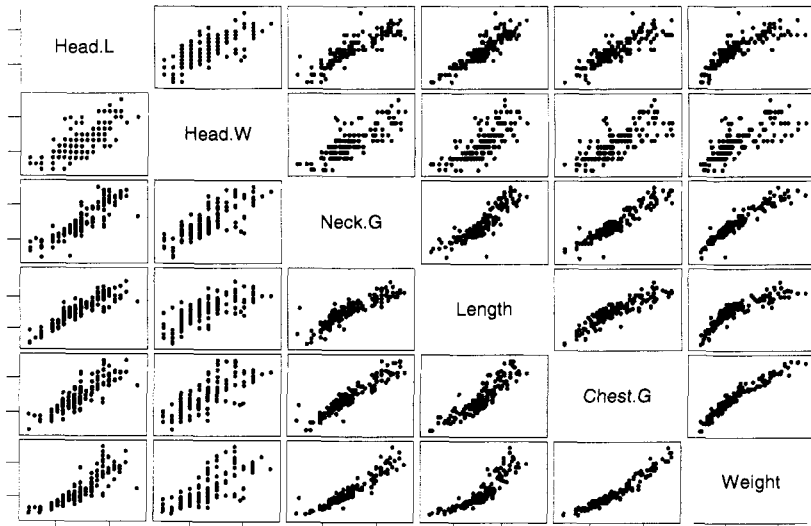
Figure 3.12 Scatterplot matrix of bear data.
