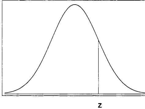
Figure B.3 Ordinates of standard normal density function. These values are shown in Table B.3.
