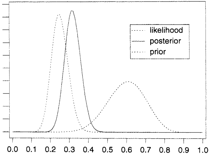
Figure 16.1 Archie's prior, likelihood, and posterior.
