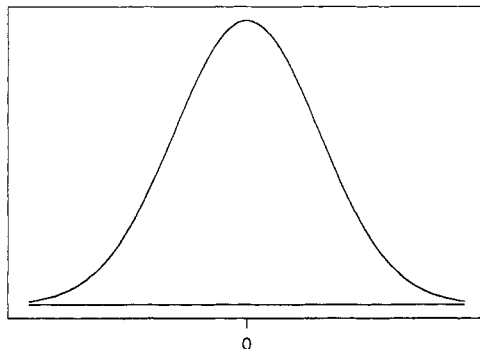
Figure B.1 Standard normal density.
