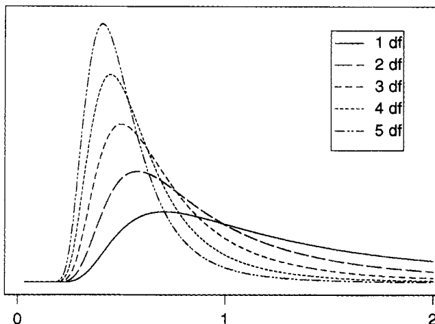
Figure 15.2 Prior for standard deviation \sigma corresponding to inverse chi square prior for variance \sigma^2 where S = 1 .
