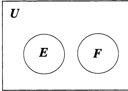
Figure 4.5 Event E and event F are mutually exclusive or disjoint events.
