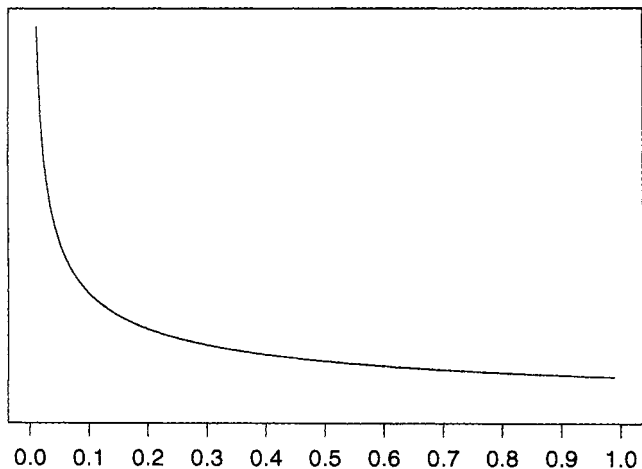
Figure A.9 The function f(x) = x^{-1/2} .
