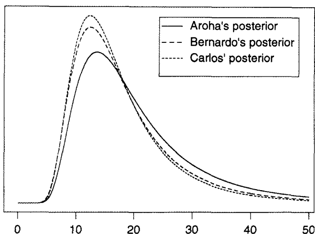
Figure 15.6 Aroha's, Bernardo's, and Carlos' posterior distributions for variance \sigma^2 .
