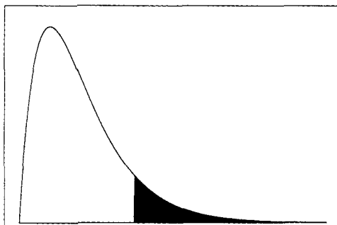
Figure B.5 Upper tail area of chi-squared distribution.
