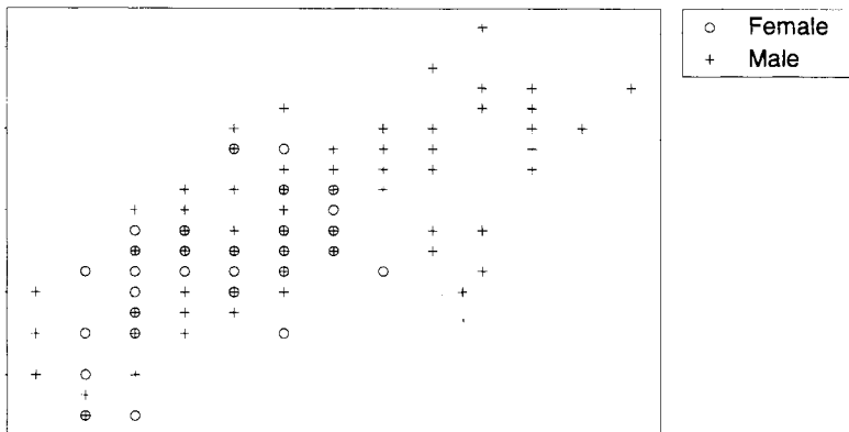
Figure 3.11 Head length versus head width in black bears.
