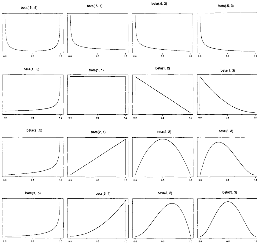
Figure 8.1 Some beta distributions.
