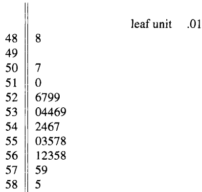
Figure 3.3 Stem-and-leaf plot for Cavendish's Earth density measurements.
