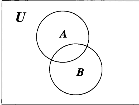
Figure 4.6 Two events A and B in the universe U .
