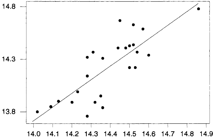
Figure 14.2 Scatterplot and least squares line for the moisture data.
