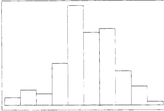
Figure 7.3 Density histogram after 100 draws.
