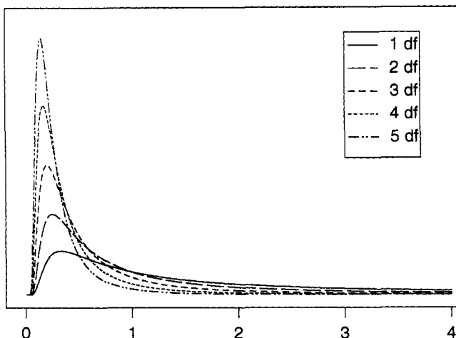
Figure 15.1 Inverse chi-squared distribution with for 1, . . . , 5 degrees of freedom. As the degrees of freedom increase, the probability gets more concentrated at smaller values. Note: S = 1 for all these graphs.
