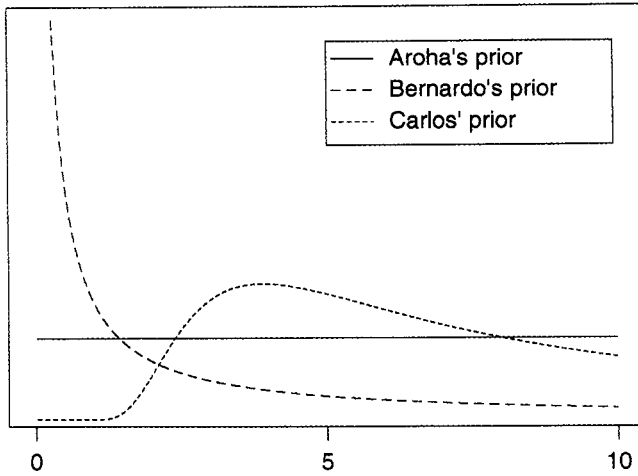
Figure 15.5 the shapes of Aroha's, Bernardo's, and Carlos' prior distributions for the standard deviation \sigma .
