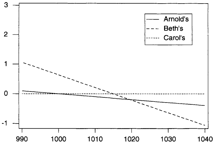
Figure 12.1 Biases of Arnold's, Beth's, and Carol's estimators.
