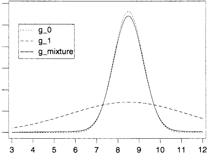
Figure 16.6 Caitlin's mixture prior and its components.
