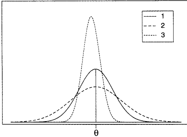
Figure 9.1 Sampling distributions of three estimators.
