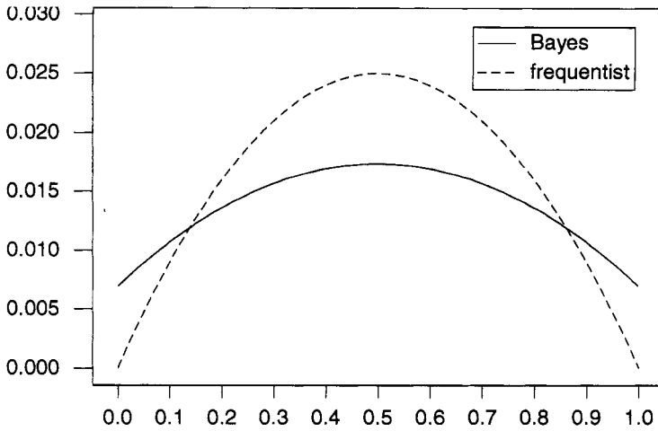
Figure 9.2 Mean squared error for the two estimators.
