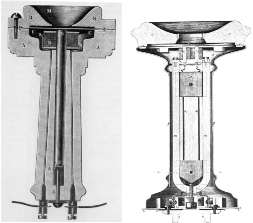
Figure 10.9 Cross sections of the Bell (left) and Siemens (right) telephones in 1878. (Scanned from Archiv für deutsche Postgeschichte , Vol. 1, 1986, pp. 37, 39.)
