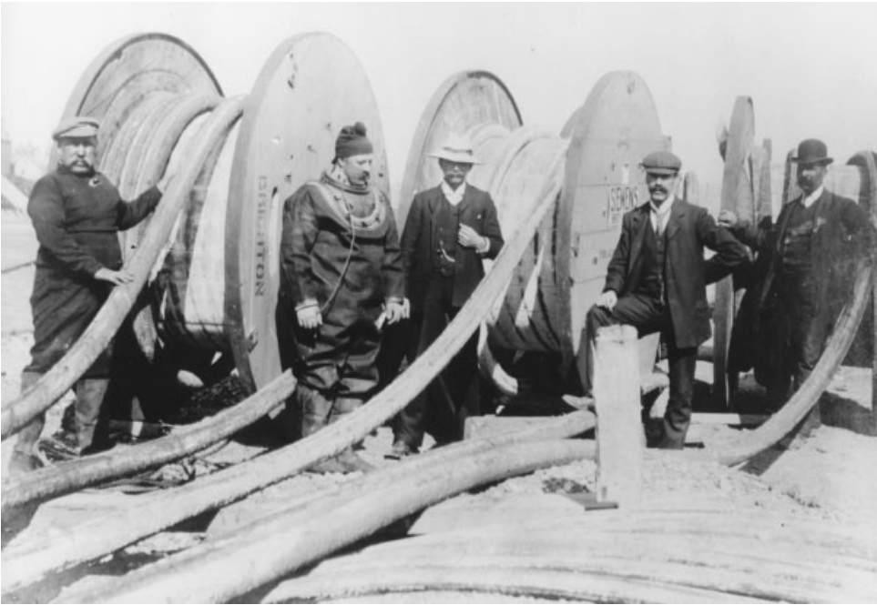
Figure 8.22 Transatlantic cable at the factory. (Courtesy of Siemens Press Photo.)
