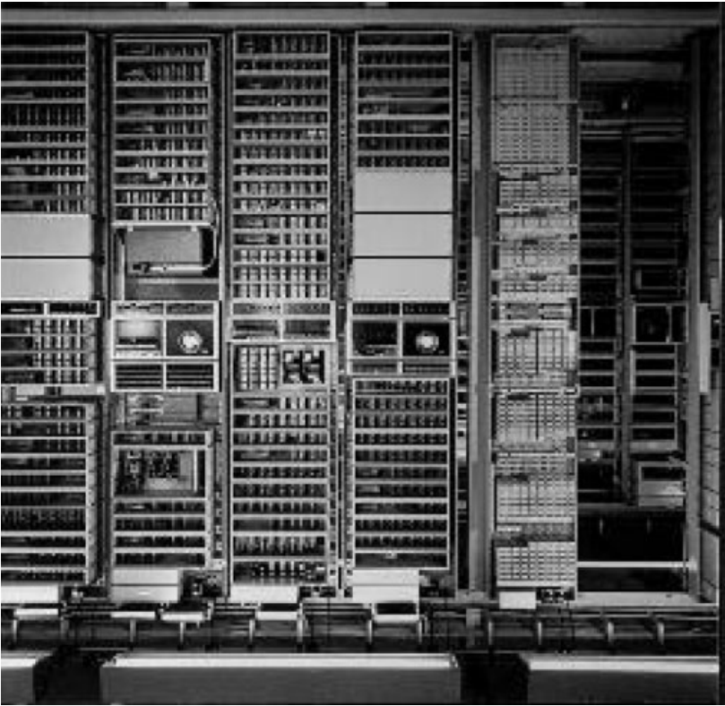
Figure 29.4 Electronic switch, type EWS, 1970. (Courtesy of Alcatel SEL.)
