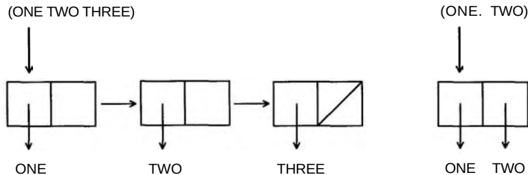
Figure 3.1: Cons Cell Diagrams
