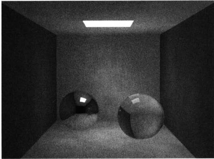
Figure 8.5. A fast simulation of the box scene. This example was rendered faster than just using ray tracing. The trick is to use only 200 photons in the photon map and 50 in the radiance estimate. A consequence of this simple approximation is that the illumination is very blurry (even the shadows are missing).
