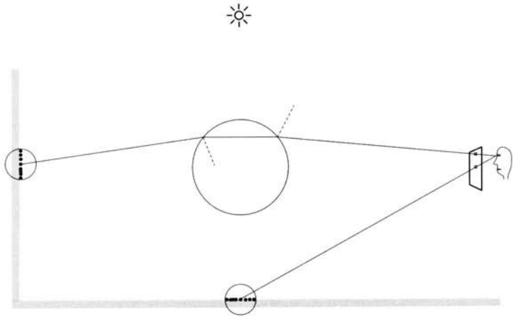
Figure 8.1. The photon map can be visualized directly using a simple ray tracer. For all diffuse surfaces the ray tracer uses the radiance estimate from the photon map, whereas standard recursive ray tracing is used for specular surfaces.
