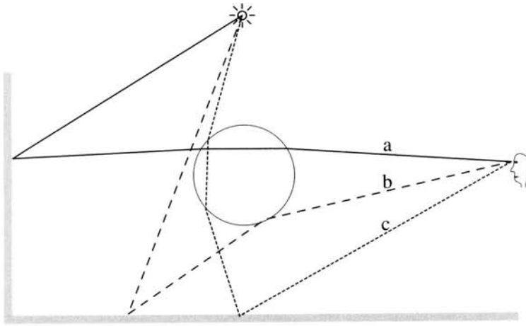
Figure 2.7. The light transport notation makes it easy to classify different paths. In this scene, with a glass ball and two diffuse walls, the paths shown are: (a) LDSSE, (b) LDSE, and (c) LSSDE.
