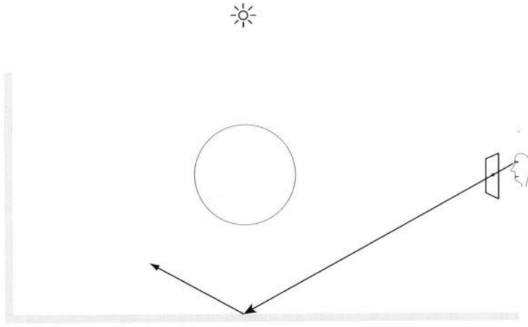
Figure 9.5. Specular and glossy reflections or transmissions are evaluated using recursive ray tracing. Ray tracing is good at integrating the contribution from the narrow peak in the BRDF. For glossy reflections it is possible to use a photon map, but this would require a large number of photons to get an accurate directional estimate.
