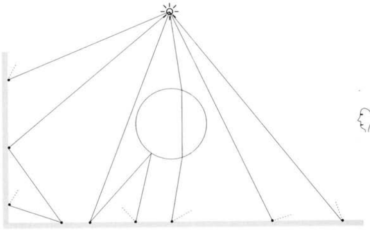
Figure 9.2. The global photon map is created by tracing photons towards all objects in the model. During photon tracing all surfaces can reflect and transmit photons. All photons that hit a diffuse surface are stored in the global photon map.
