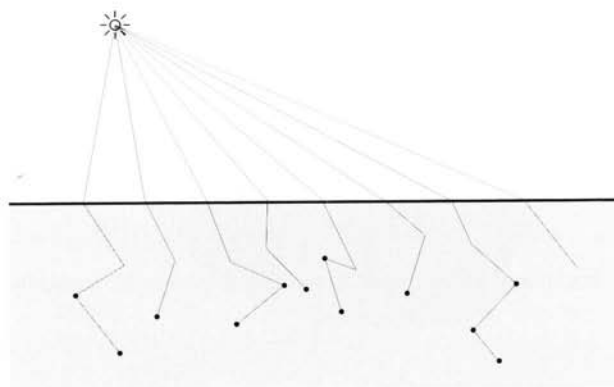
Figure 10.8. Photon tracing for subsurface scattering.
