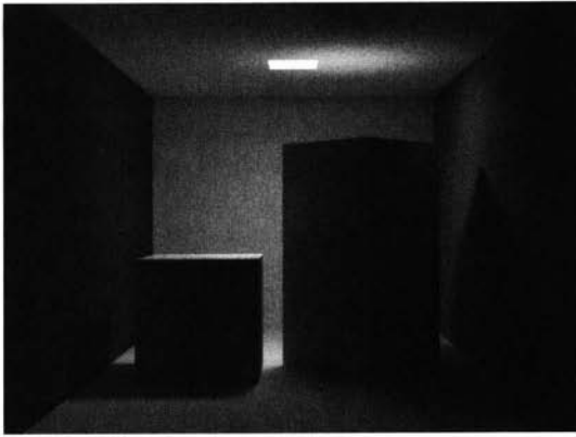
Figure 1.4. A typical radiosity scene. This is a replica of the widely used Cornellbox which is a box scene with two cubes and a square light source at the top. Radiosity is good at handling diffuse reflection and polygonal surfaces. (See Color Plate II.)
