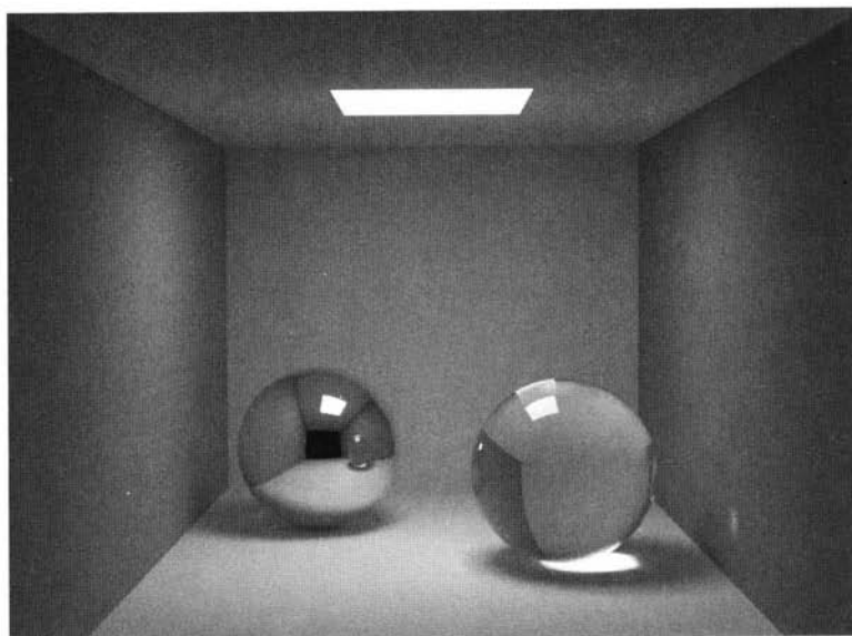
Figure 9.9. The box scene with full global illumination. (See Color Plate VI)
