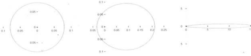
Figure 10.1. The Henyey-Greenstein phase function with different g . From left to right g = 0.0 , g = 0.3 , and g = 0.9 .
