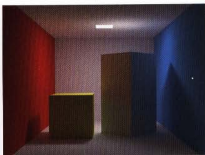
Plate II. Finite element radiosity algorithms are good at simulating diffuse interreflection as seen in this replica of the widely used Cornellbox. (See Figure 1.4)
