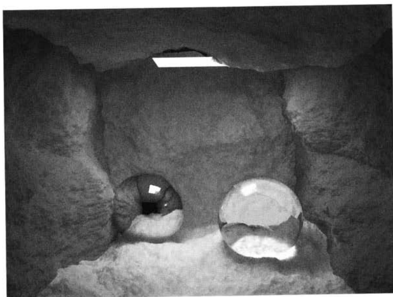
Figure 9.13. Fractal box.
