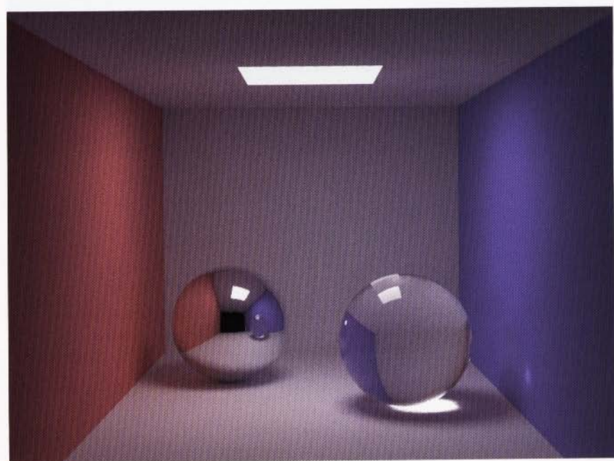
Plate VII. The box scene with full global illumination. (See Figure 9.9)
