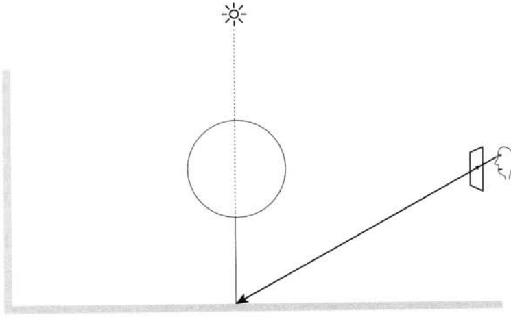
Figure 9.4. Direct illumination is evaluated accurately using ray tracing. A shadow ray is traced between the light source and the point of interest to determine if the point is illuminated or in shadow.
