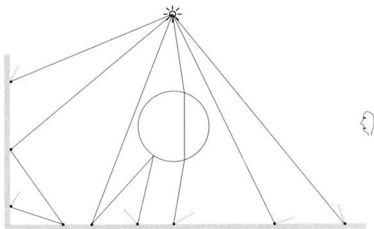
Figure 5.1. The photon map is built using photon tracing in which photons are emitted from the light sources and stored as they interact with the diffuse surfaces in the model.
