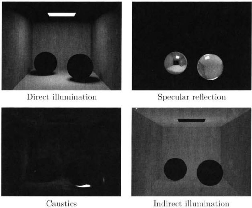
Figure 9.8. The different components of the rendered solution.
