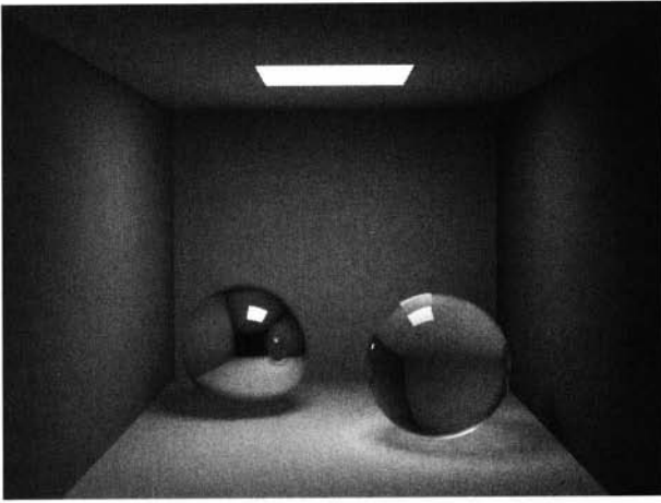
Figure 8.4. A simulation of global illumination in the box using 10,000 photons in the photon map and 500 photons in the radiance estimate. For this image we used only the photon map to compute the indirect illumination. The direct lighting is computed using standard ray-tracing techniques. Even though the indirect lighting is blurry (in particular the caustic below the glass sphere) the overall quality of the illumination is reasonable.
