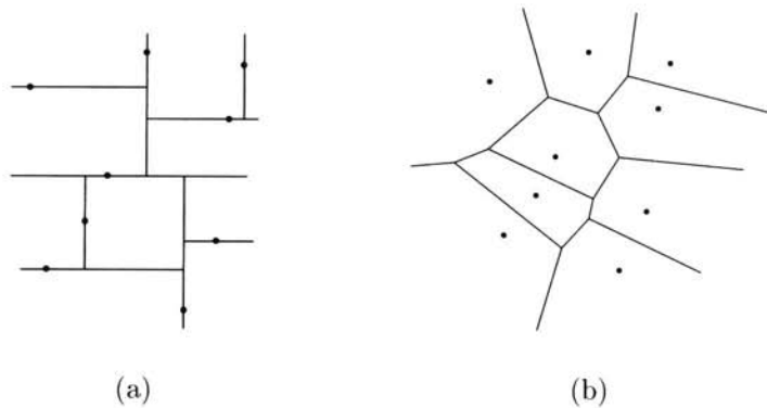
Figure 6.1. A two-dimensional point set classified using (a) a kd-tree and (b) a Voronoi diagram.
