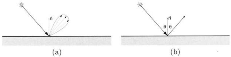
Figure 2.5. A specular surface reflects the incoming light in the mirror direction. (a) shows glossy specular reflection (i.e., a rough mirror surface), and (b) shows perfect specular reflection (a mirror surface).
