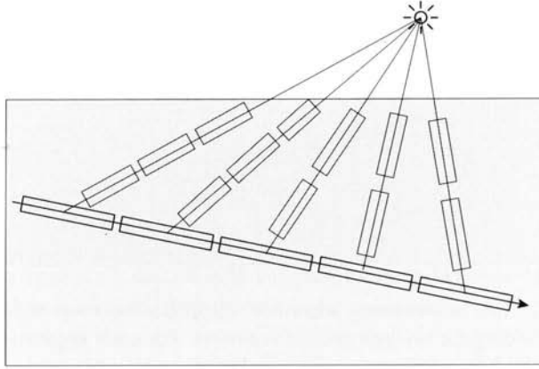
Figure 10.3. The contribution from the light source must be attenuated based on the medium along the shadow ray. In non-homogeneous media this requires a ray-marching integration for each shadow ray.
