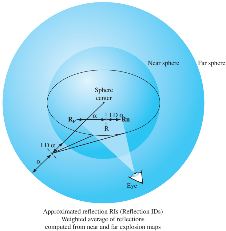
Figure 17.12 Combining the results of near and far explosion map evaluation.
